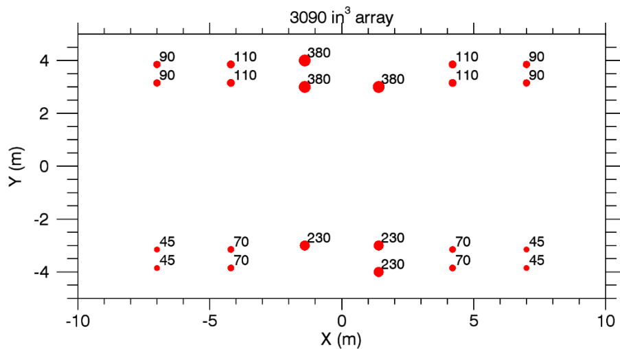
Figure A-1. Layout of the modelled 3090 in 3 array. Tow depth is 6 m. The labels indicate the firing volume (in cubic inches) for each airgun. Also see Table A-1.
