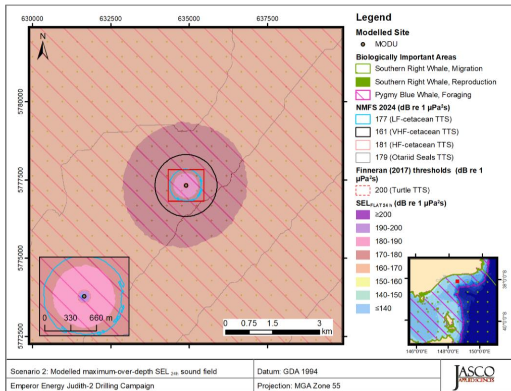
Figure 15. Scenario 2: MODU Drilling : Sound level contour map showing maximum-over-depth SEL 24h results (unweighted/flat), along with frequency weighted isopleths for TTS in low, high, very high-frequency cetaceans, otariid seals and turtles. Thresholds omitted here were not reached or not long enough to display graphically.
