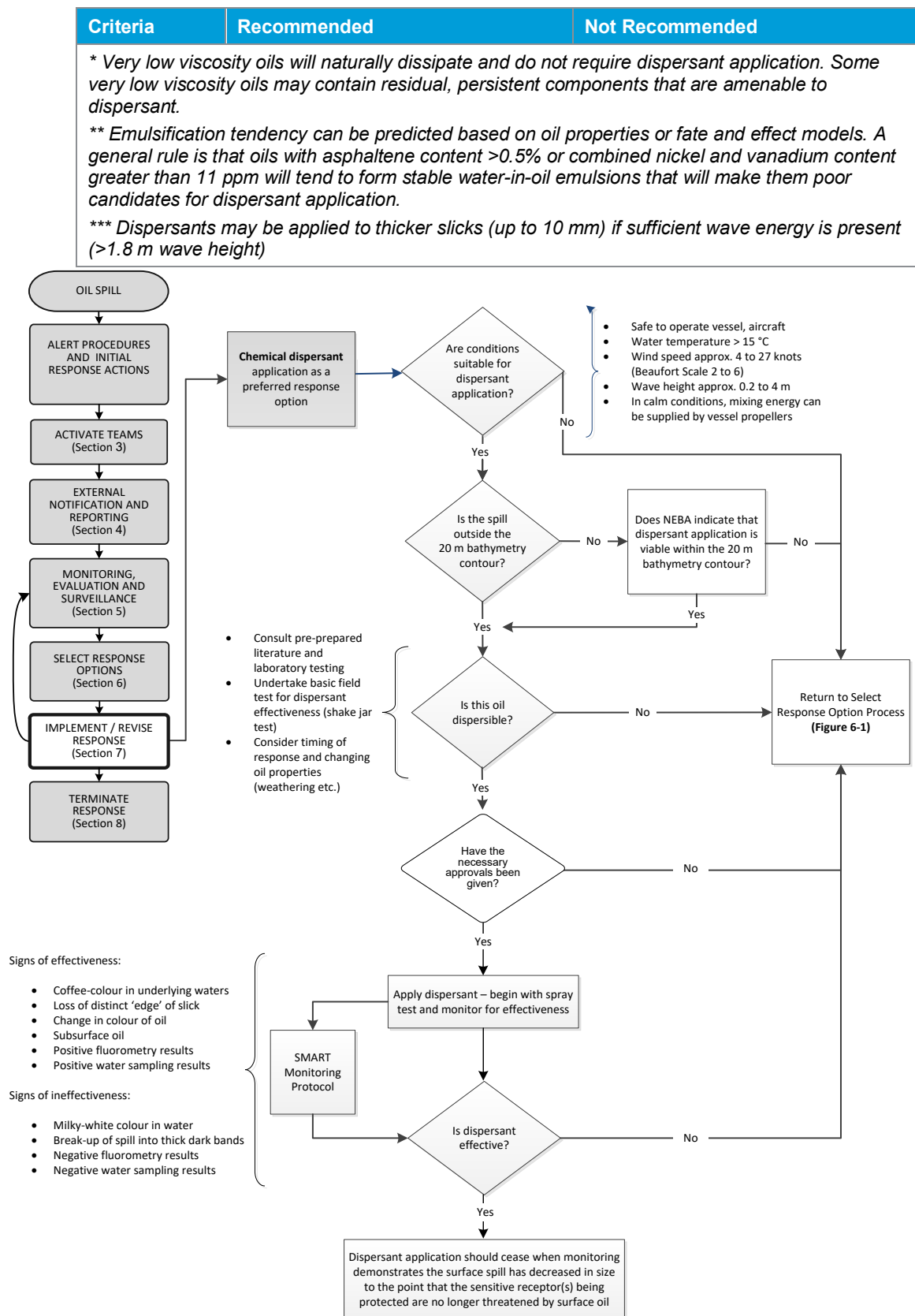
Figure 7-4: Surface Dispersant Operations Decision Guide
