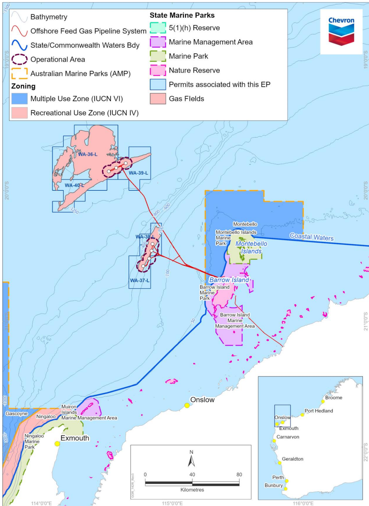
Figure 2-1: Overview of Gorgon and Jansz infrastructure 1
