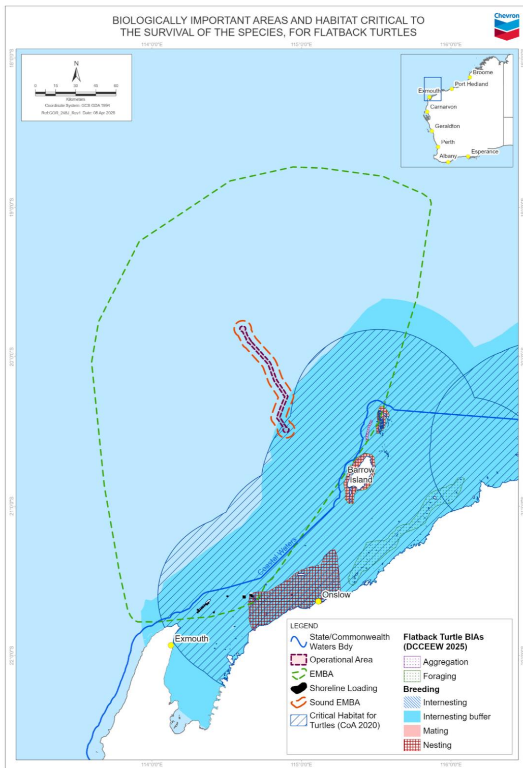
Figure 4-8: Flatback BIAs and HCTS of the species
