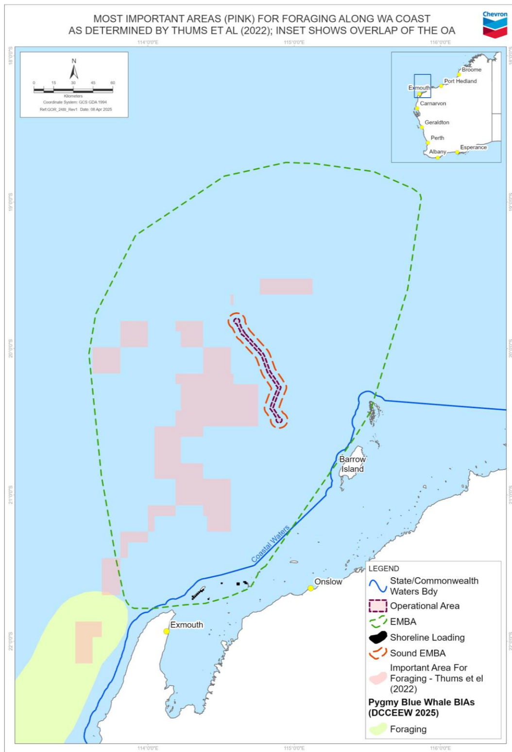
Figure 4-7: Most important areas (pink) for foraging along WA coast as determined by Thums et al. (2022)
