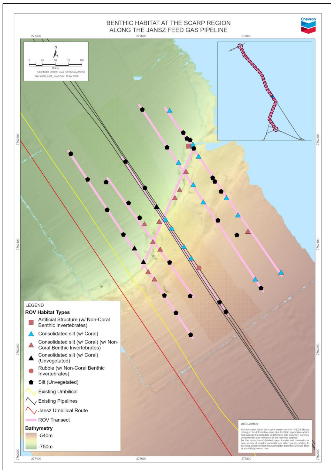
Figure 4-4: Benthic habitat at the scarp region along the Jansz feed gas pipeline
