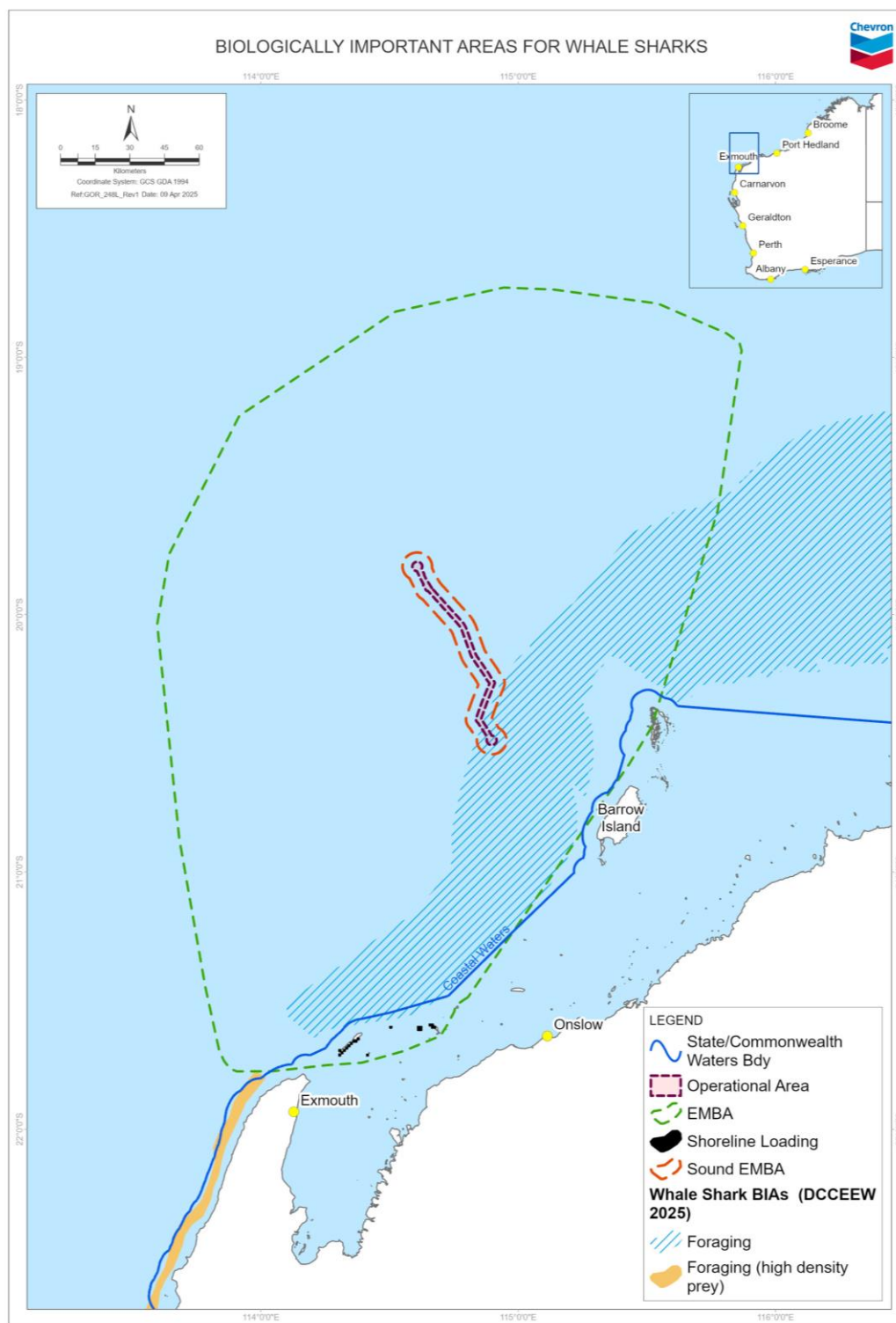
Figure 4-9: Biologically important areas for Whale Sharks
