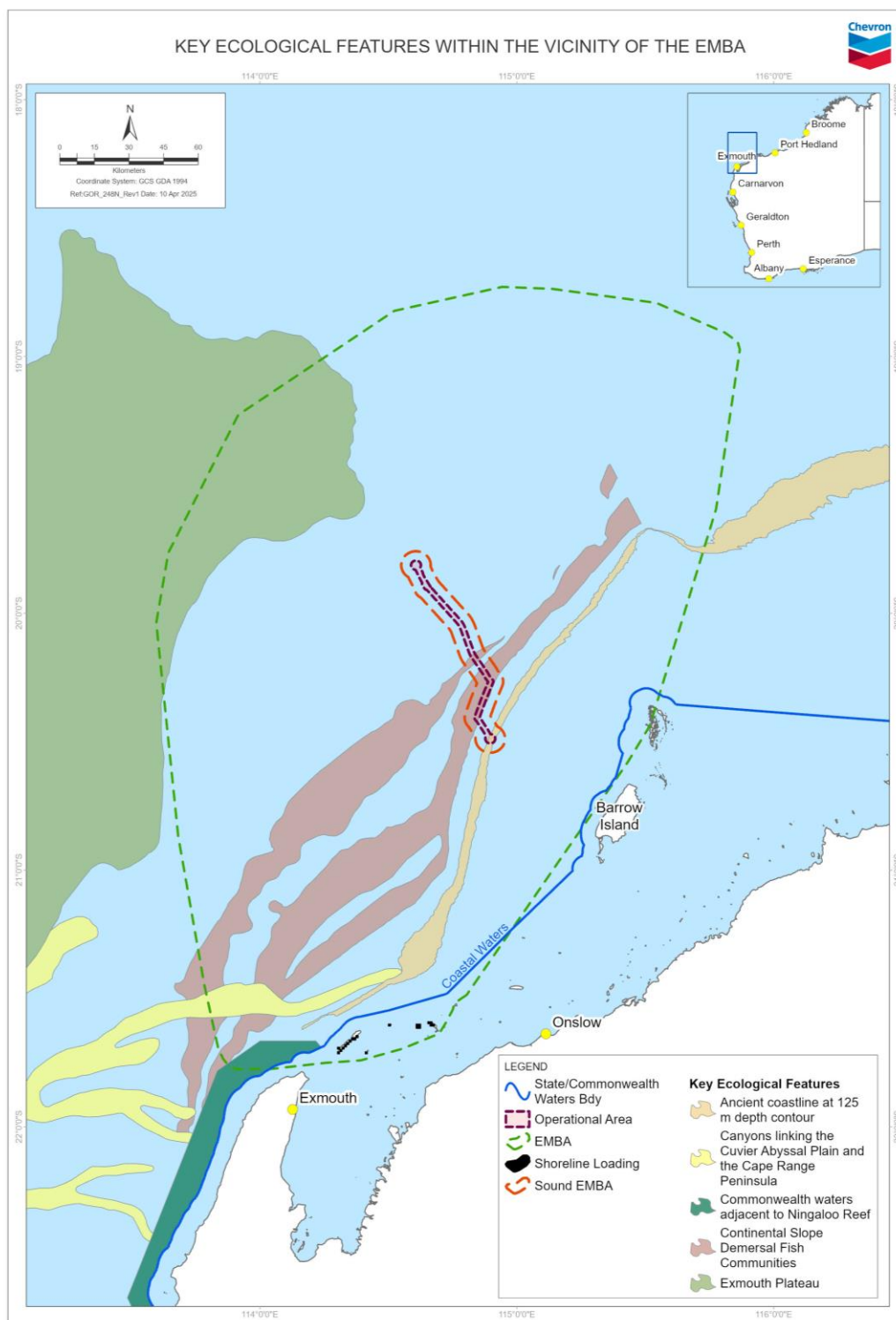
Figure 4-11: Key ecological features within the vicinity of the EMBA
