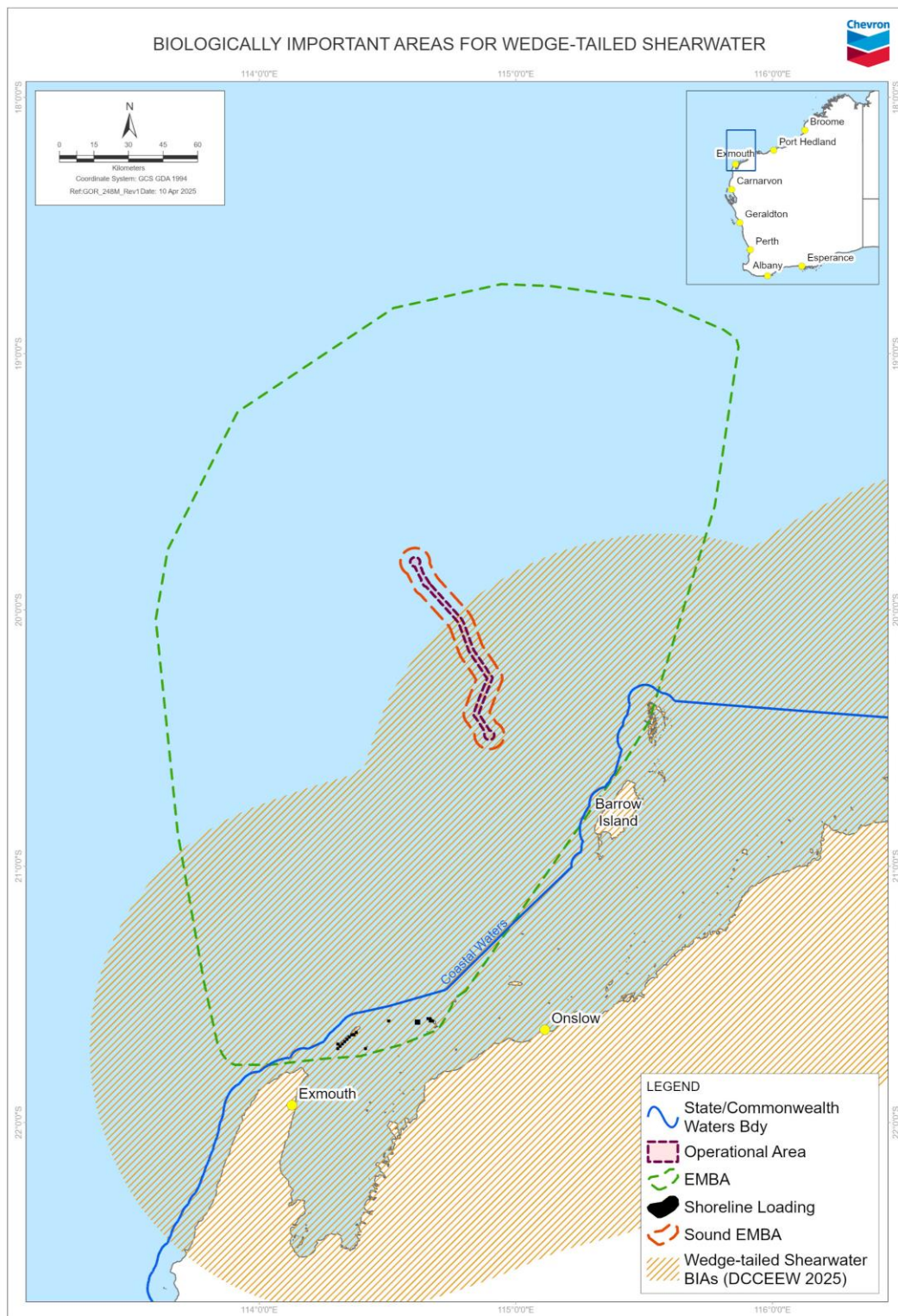
Figure 4-10: Biologically important areas for Wedge-tailed Shearwater
