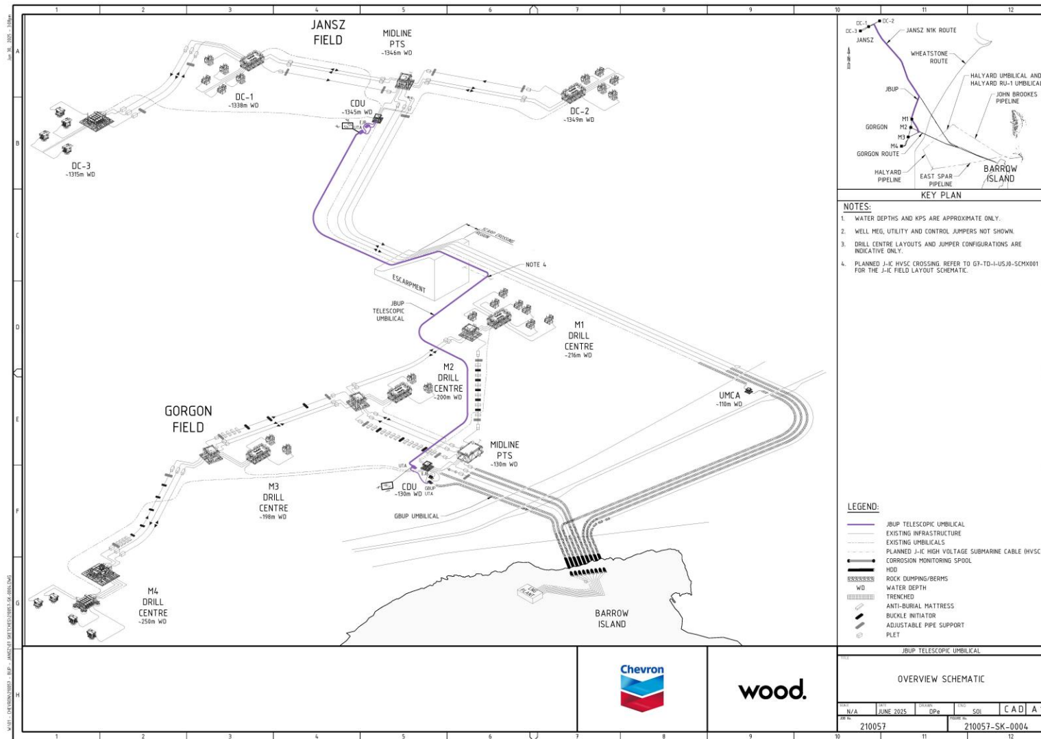
Figure 3-2: Schematic of existing infrastructure layout
