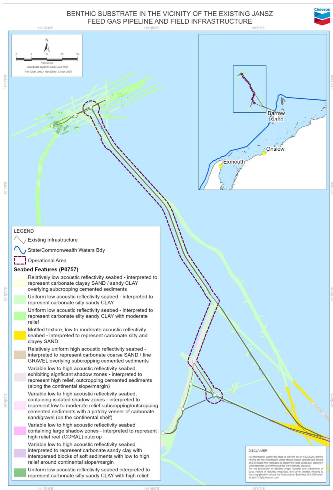
Figure 4-2: Benthic substrate in the vicinity of the existing Jansz feed gas pipeline and field infrastructure
