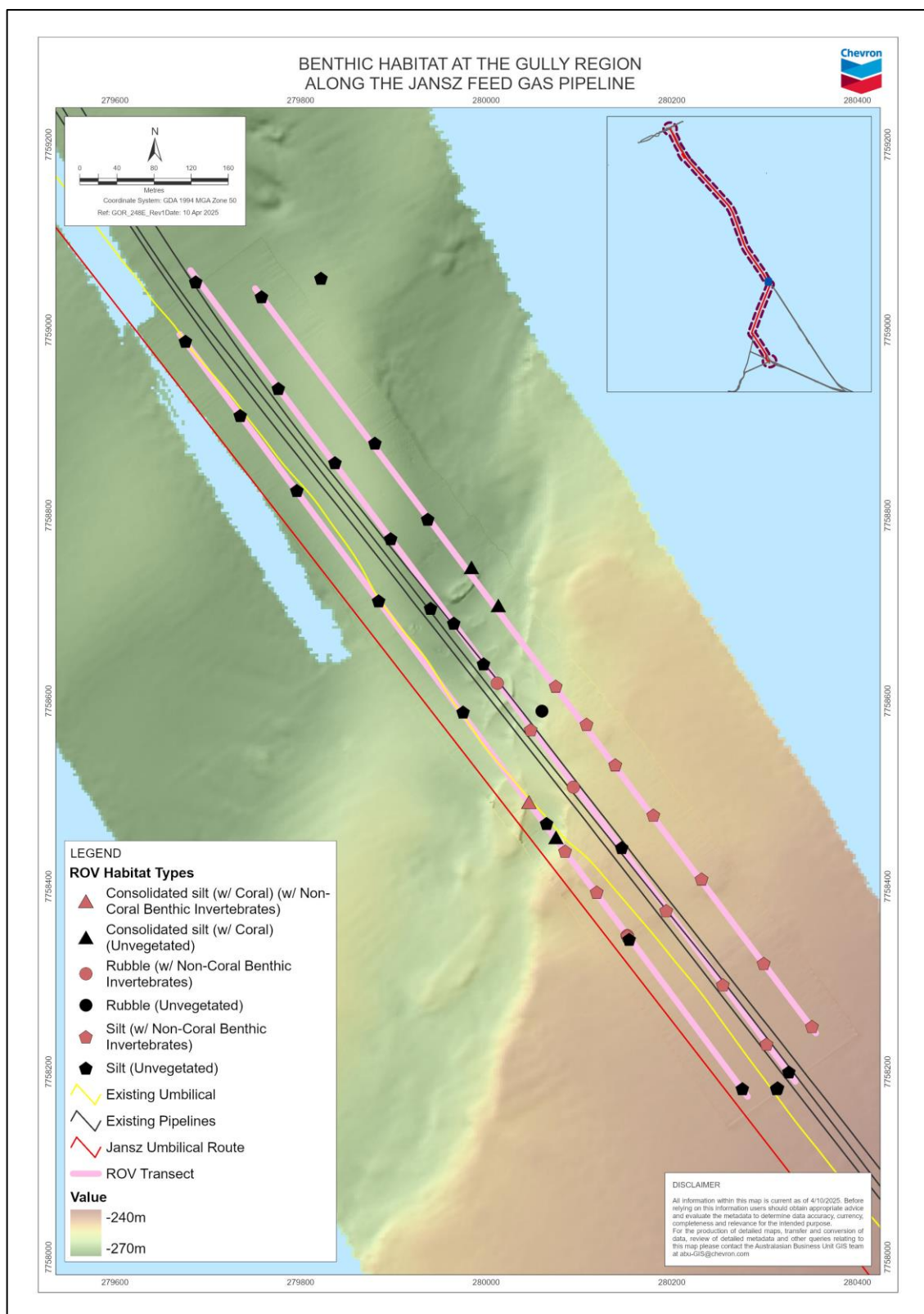
Figure 4-3: Benthic habitat at the gully region along the Jansz feed gas pipeline
