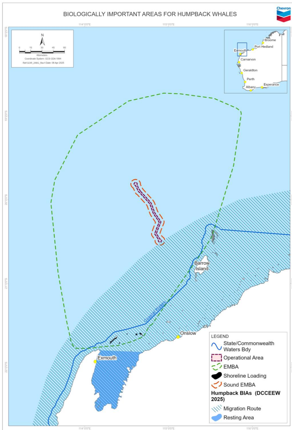
Figure 4-5: Biologically important areas for Humpback Whales
