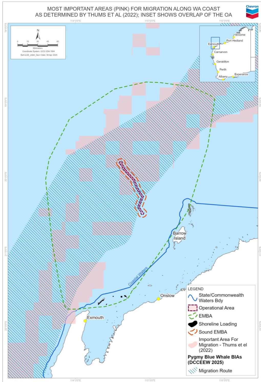
Figure 4-6: Most important areas (pink) for migration along WA coast as determined by Thums et al. (2022)
