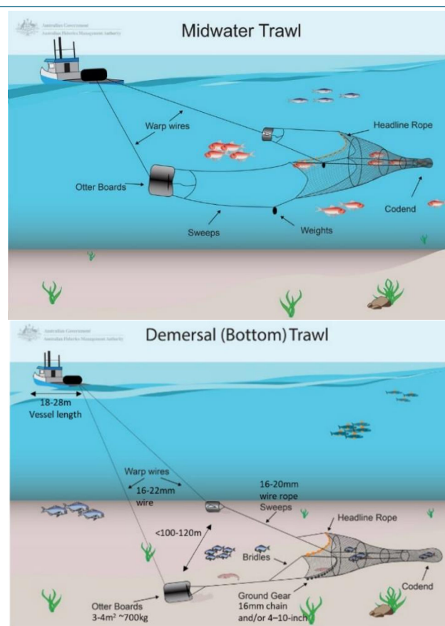
Figure 40. Demersal and midwater otter board trawl diagrams
