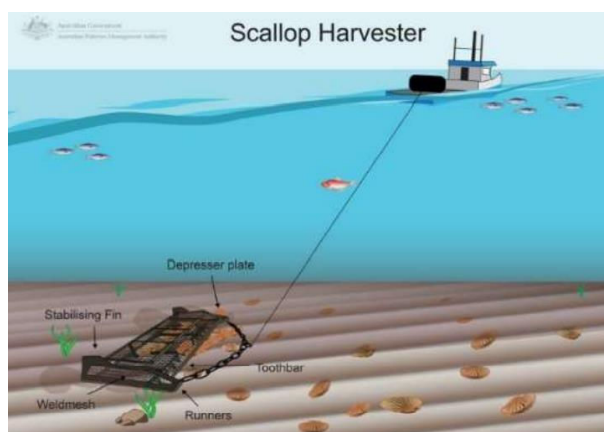
Figure 49. Diagram of scallop harvester
