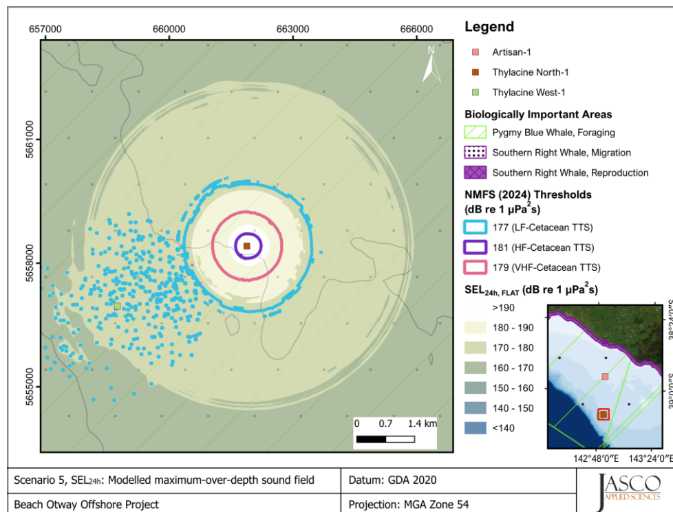
Figure 8. Scenario 5, MODU Drilling + 4h AHTS resupply at Thylacine North-1 + AHTS Standby at Thylacine West -1, accumulated SEL 24h : Sound level contour map showing maximum-over-depth SEL 24h results (unweighted/flat), along with frequency weighted isopleths for TTS in low, high, and very high-frequency cetaceans.
