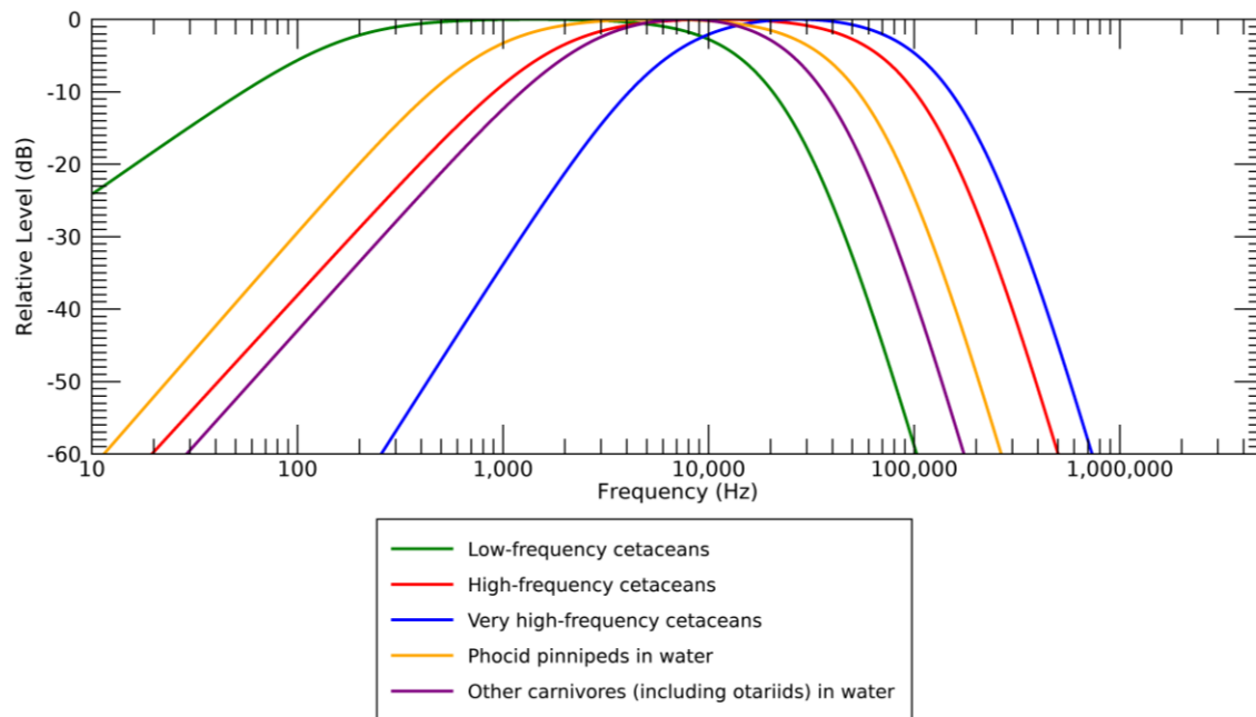
Figure A-1. Auditory weighting functions for functional marine mammal hearing groups used in this project as recommended by NMFS (2024).
