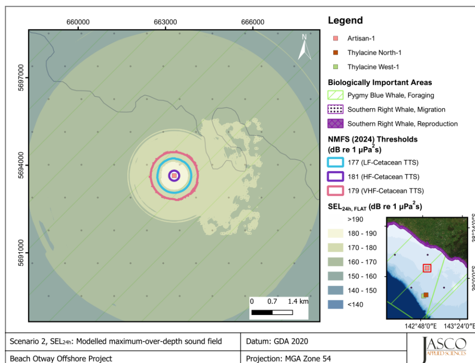
Figure 5. Scenario 2, MODU Drilling + OSV Standby Transit at Artisan-1, accumulated SEL 24h : Sound level contour map showing maximum-over-depth SEL 24h results (unweighted/flat), along with frequency weighted isopleths for TTS in low, high, and very high-frequency cetaceans.
