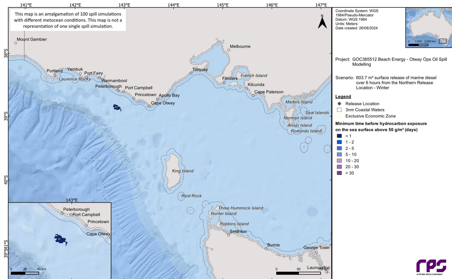
Figure 14-9 Minimum time before floating oil exposure above 50 g/m 2 , in the event of 603.7 m 3 surface release of marine diesel for a loss of containment from vessel collision at Northern Release Location. The results were calculated from 100 spill simulations during winter conditions.
