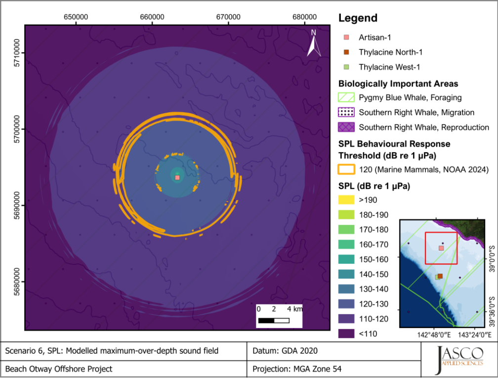
Figure 3. Scenario 6, MODU on DP + 1x OSV on DP + 2x OSV within 2km of location (hooking up anchors) at Artisan-1, SPL: Sound level contour map showing the unweighted maximum-over-depth sound field in 10 dB steps, and the isopleth for behavioural response threshold for marine mammals.
