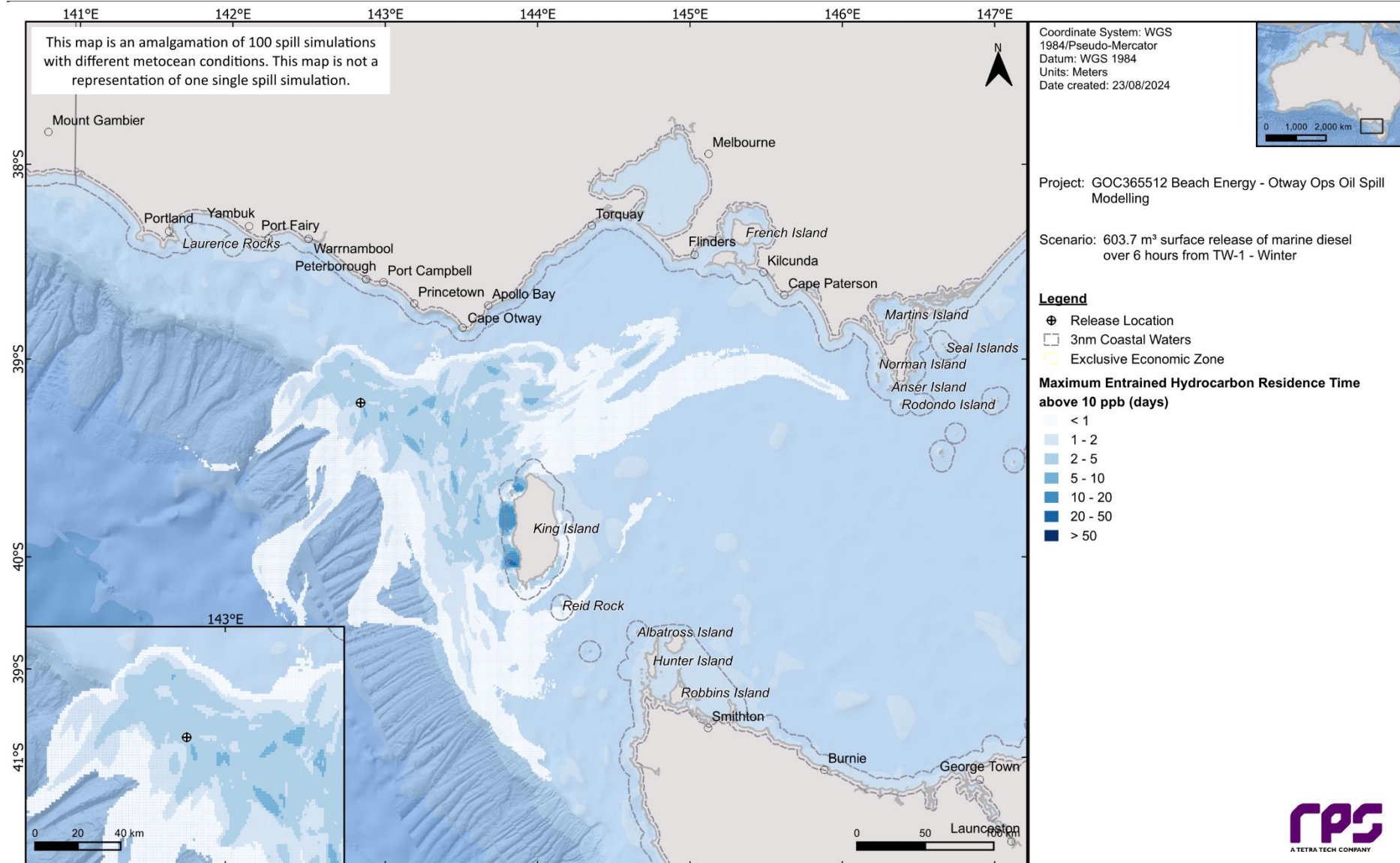
Figure 16-20 Maximum residence time for entrained hydrocarbon exposure above 10 ppb, at 0-10 m below the sea surface in the event of a 603.7 m 3 surface release of marine diesel for a loss of containment from vessel collision at TW1. The results were calculated from 100 spill simulations during winter conditions.
