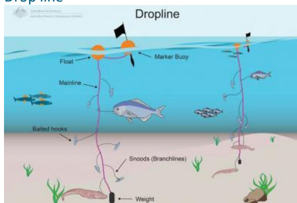
Figure 47. Diagram of dropline arrangement
