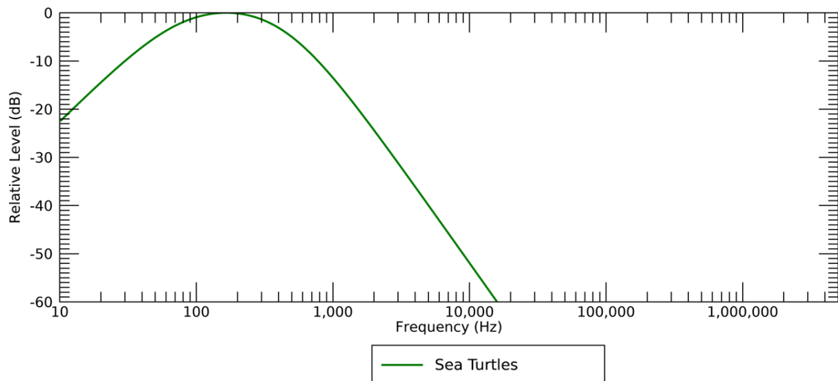
Figure A-2. Auditory weighting functions for sea turtles used in this project as recommended by Accomando et al. (2025).
