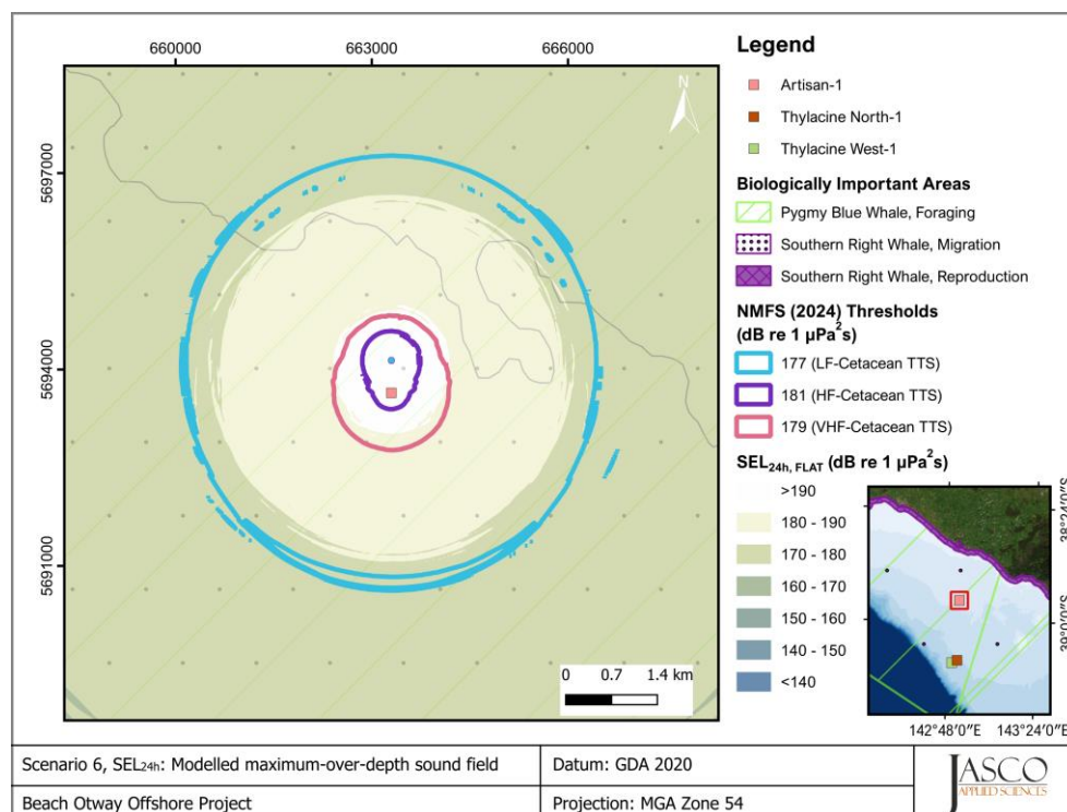
Figure 9. Scenario 6, MODU on DP + 1x OSV on DP + 2x OSV within 2km of location (hooking up anchors) at Artisan-1, accumulated SEL 24h : Sound level contour map showing maximum-over-depth SEL 24h results (unweighted/flat), along with weighted isopleths for TTS in low, high, and very high-frequency cetaceans.
