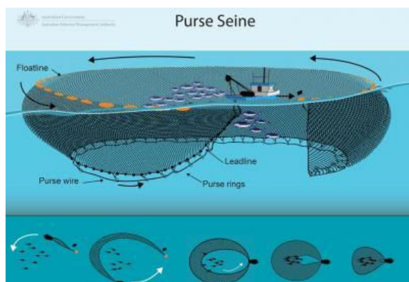
Figure 42. Diagram of purse seine fishing method
