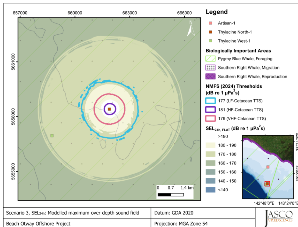
Figure 6. Scenario 3, MODU Drilling + 4h OSV resupply at Thylacine North-1, accumulated SEL_{24h} : Sound level contour map showing maximum-over-depth SEL_{24h} results (unweighted/flat), along with frequency weighted isopleths for TTS in low, high, and very high-frequency cetaceans.
