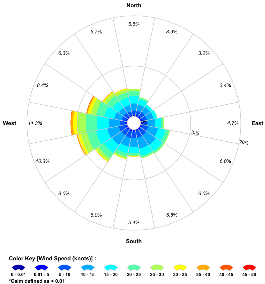
Figure 4-3 Modelled total wind rose distributions from 2010–2019 (inclusive) for the node nearby the Northern Release Location.
