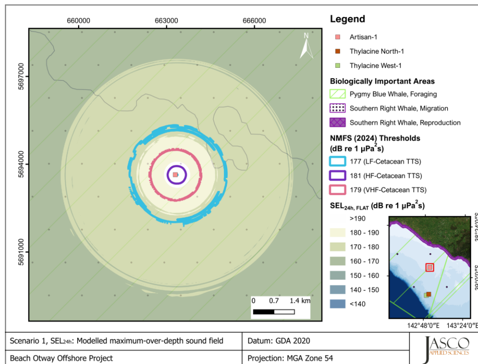
Figure 4. Scenario 1, MODU Drilling + 4h OSV resupply at Artisan-1, accumulated SEL 24h : Sound level contour map showing maximum-over-depth SEL 24h results (unweighted/flat), along with frequency weighted isopleths for TTS in low, high, and very high-frequency cetaceans.
