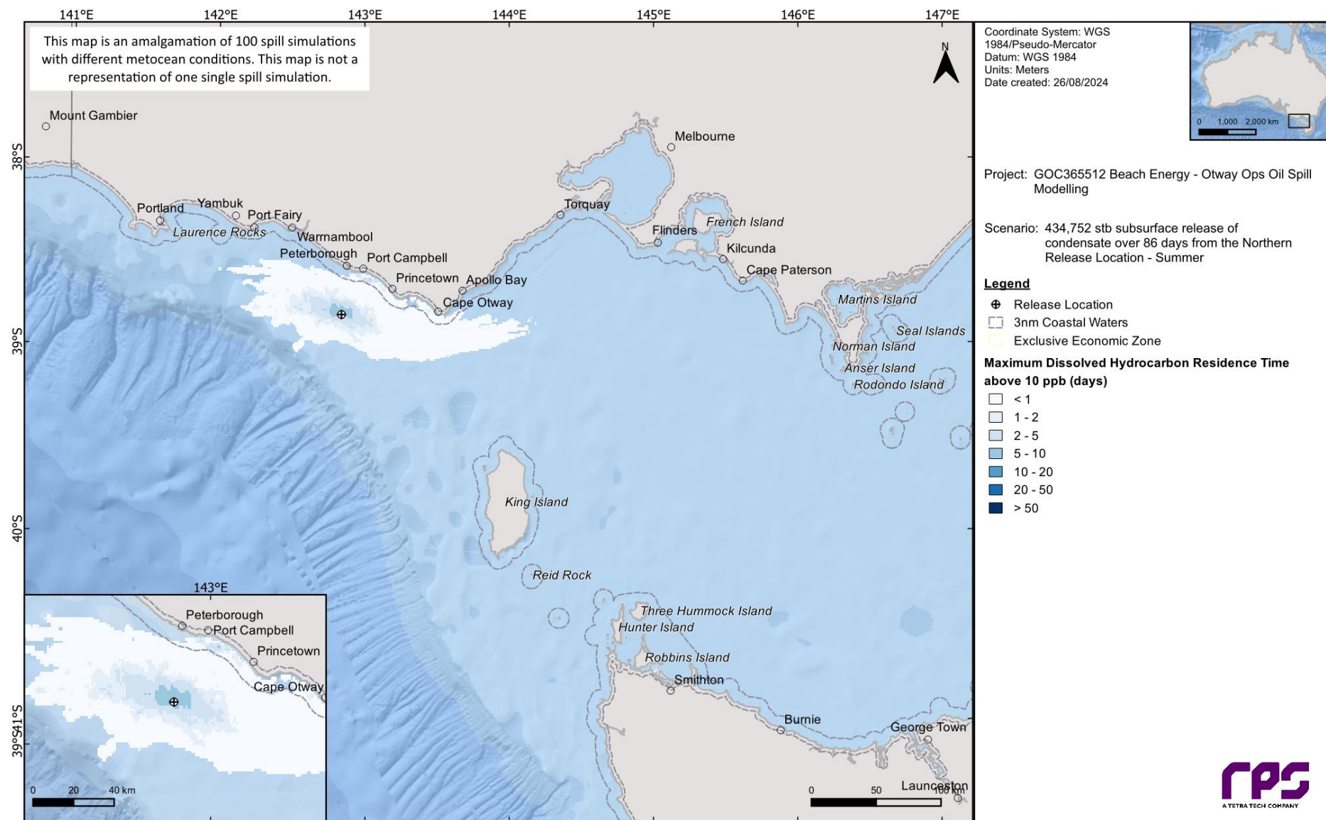
Figure 13-12 Maximum residence time for dissolved hydrocarbon exposure above 10 ppb, at 0-10 m below the sea surface in the event of a 434,752 stb subsea release of condensate over 86 days from a loss of well control at the Northern Release Location. The results were calculated from 100 spill simulations during summer conditions.
