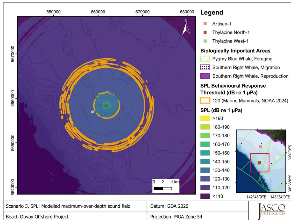
Figure 2. Scenario 5, MODU Drilling + 4h AHTS resupply at Thylacine North-1 + AHTS Standby at Thylacine West -1, SPL: Sound level contour map showing the unweighted maximum-over-depth sound field in 10 dB steps, and the isopleth for behavioural response threshold for marine mammals.
