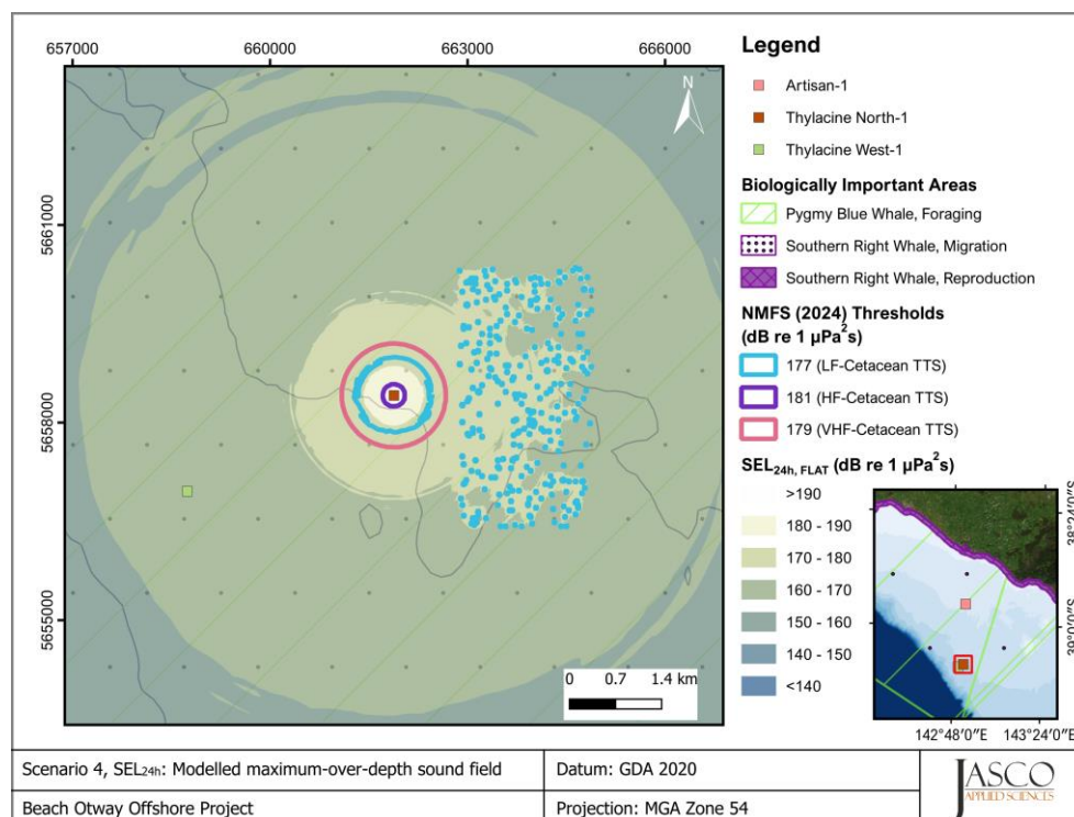
Figure 7. Scenario 4, MODU Drilling + OSV Standby Transit at Thylacine North-1, accumulated SEL_{24h} : Sound level contour map showing maximum-over-depth SEL_{24h} results (unweighted/flat), along with frequency weighted isopleths for TTS in low, high, and very high-frequency cetaceans.
