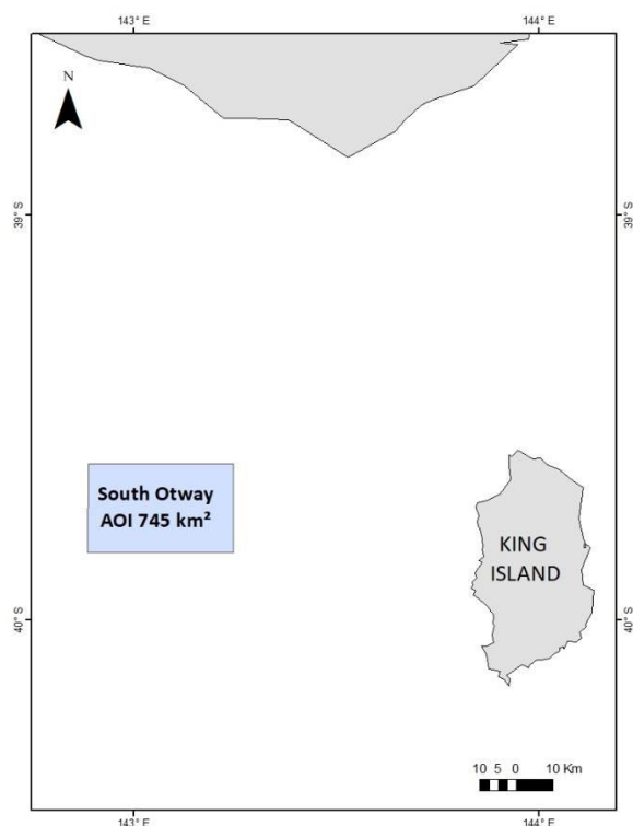
Figure 10. South Otway AOI position and size
