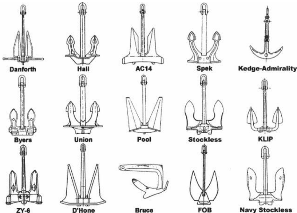
Figure 55 Types of Stockless anchor (source: www.gratitudesailingnw.com/sailing-lessons.html )
