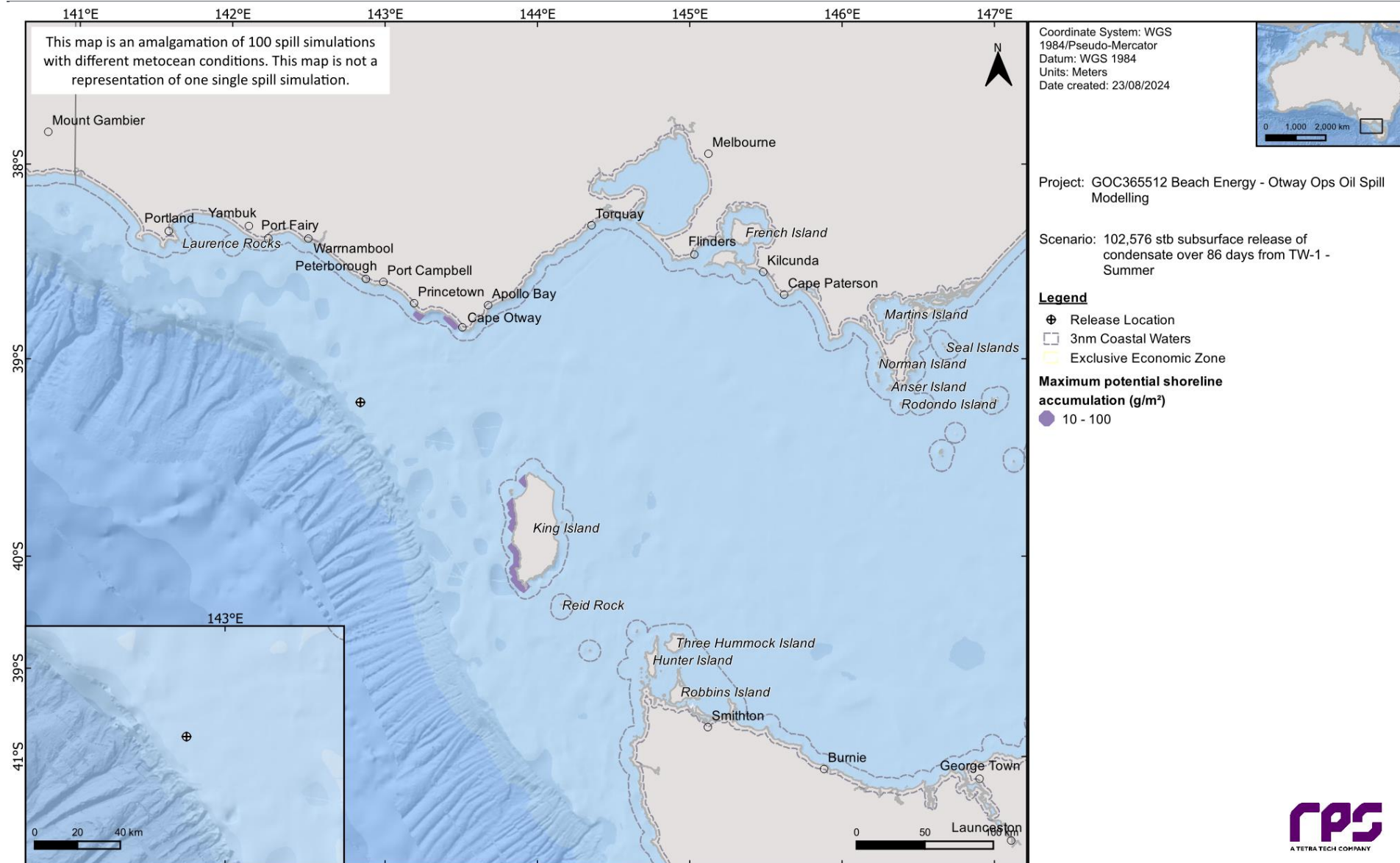
Figure 15-6 Maximum potential shoreline loading in the event of a 102,576 stb subsea release of condensate over 86 days from a loss of well control at TW1. The results were calculated from 100 spill simulations during summer conditions.
