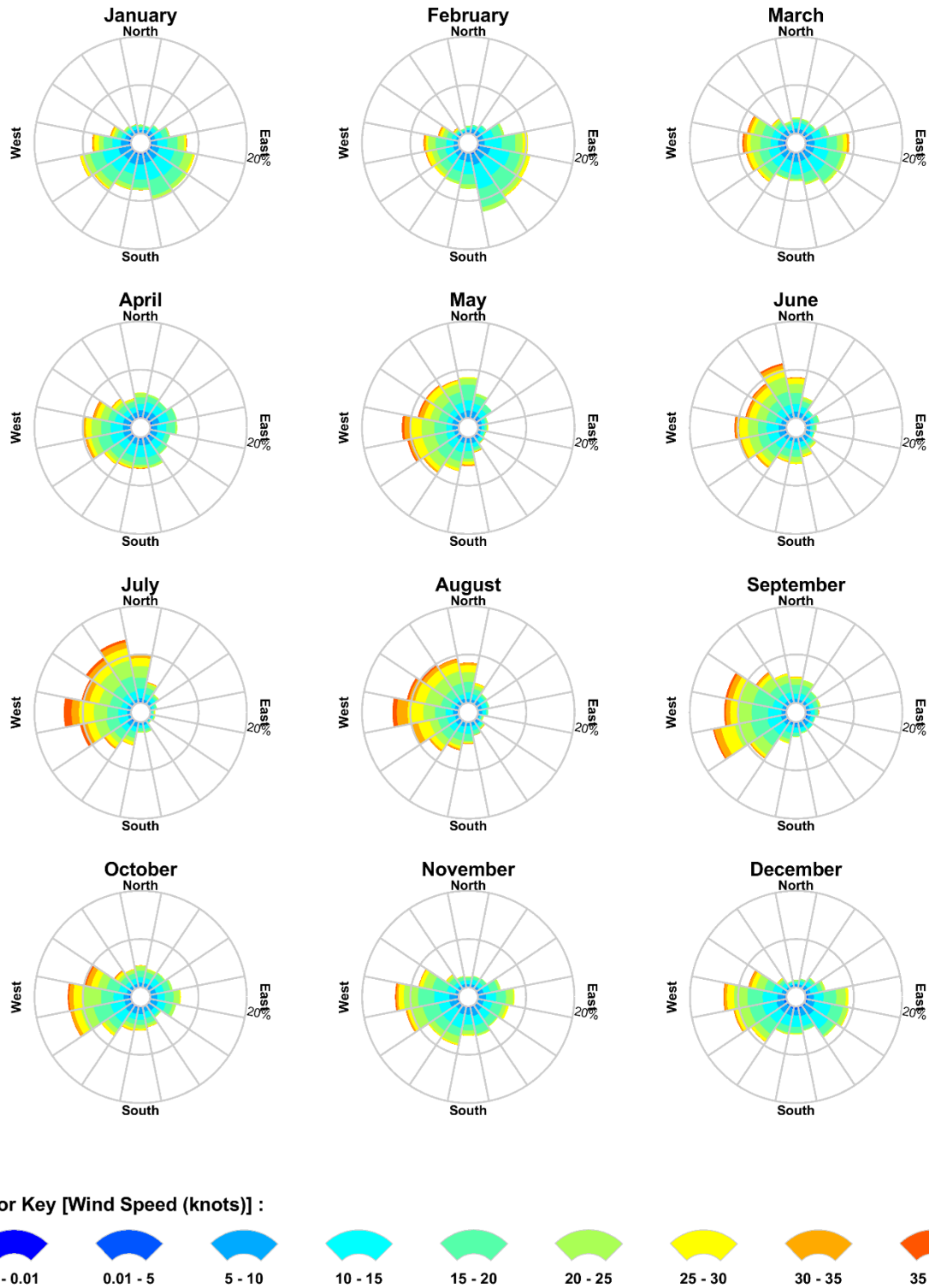
Figure 4-4 Modelled monthly wind rose distributions from 2010–2019 (inclusive) for the node nearby TW1.
