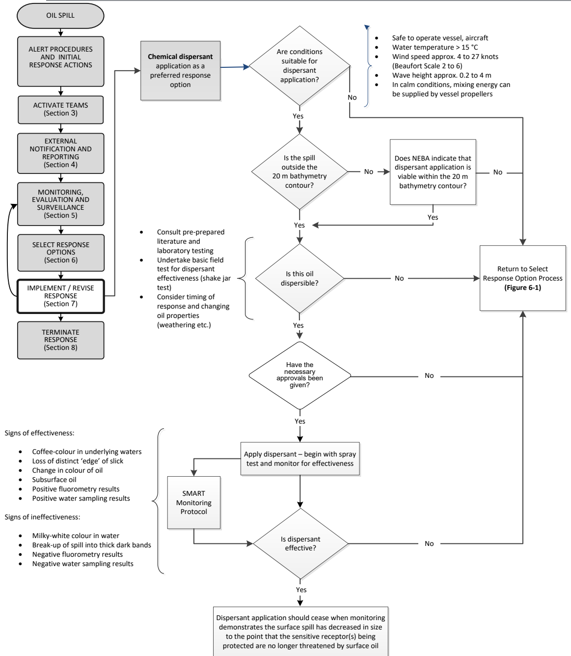
Figure 7-4: Surface Dispersant Operations Decision Guide
