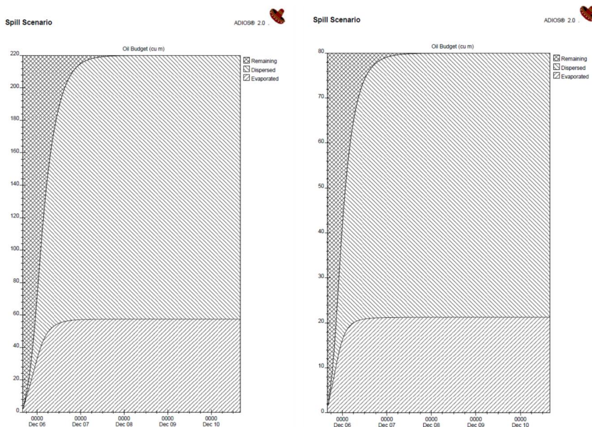
Figure 6-3 ADIOS Oil Budgets for marine diesel spills
