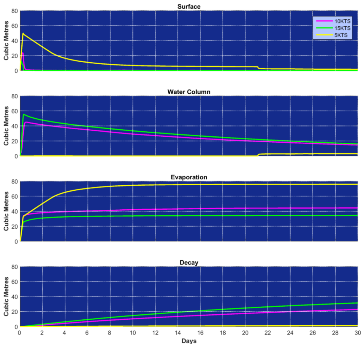
Figure 6-1 Predicted weathering and fates graph for Marine Diesel Oil
