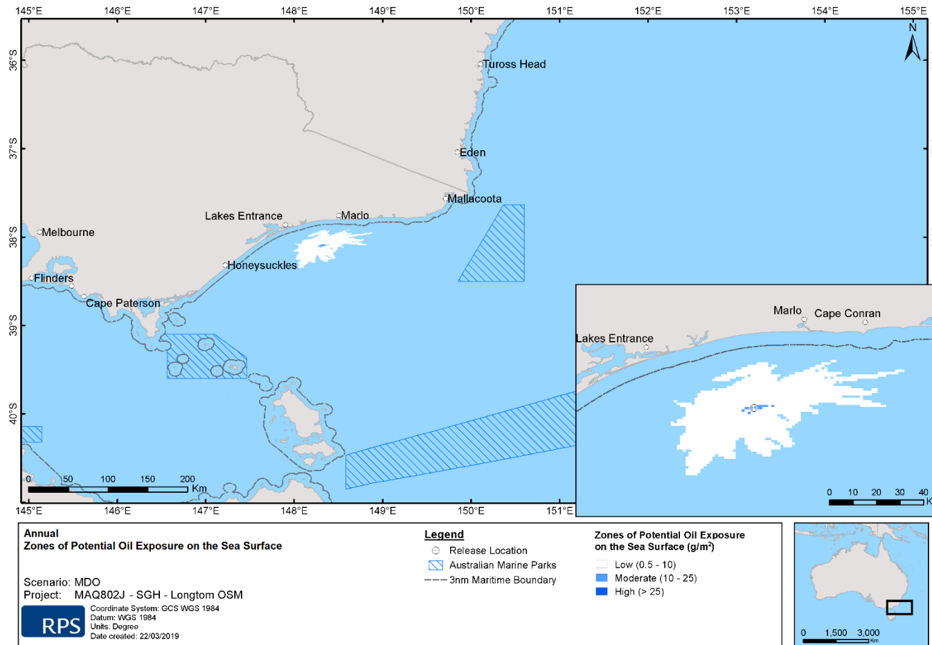
Figure 6-2 Zones of potential MDO exposure on the sea surface.
