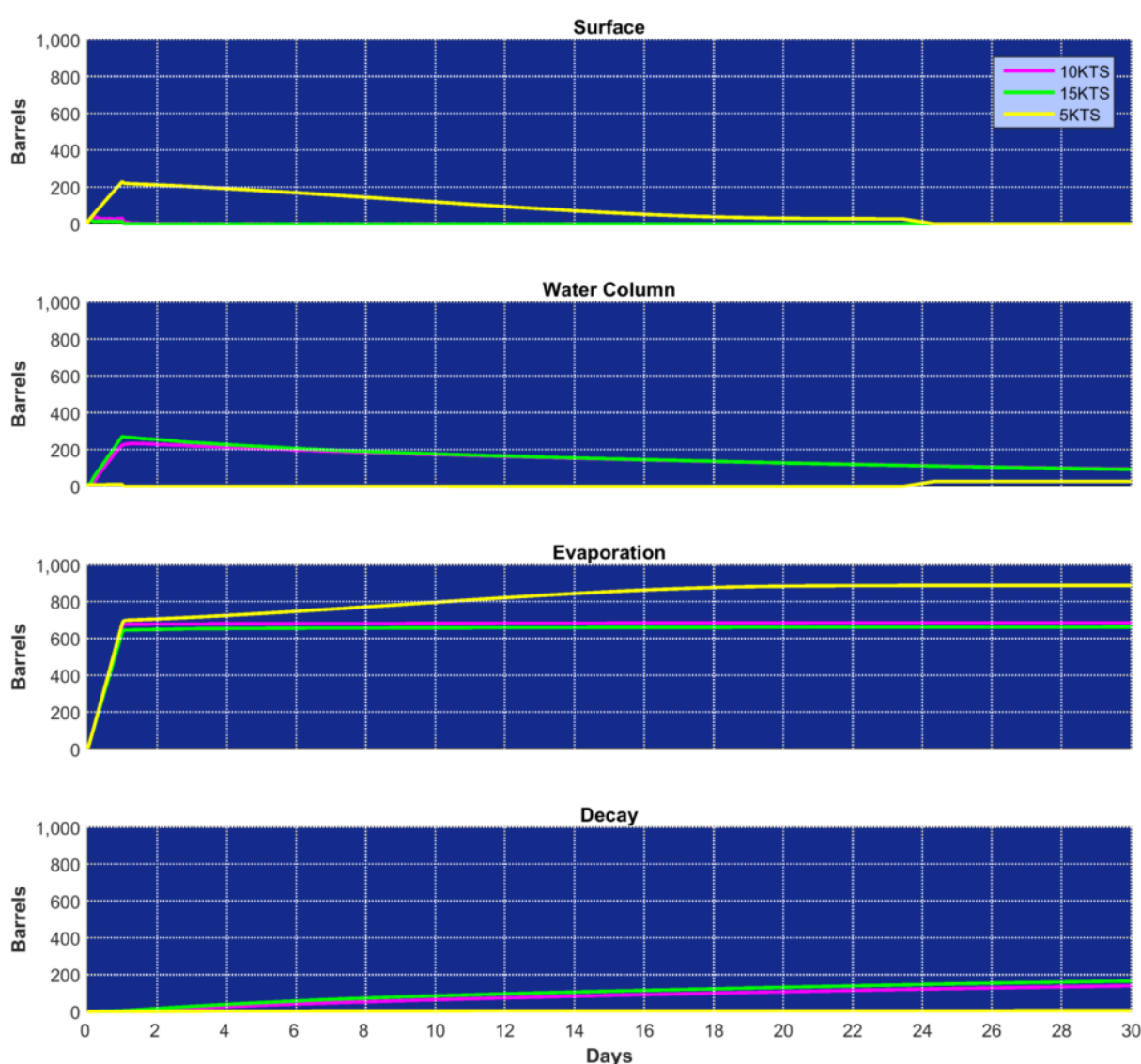
Figure 6-5 Predicted weathering and fates graph for a single spill trajectory
