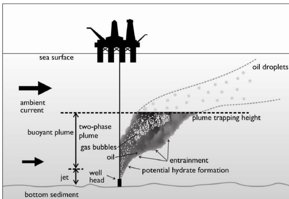
Figure 6-4 Illustration of how oil behaves when spilled to the marine environment
