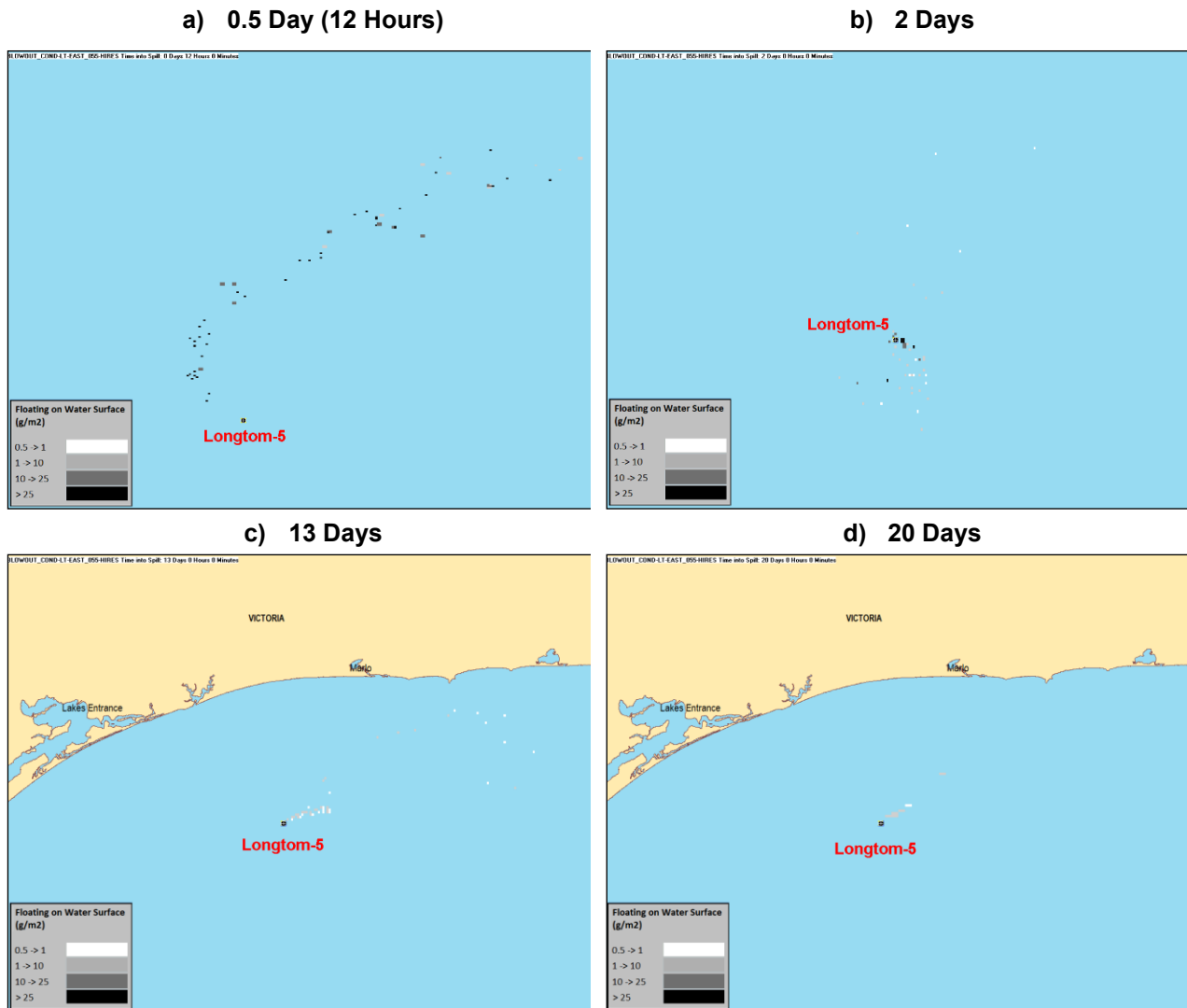
Figure 6-6 Deterministic plot of surface oil from a well blowout
