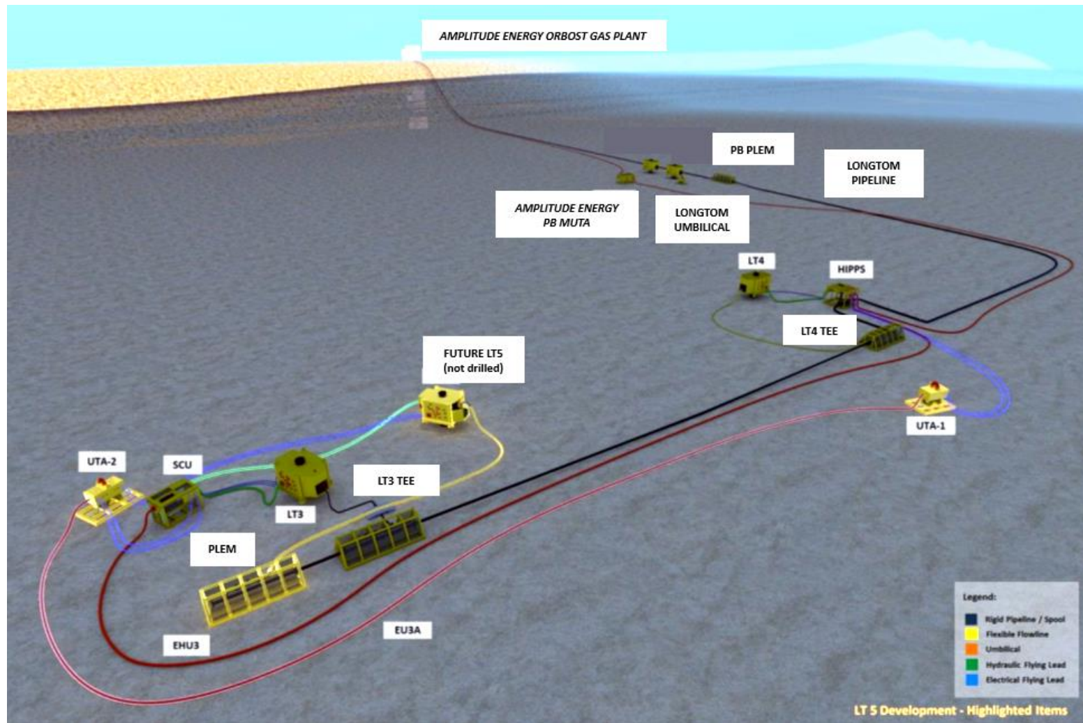
Figure 1-2 Longtom Gas Project – schematic (italicised infrastructure owned by Amplitude Energy shown for context only)
