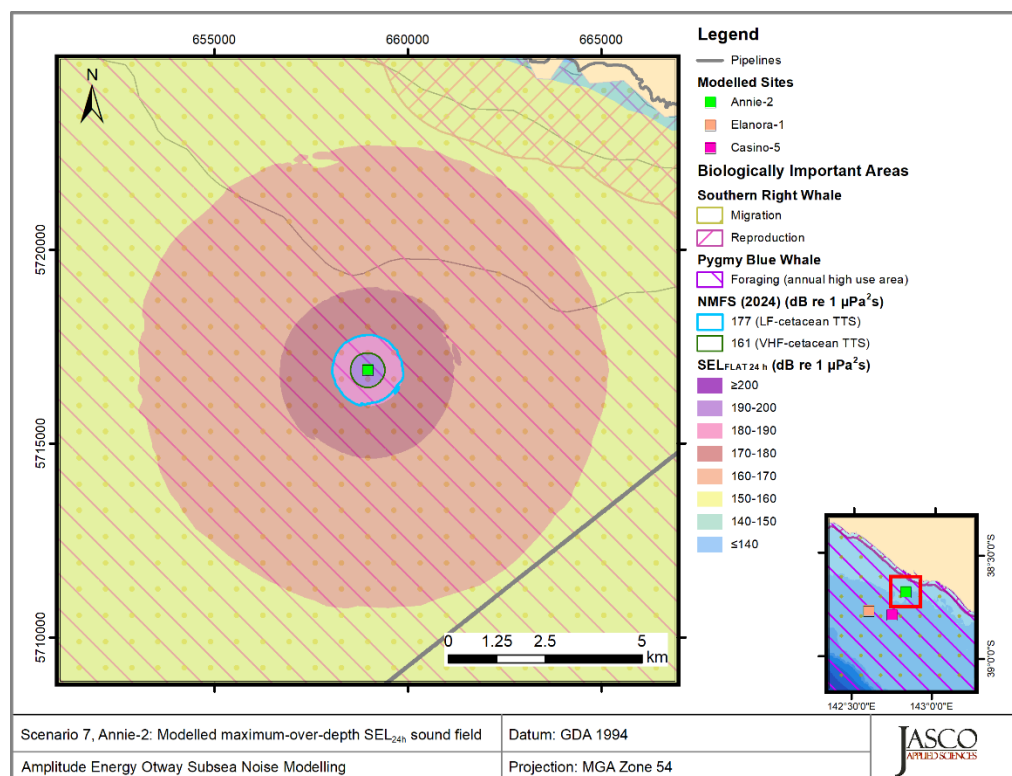
Figure 39. Scenario 7, Installation, Annie-2, accumulated SEL_{24h} : Sound level contour map showing weighted maximum-over-depth SEL_{24h} results, along with isopleths for TTS in low and very-high-frequency cetaceans. Thresholds omitted here were not reached or not long enough to display graphically.
