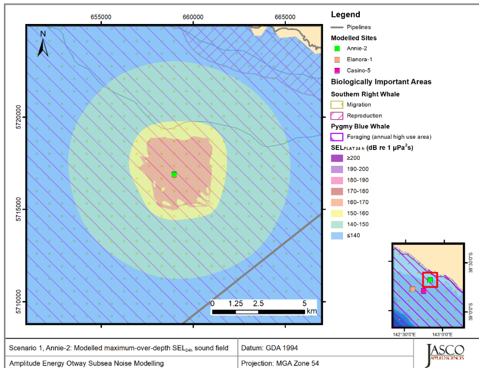
Figure 28. Scenario 1, Drilling prelays, Annie-2, accumulated SEL_{24h} : Sound level contour map showing weighted maximum-over-depth SEL_{24h} results, along with isopleths for TTS in low and very-high-frequency cetaceans. Thresholds omitted here were not reached or not long enough to display graphically.
