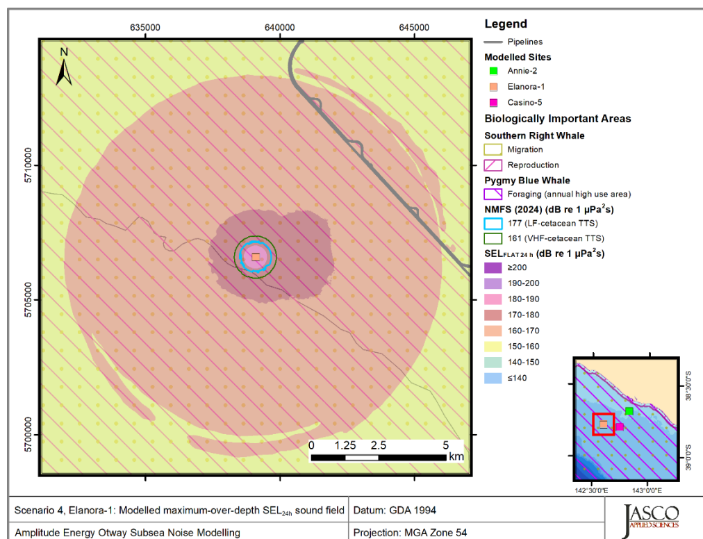
Figure 35. Scenario 4, Drilling and standby OSV, Elanora-1, accumulated SEL_{24h} : Sound level contour map showing weighted maximum-over-depth SEL_{24h} results, along with isopleths for TTS in low and very-high-frequency cetaceans. Thresholds omitted here were not reached or not long enough to display graphically.
