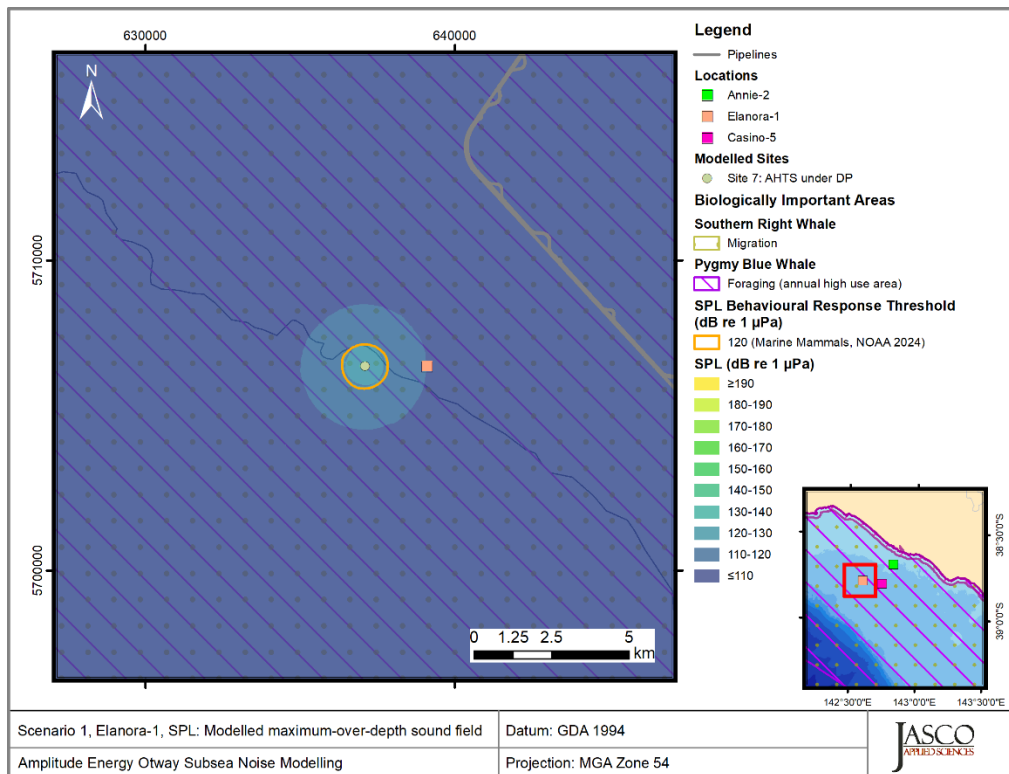
Figure 8. Scenario 1, Drilling prelays, Elanora-1, SPL : Sound level contour map showing the unweighted maximum-over-depth sound field in 10 dB steps, and the isopleths for behavioural response threshold for marine mammals.
