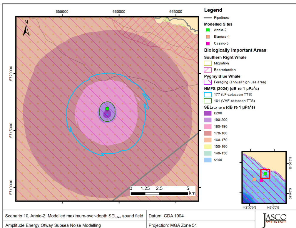
Figure 43. Scenario 10, Mooring with MODU on DP, Annie-2, accumulated SEL_{24h} : Sound level contour map showing weighted maximum-over-depth SEL_{24h} results, along with isopleths for TTS in low and very-high-frequency cetaceans. Thresholds omitted here were not reached or not long enough to display graphically.
