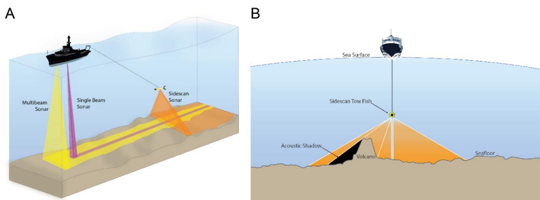
Figure 3. Graphical illustration of the differences between multi-beam, single beam, and side scan sonar. B) Graphical illustration of the side scan towfish swath coverage of the seafloor. Illustrations by Vicki Gazzola. https://ecce.esri.ca/wp-content/uploads/2022/01/Towfish.png
