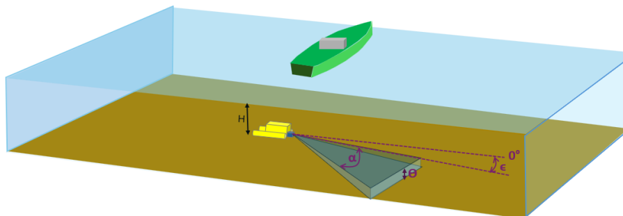
Figure 4. Geometric characteristics of the acoustic pulses generated by a forward-looking sonar mounted on an ROV. The swath generated by this configuration can be described by its horizontal directionality ( \alpha ), vertical directionality ( \theta ), and beam tilt angle ( \epsilon ).
