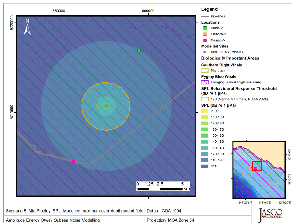
Figure 18. Scenario 6, Pipelay installation – mid, Annie-2 and Casino-5, SPL: Sound level contour map showing the unweighted maximum-over-depth sound field in 10 dB steps, and the isopleths for behavioural response threshold for marine mammals.
