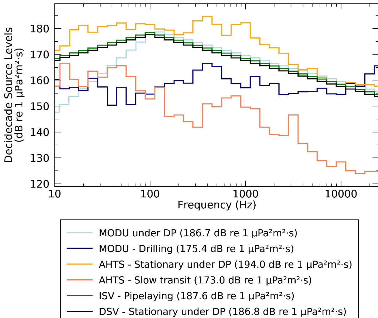
Figure 2. Source level (SL) spectra (in decidecade frequency-band) for all sound sources.
