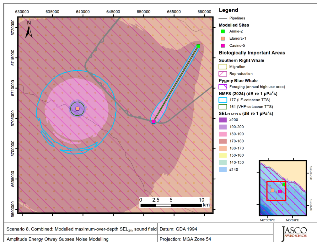
Figure 40. Scenario 8, Drilling and standby OSV during resupply and pipelay, Elanora-1 and between Annie-2 and Casino-5, accumulated SEL_{24h} : Sound level contour map showing weighted maximum-over-depth SEL_{24h} results, along with isopleths for TTS in low and very-high-frequency cetaceans. Thresholds omitted here were not reached or not long enough to display graphically.
