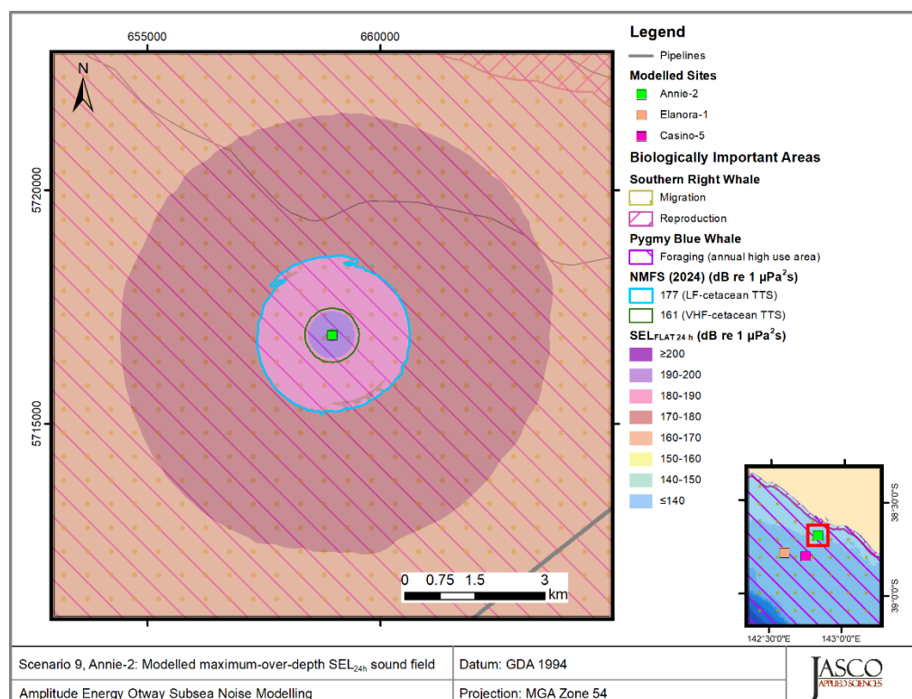
Figure 41. Scenario 9, MODU on DP, Annie-2, accumulated SEL_{24h} : Sound level contour map showing weighted maximum-over-depth SEL_{24h} results, along with isopleths for TTS in low and very-high-frequency cetaceans. Thresholds omitted here were not reached or not long enough to display graphically.
