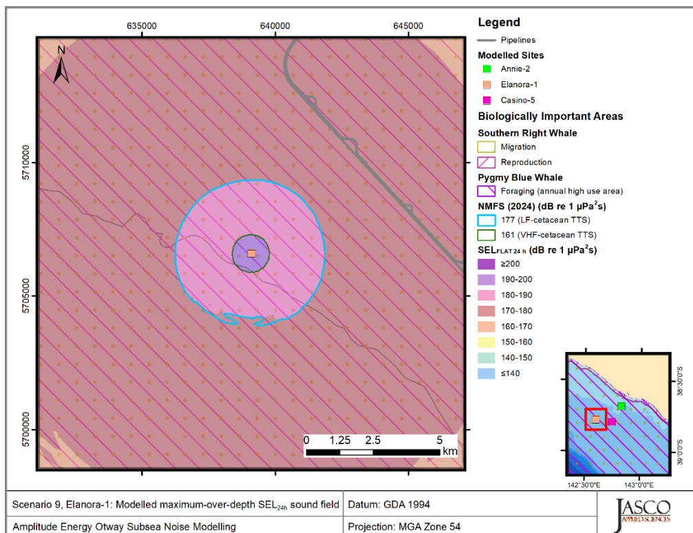
Figure 42. Scenario 9, MODU on DP, Elanora-1, accumulated SEL_{24h} : Sound level contour map showing weighted maximum-over-depth SEL_{24h} results, along with isopleths for TTS in low and very-high-frequency cetaceans. Thresholds omitted here were not reached or not long enough to display graphically.
