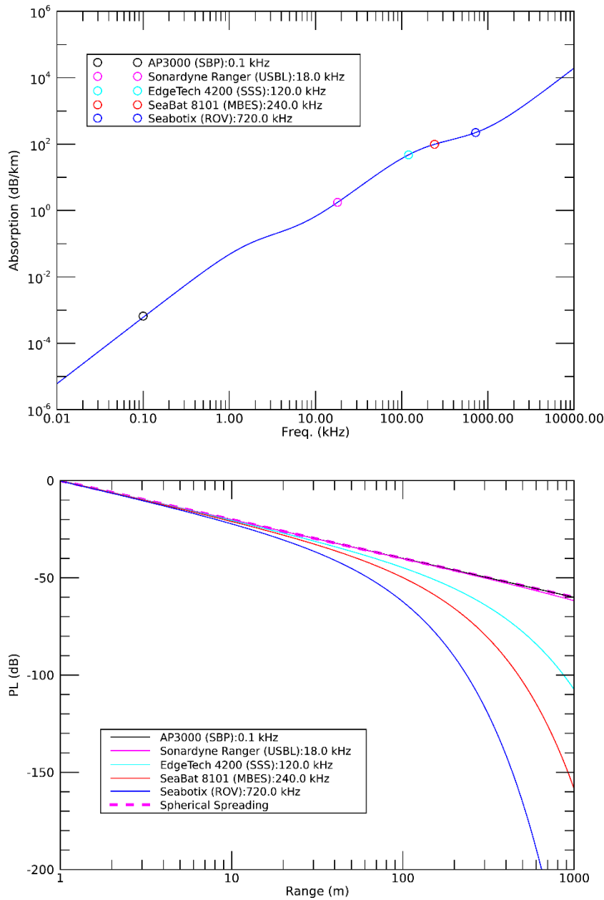
Figure 1. (Top) Sound absorption in seawater with circles (o) indicating the frequencies of the systems considered in this study. (Bottom) Propagation loss (water absorption + spherical spreading) at the frequencies of the systems considered in this study. The propagation loss due to spherical spreading alone is presented as a dashed line.
