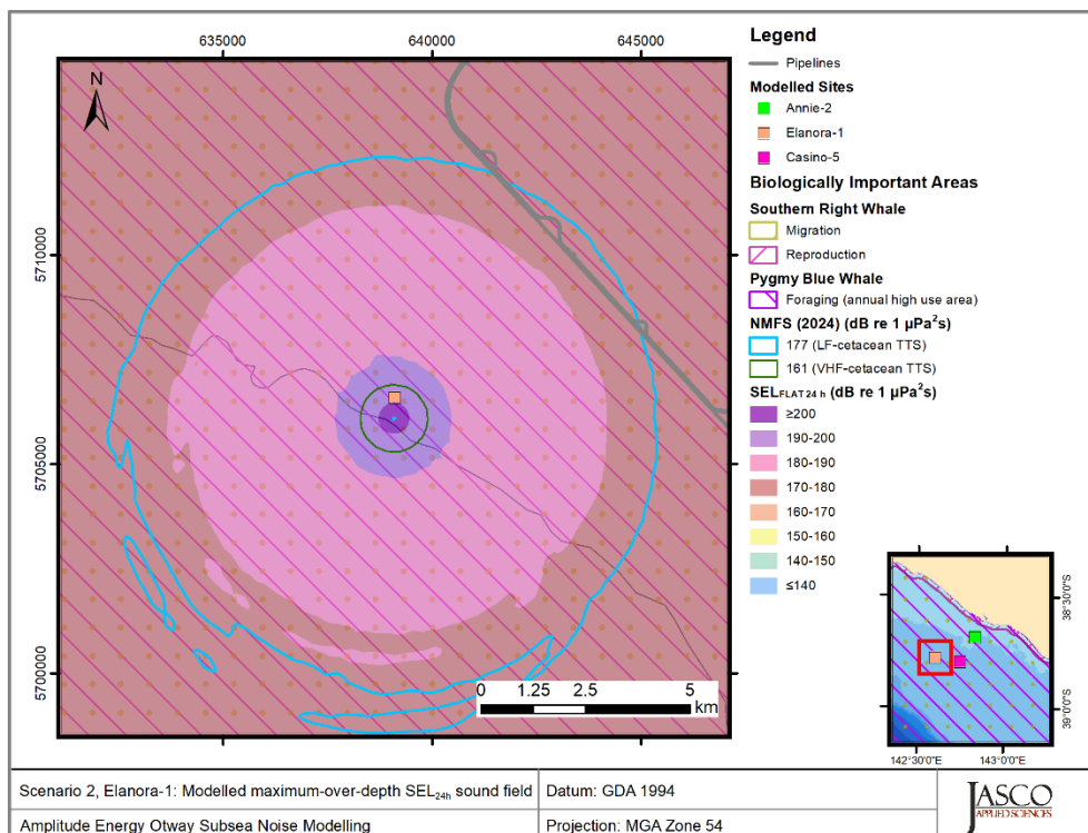
Figure 31. Scenario 2, Mooring, Elanora-1, accumulated SEL_{24h} : Sound level contour map showing weighted maximum-over-depth SEL_{24h} results, along with isopleths for TTS in low and very-high-frequency cetaceans. Thresholds omitted here were not reached or not long enough to display graphically.
