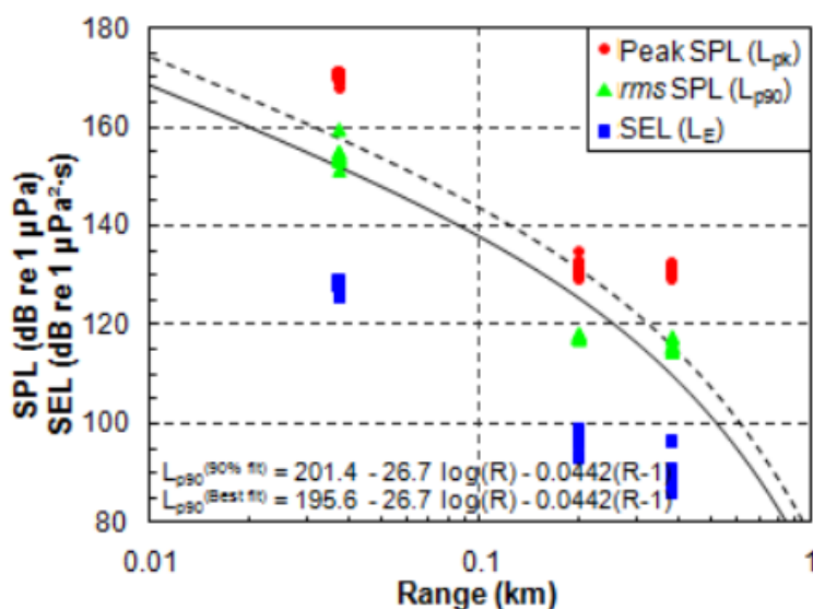
Figure 2. Figure 3.103 in Chorney et al. (2011). Multibeam sonar (RESON SeaBat 8101) 240 kHz pulse in-beam PK (peak SPL), 90% rms SPL, and SEL versus range, at 7 m receiver depth. Solid line is best fit of the empirical function to L_{p90} values. Dashed line is the best-fit shifted to exceed 90% of the L_{p90} values (90th percentile fit). Measurements at 200 and 380 m range are near background noise levels of these recordings.
