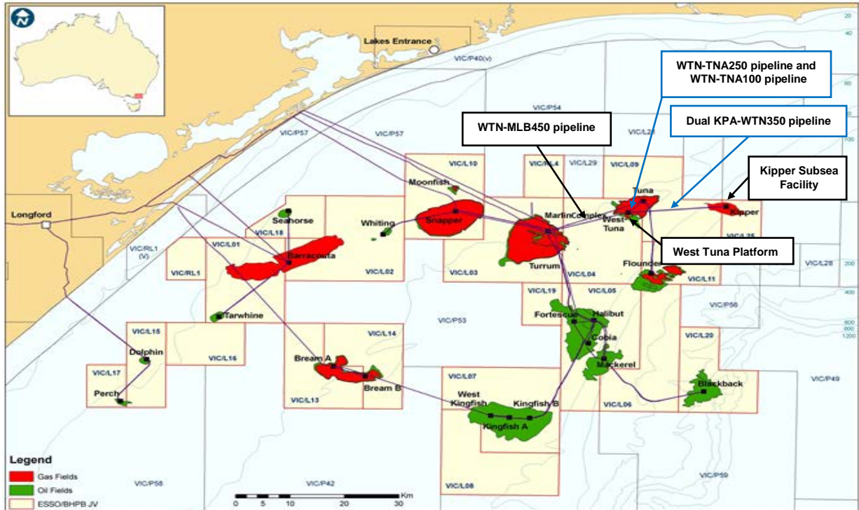
Figure 1 Esso production facilities in Bass Strait
