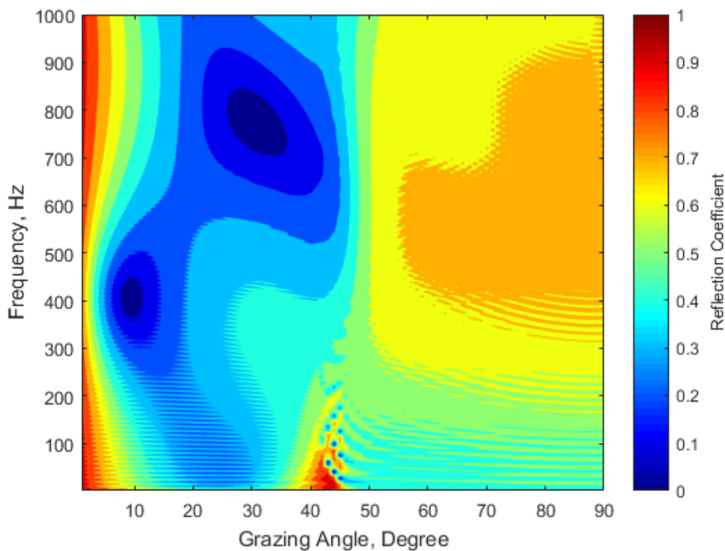
Figure 9 Reflection coefficient variations with grazing angle and frequency for the geo-acoustic model
