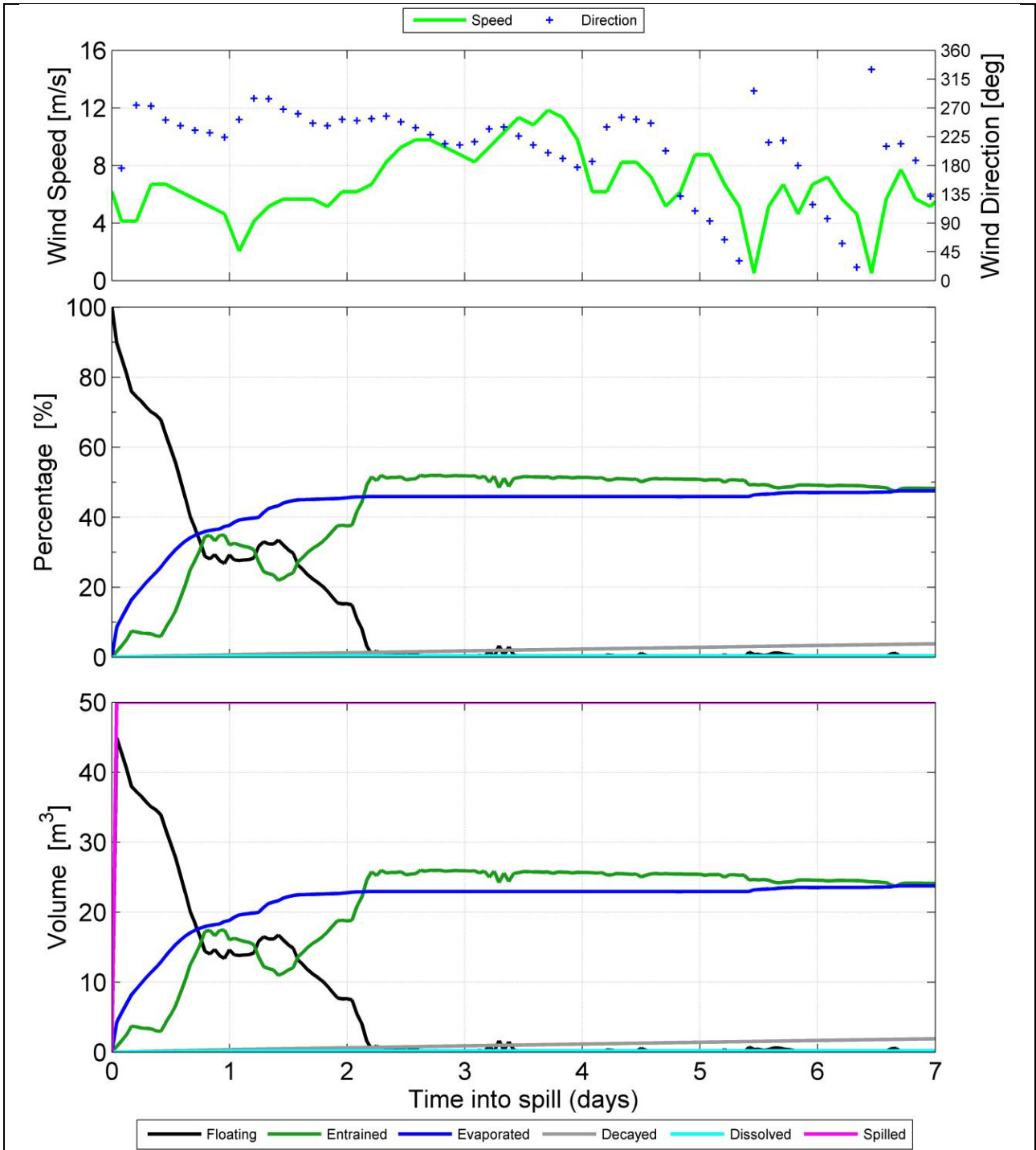
Figure 6-5: Mass balance plot representing, as proportion (middle panel) and volume (bottom panel), the weathering of marine diesel spilled onto the water surface as a one-off release (50 m 3 over one hour) and subject to variable wind at 27 °C water temperature and 25 °C air temperature
