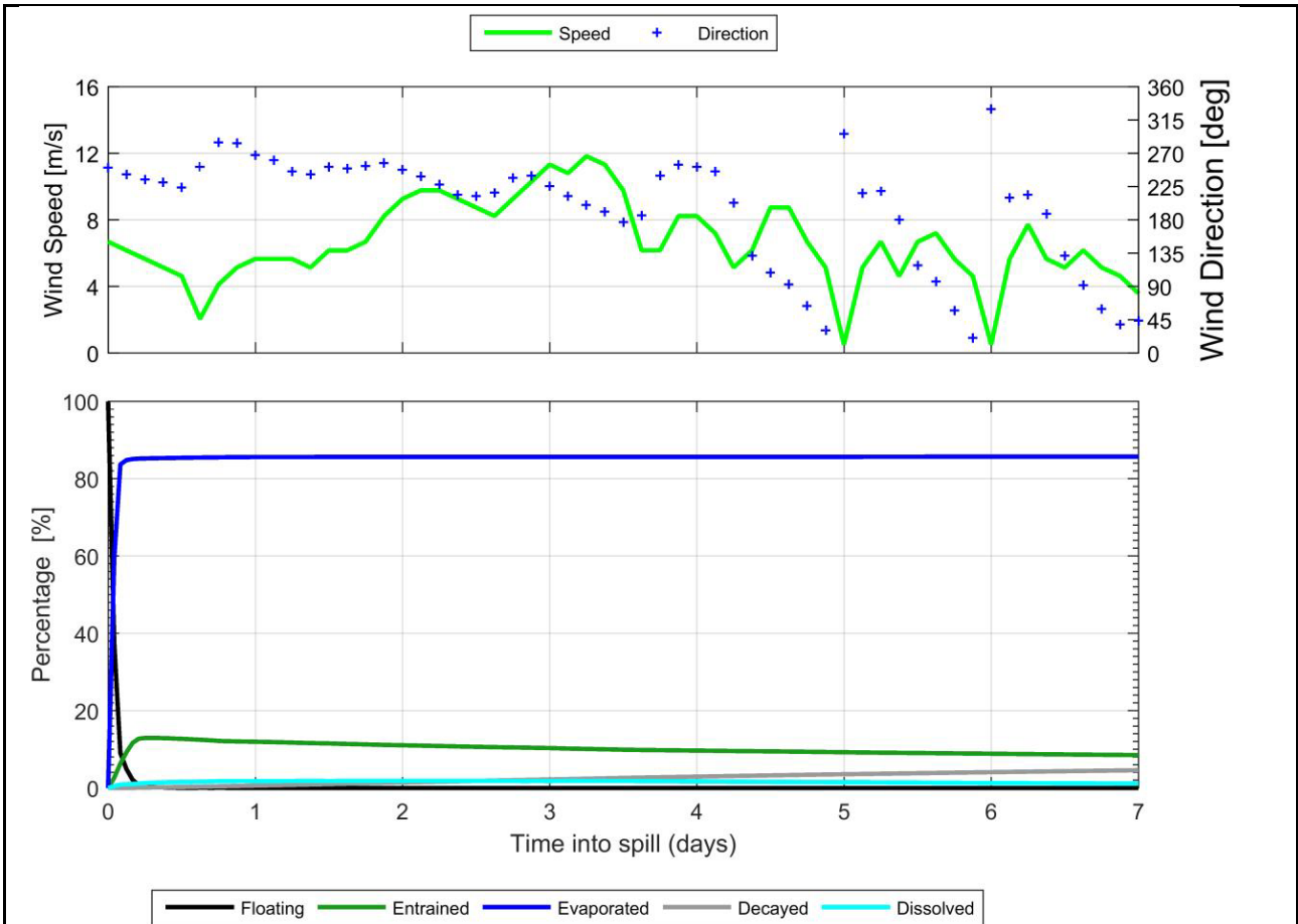
Figure 6-3: Time series wind speed and percentage mass balance plots for the weathering of Pyxis condensate (subsea) spilled onto the water column as a one-off release and subject to variable wind at 27 °C water temperature and 25 °C air temperature
