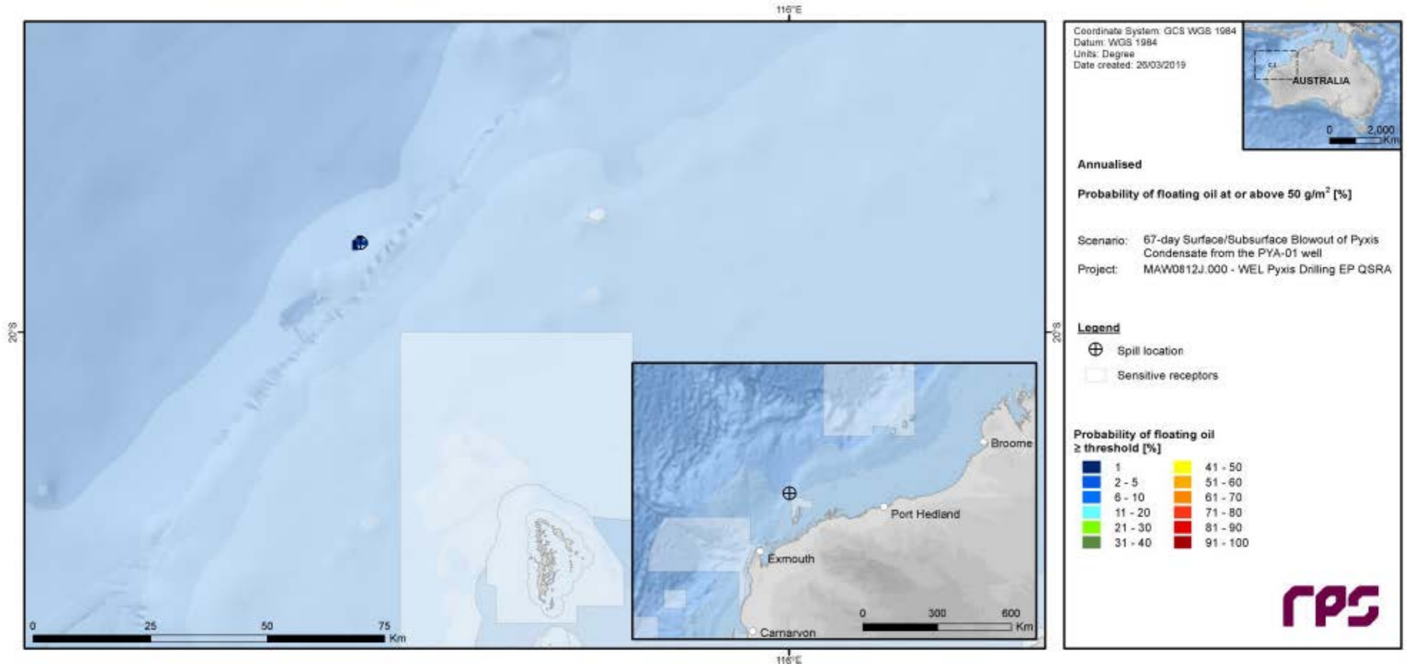
Figure 2-5 Predicted annualised probability of floating oil concentration at 50 g/m 2 for a 67-day surface/subsurface release of Pyxis Condensate at the PYA-01 well.
