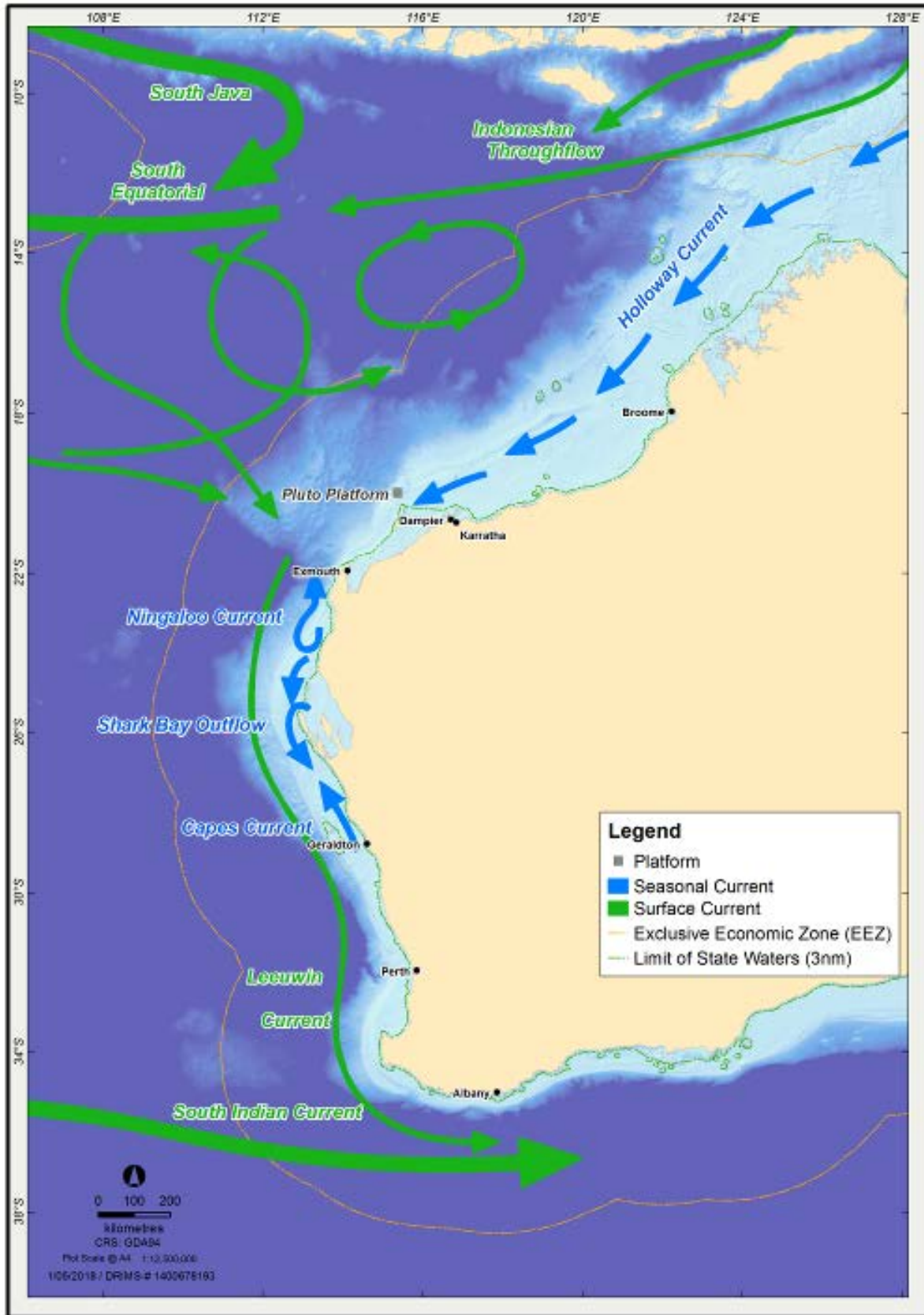
Figure 4-5: Large-scale ocean circulation of the North West Marine Region including the location of the Indonesian Throughflow and other significant currents (DEWHA, 2008)
