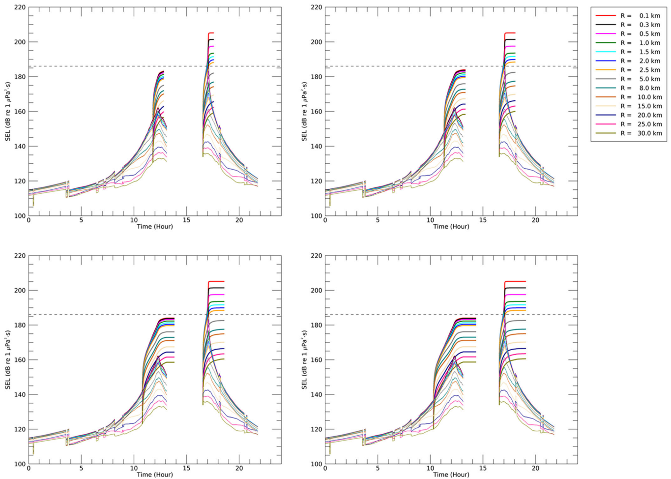
Figure 6-10: Example of maximum-over-depth per-pulse unweighted SEL (thin lines) and accumulated unweighted SEL (thick lines) for fourteen receiver locations at increasing distance from the survey lines for Scenario 1. Clockwise from top-left the plots show accumulation over a 1, 2, 3 and 4 hour window. Gaps in the per-pulse curves correspond to vessel turns. The horizontal black dashed line corresponds to the fish TTS threshold of 186 dB re 1 μPa 2 ·s
