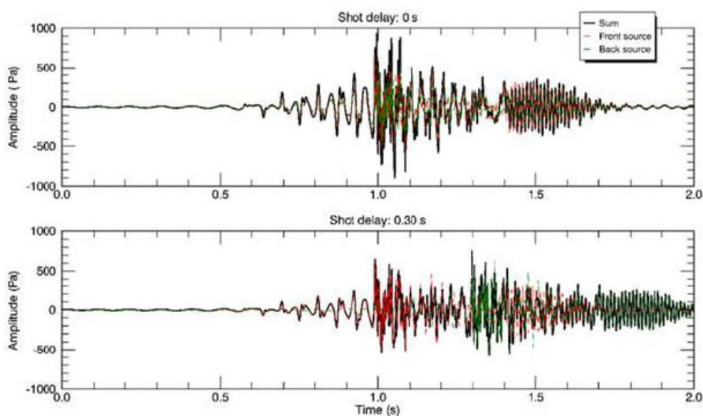
Figure 6-25: Two separate pulses of sound occurring in synch (top) and out of synch (bottom) (Quijano et al. 2018)
