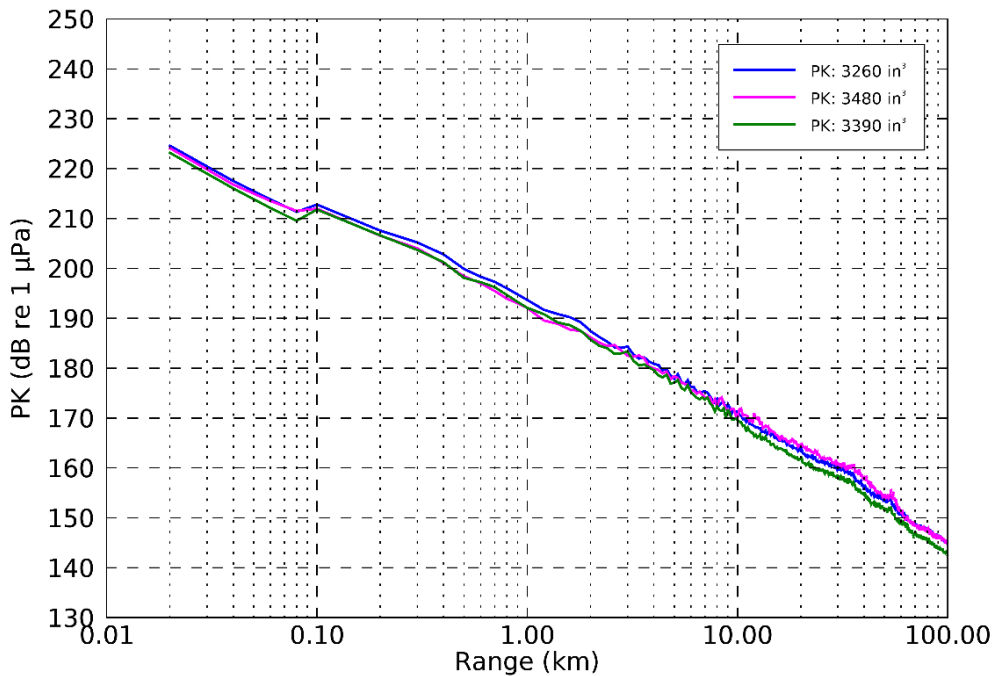
Figure 6-6: FWRAM model output comparing the PK levels over horizontal distance within the water column from three seismic sources (Source: JASCO Applied Sciences).
