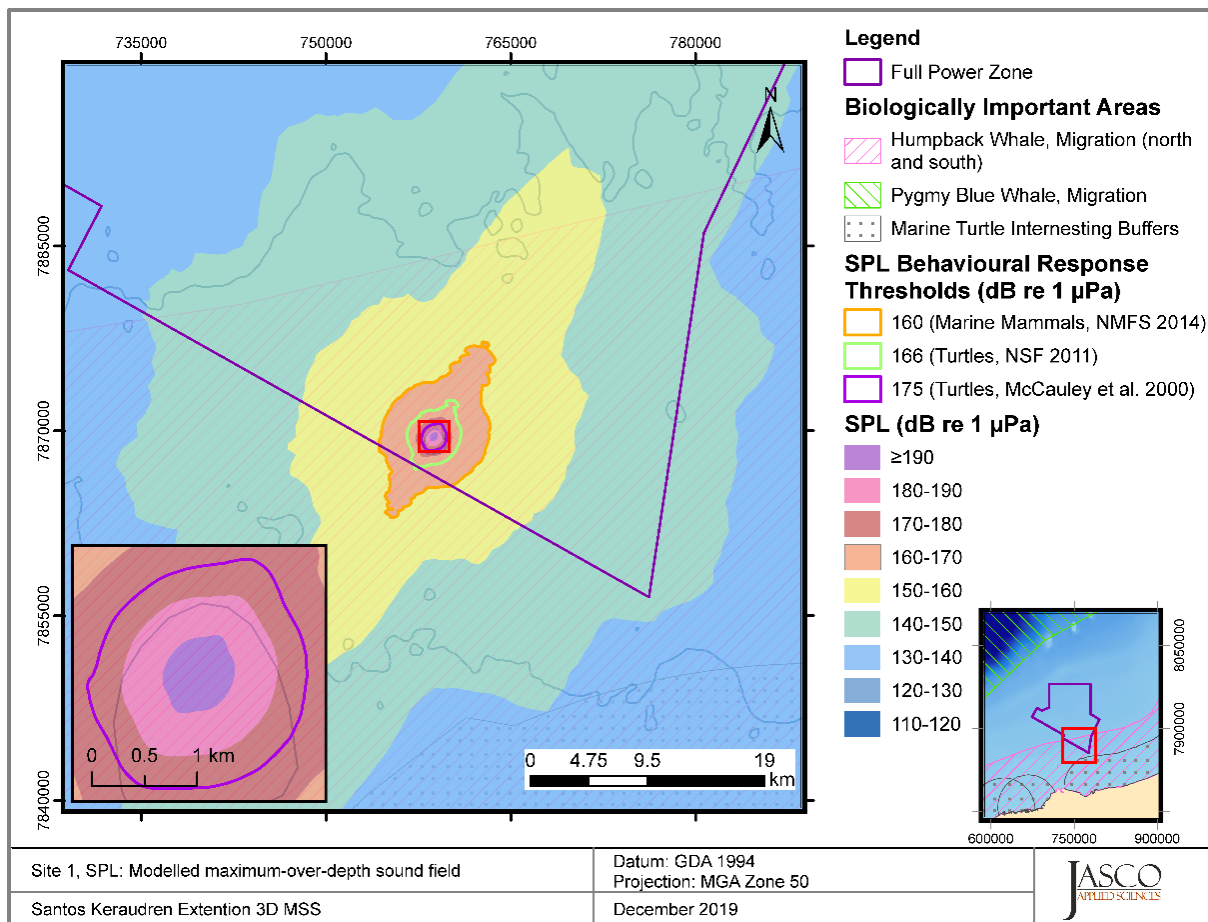
Figure 6-8: Sound level contour map showing unweighted maximum-over-depth per-pulse SPL results for the primary 3,260 in 3 seismic source (Scenario 1, site 1) (Source: JASCO Applied Sciences).
