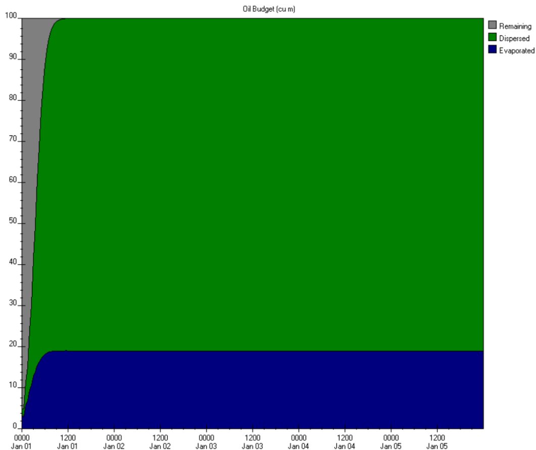
Figure 6-3: Percentage of oil remaining from a 100 m 3 of diesel spill due to vessel collision
