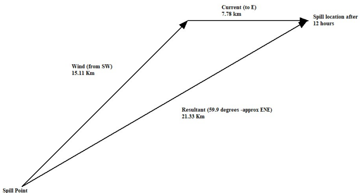
Figure 6-4: Travel distance of a 100 m 3 of diesel spill due to vessel collision
