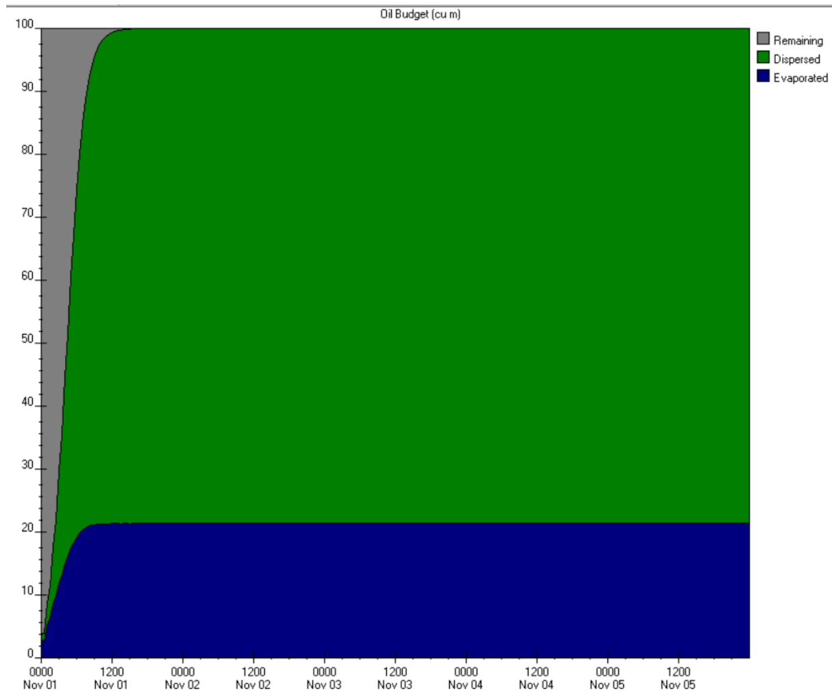
Figure 6-4: Percentage of oil remaining from a 100 m 3 of diesel spill due to vessel collision
