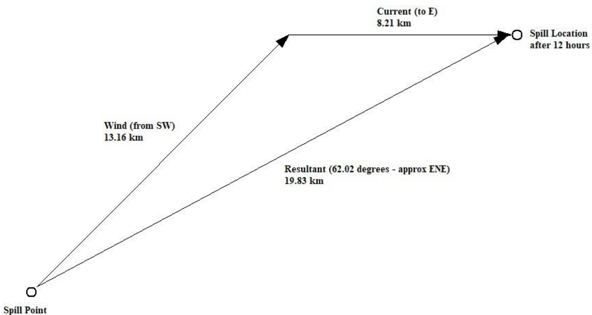
Figure 6-5: Travel distance of a 100 m 3 of diesel spill due to vessel collision
