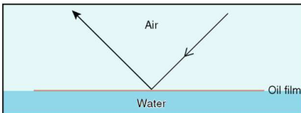
Figure 10: Light Reflecting From Very Thin Oil Films
