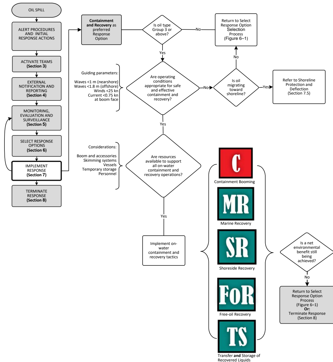
Figure 7-5: On-Water Containment and Recovery Decision Guide
