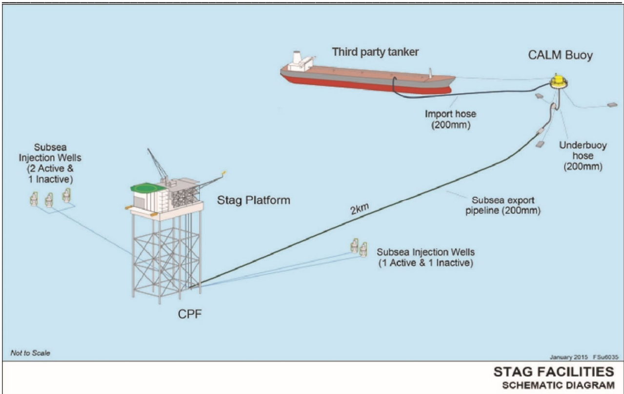
Figure 1-1: Schematic of the Stag Facility
