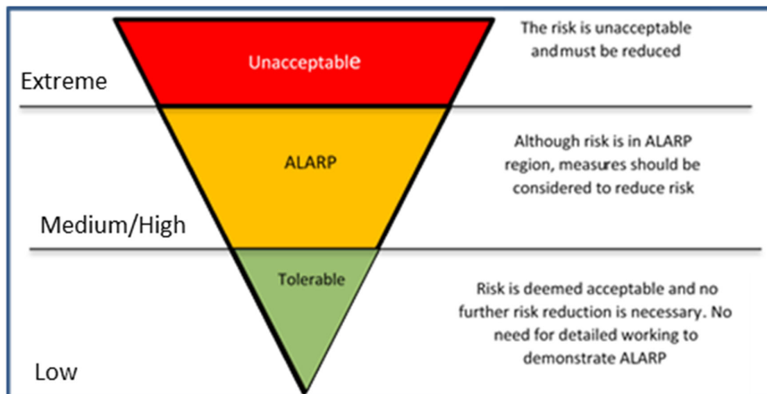
Figure 4-2: ALARP Triangle
