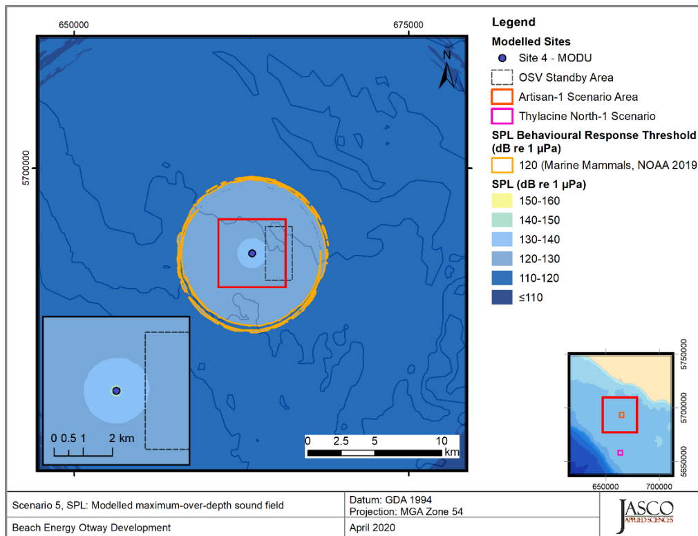
Figure 17. Artisan-1, MODU (Scenario 5), SPL: Sound level contour map, showing unweighted maximum-over-depth SPL results. Isoleth for marine mammal (120 dB re 1 µPa) behavioural criteria is shown as an orange contour line.
