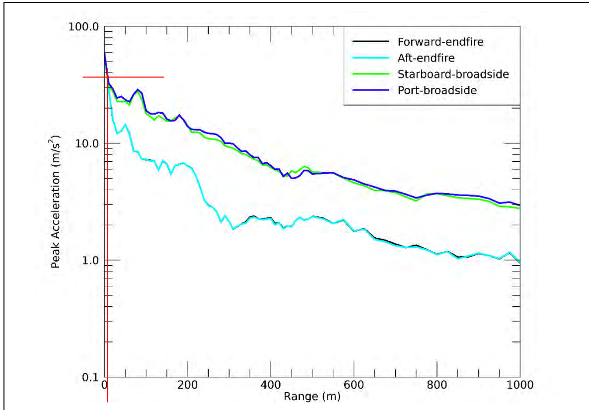
Figure 7.8. Maximum particle acceleration at the seafloor as a function of horizontal range from the centre of the seismic source along four directions at Site 3 (79 m water depth)
