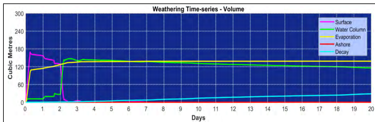
Figure 7.14. Predicted weathering and fate of MDO for the largest swept area based on a 280 m 3 surface release of MDO over 6 hours and tracked for 20 days based on 200 spill trajectories during annual conditions
