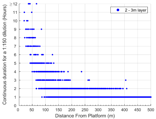
Figure 2-16 Scatter plots presenting the maximum continuous hours the PFW stream concentration occurred at, or below, equivalent dilution of 1:150 for the whole PFW stream. Modelling based on a flow rate of 37,500 kL/d during summer (January) conditions for the 0 – 1m (top plot), 1 – 2m (middle plot) and 2 – 3m depth layers (bottom plot).
