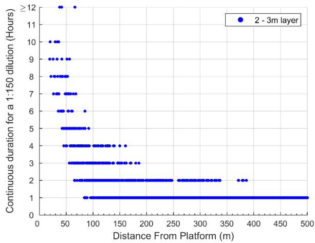
Figure 2-6 Scatter plots presenting the maximum continuous hours the PFW stream concentration occurred at, or below, equivalent dilution of 1:150 for the whole PFW stream. Modelling based on a flow rate of 33,500 kL/d during summer (January) conditions for the 0 – 1m (top plot), 1 – 2m (middle plot) and 2 – 3m depth layers (bottom plot)
