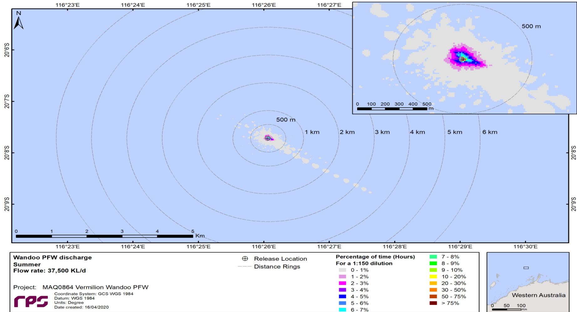
Figure 2-15 Spatial plots of percentage of time (hours) the PFW stream concentration occurred at, or below, equivalent dilution of 1:150 for the whole PFW stream. Modelling based on a flow rate of 37,500 kL/d during summer (January) conditions .
