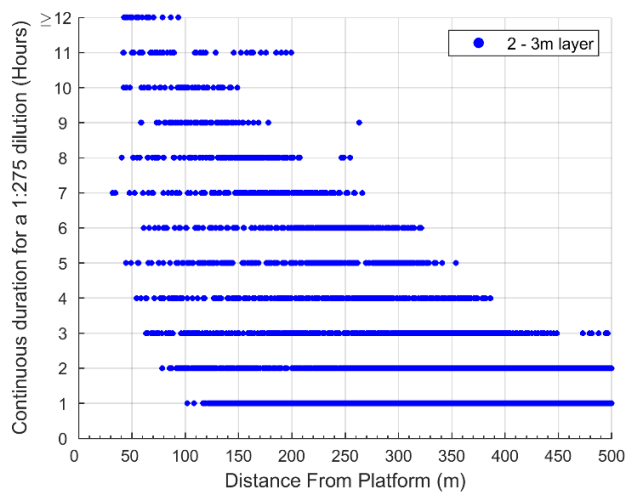
Figure 2-2 Scatter plots presenting the maximum continuous hours the PFW stream concentration occurred at, or below, equivalent dilution of 1:275 for the whole PFW stream. Modelling based on a flow rate of 33,500 kL/d during winter (July) conditions for the 0 – 1m (top plot), 1 – 2m (middle plot) and 2 – 3m depth layers (bottom plot)
