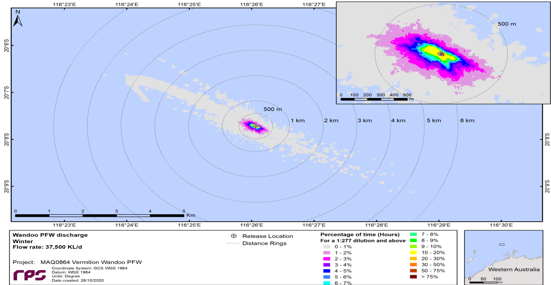
Figure 2-19 Spatial plots of percentage of time (hours) the PFW stream concentration occurred at, or below, equivalent dilution of 1:277 for the whole PFW stream. Modelling based on a flow rate of 37,500 kL/d during winter(July) conditions
