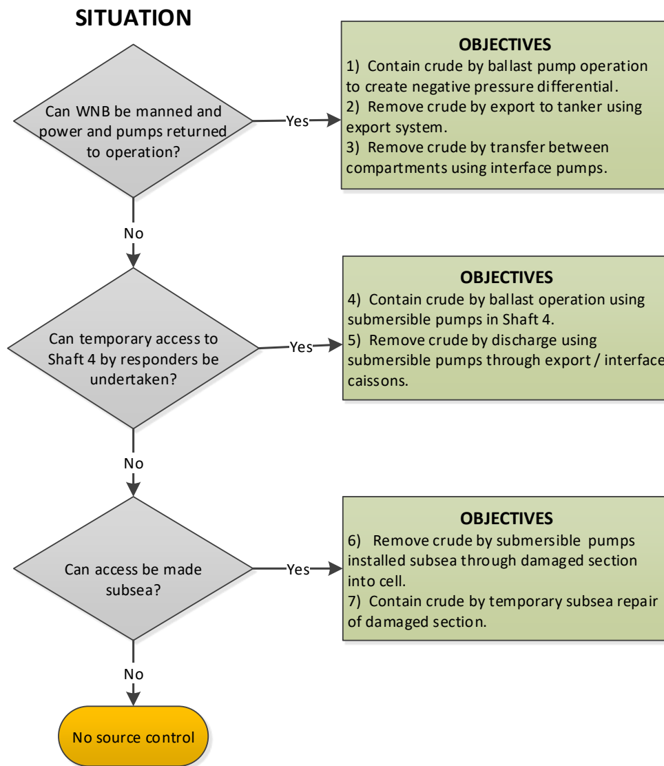
Figure 6-5 CGS source control situations and objectives flowchart
