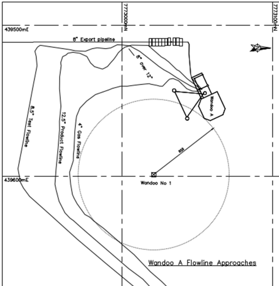
Figure 2-3 Wandoo-1 Location (WNB-5000-DG-0004.11)
