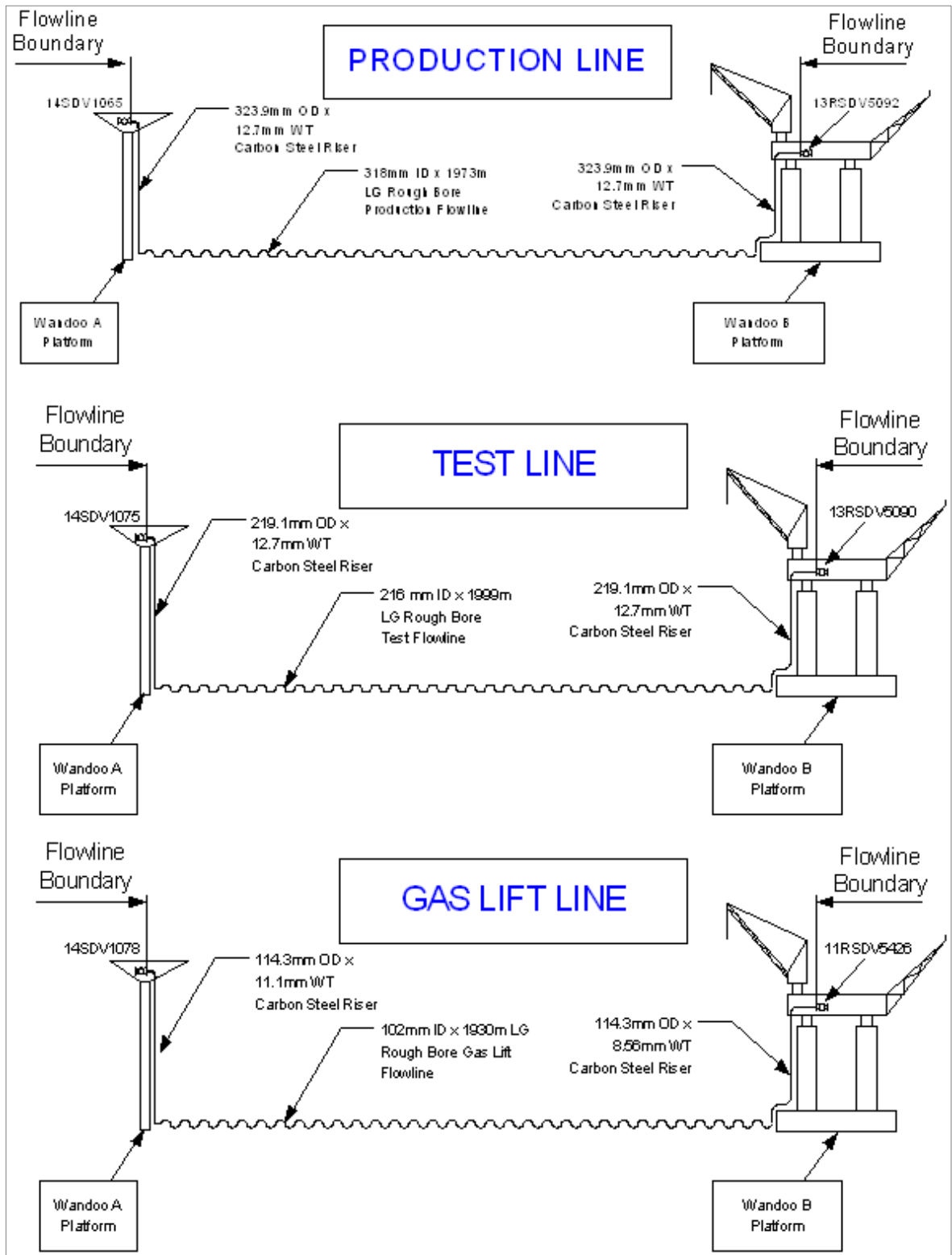
Figure 2-5: Production, test and gas lift lines
