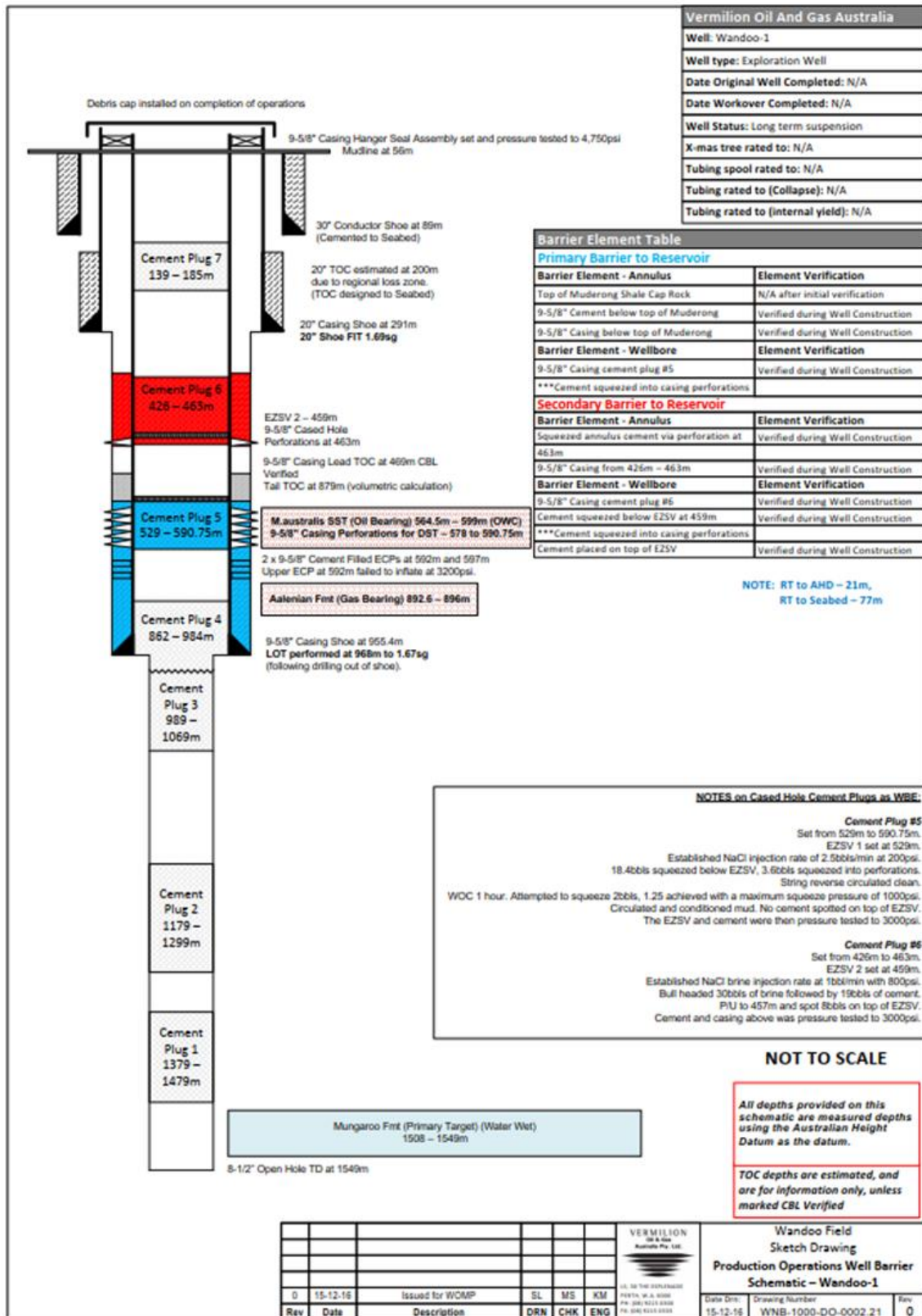
Figure 2-4 Wandoo-1 Well Barrier Schematic
