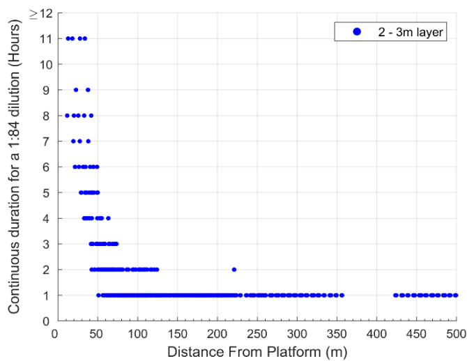
Figure 2-22 Scatter plots presenting the maximum continuous hours the PFW stream concentration occurred at, or below, equivalent dilution of 1:84 for the whole PFW stream. Modelling based on a flow rate of 33,500 kL/d during summer (January) conditions for the 0 – 1m (top plot), 1 – 2m (middle plot) and 2 – 3m depth layers (bottom plot).
