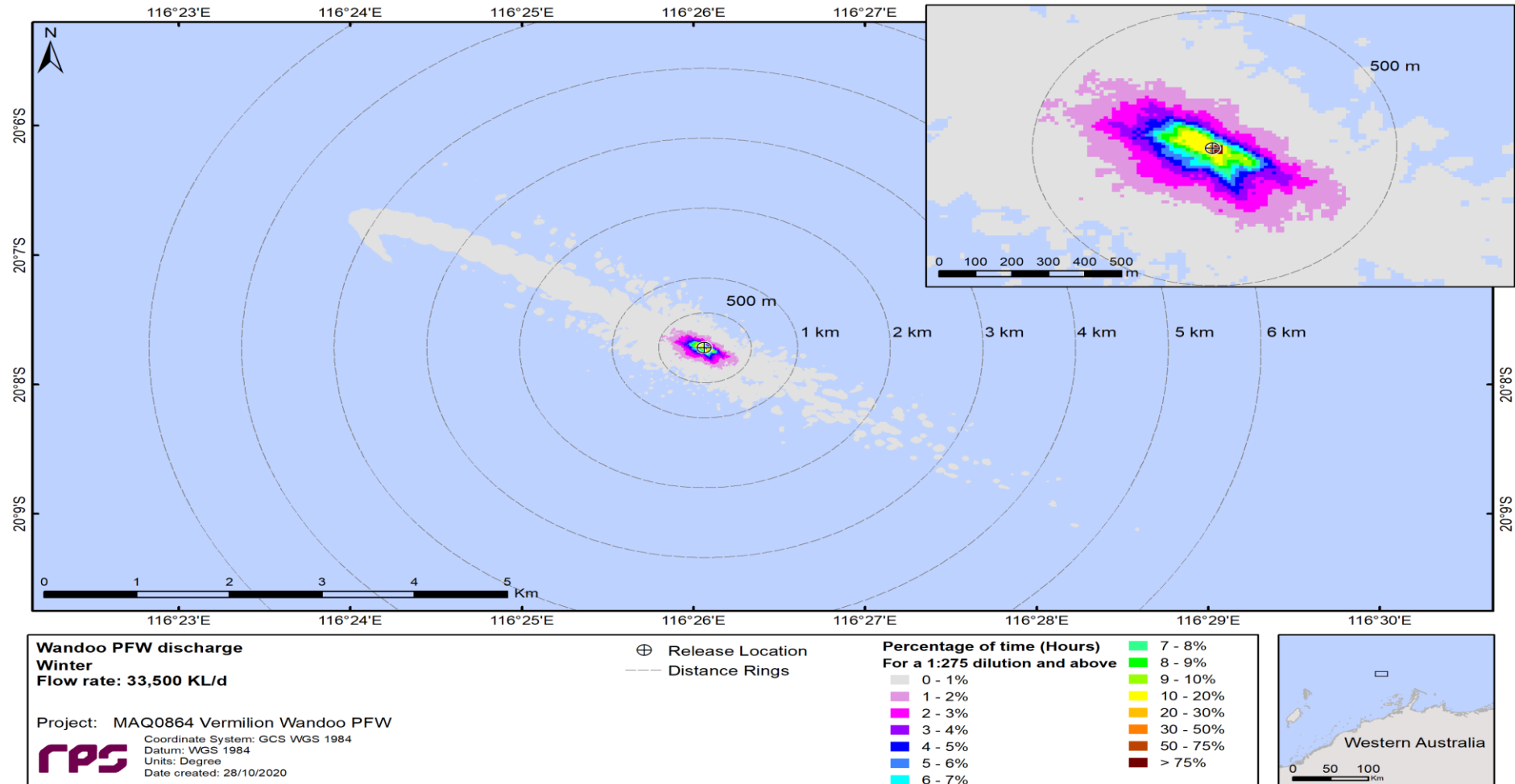
Figure 2-1 Spatial plots of percentage of time (hours) the PFW stream concentration occurred at, or below, equivalent dilution of 1:275 for the whole PFW stream. Modelling based on a flow rate of 33,500 kL/d during winter (July) conditions .
