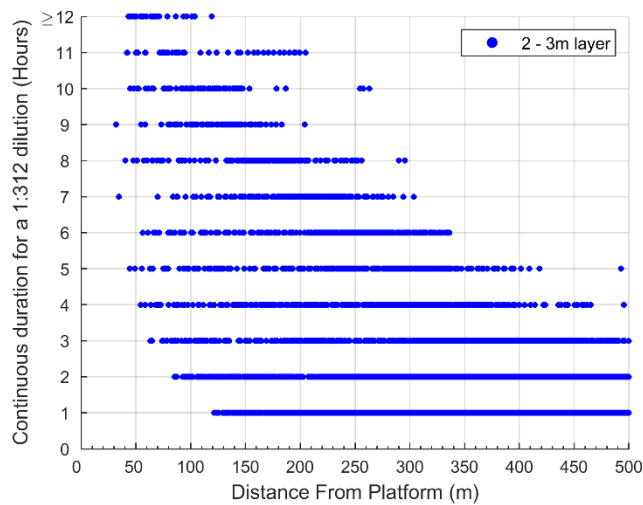
Figure 2-18 Scatter plots presenting the maximum continuous hours the PFW stream concentration occurred at, or below, equivalent dilution of 1:312 for the whole PFW stream. Modelling based on a flow rate of 33,500 kL/d during winter (July) conditions for the 0 – 1m (top plot), 1 – 2m (middle plot) and 2 – 3m depth layers (bottom plot)
