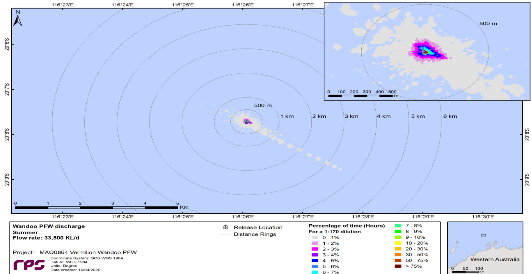
Figure 2-13 Spatial plots of percentage of time (hours) the PFW stream concentration occurred at, or below, equivalent dilution of 1:170 for the whole PFW stream. Modelling based on a flow rate of 33,500 kL/d during summer (January) conditions .
