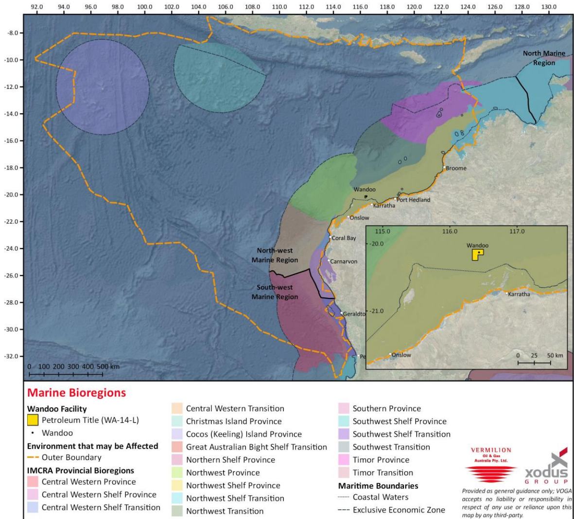
Figure 4-2: Marine Bioregions
