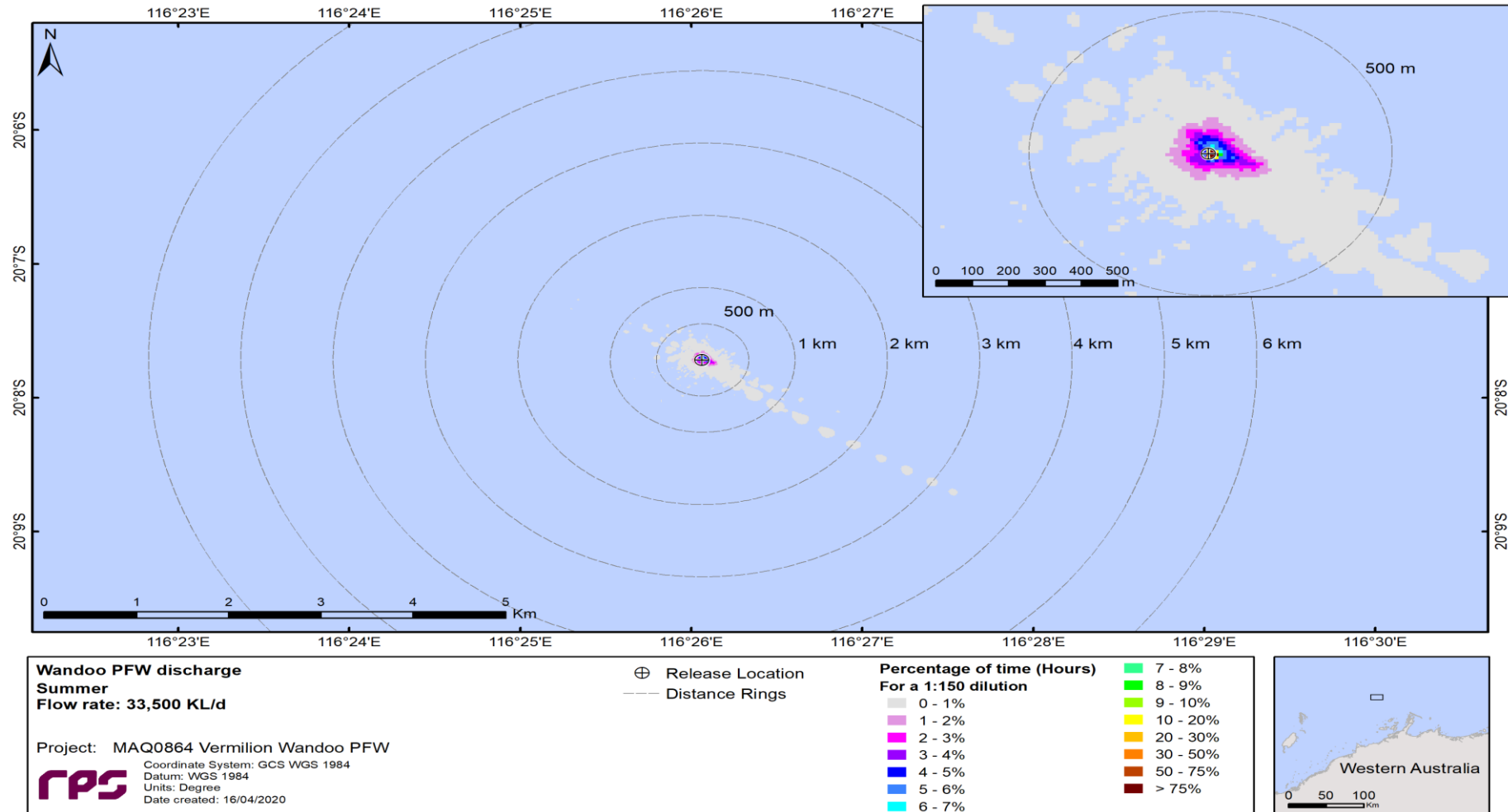
Figure 2-5 Spatial plots of percentage of time (hours) the PFW stream concentration occurred at, or below, equivalent dilution of 1:150 for the whole PFW stream. Modelling based on a flow rate of 33,500 kL/d during summer (January) conditions .
