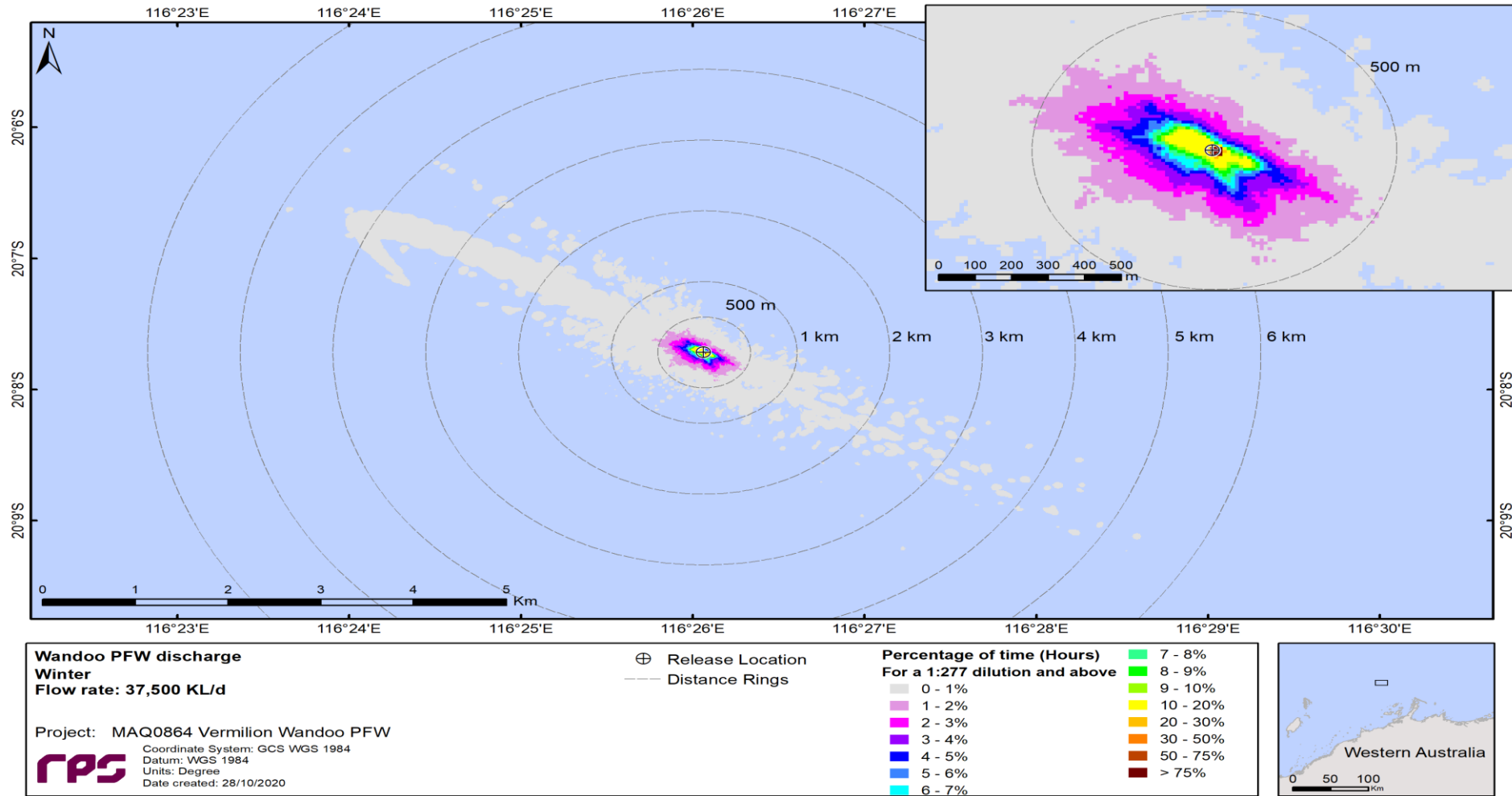
Figure 2-3 Spatial plots of percentage of time (hours) the PFW stream concentration occurred at, or below, equivalent dilution of 1:277 for the whole PFW stream. Modelling based on a flow rate of 37,500 kL/d during winter (July) conditions
