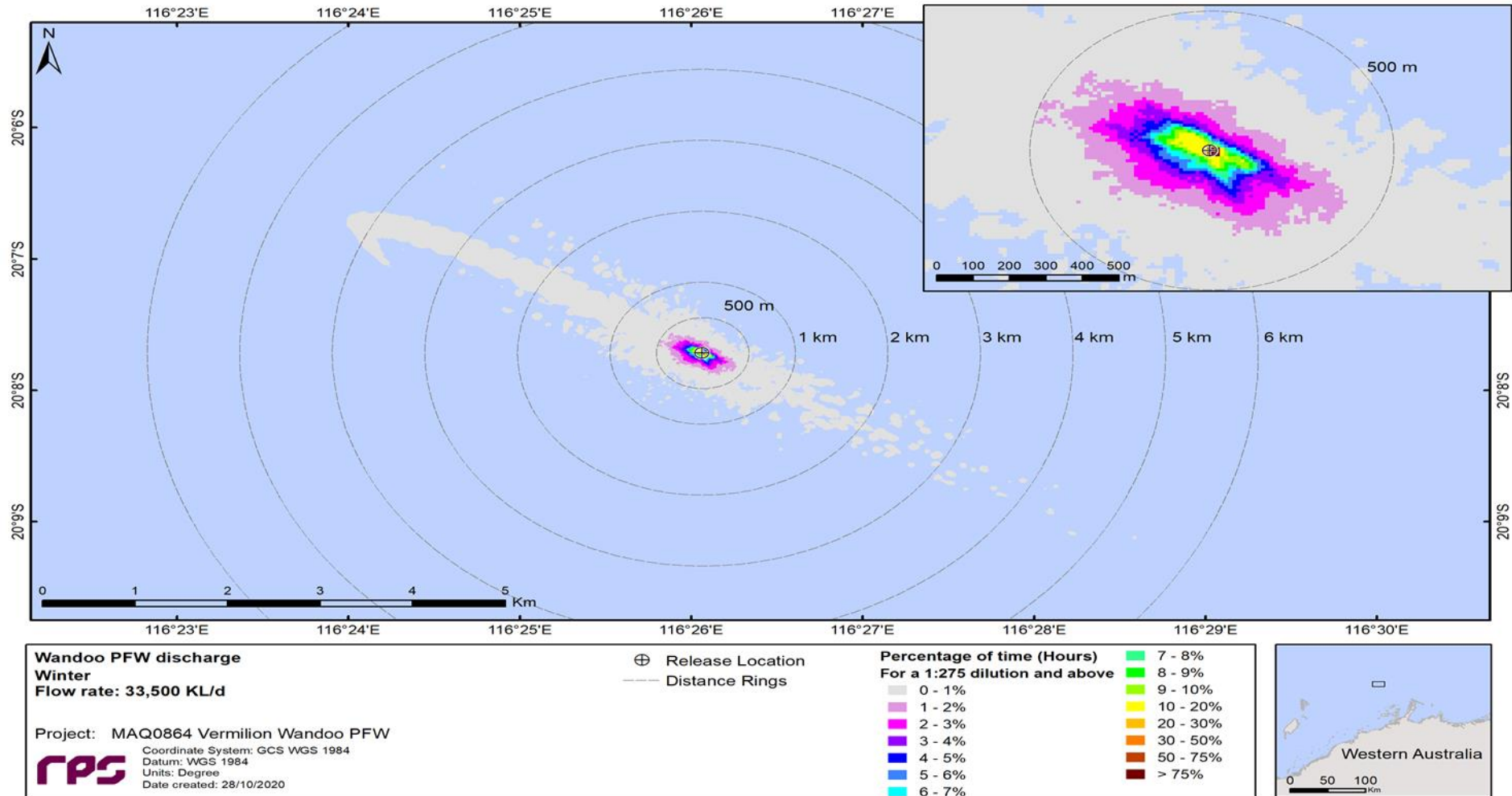
Figure 2-9 Spatial plots of percentage of time (hours) the PFW stream concentration occurred at, or below, equivalent dilution of 1:275 for the whole PFW stream. Modelling based on a flow rate of 33,500 kL/d during winter (July) conditions .
