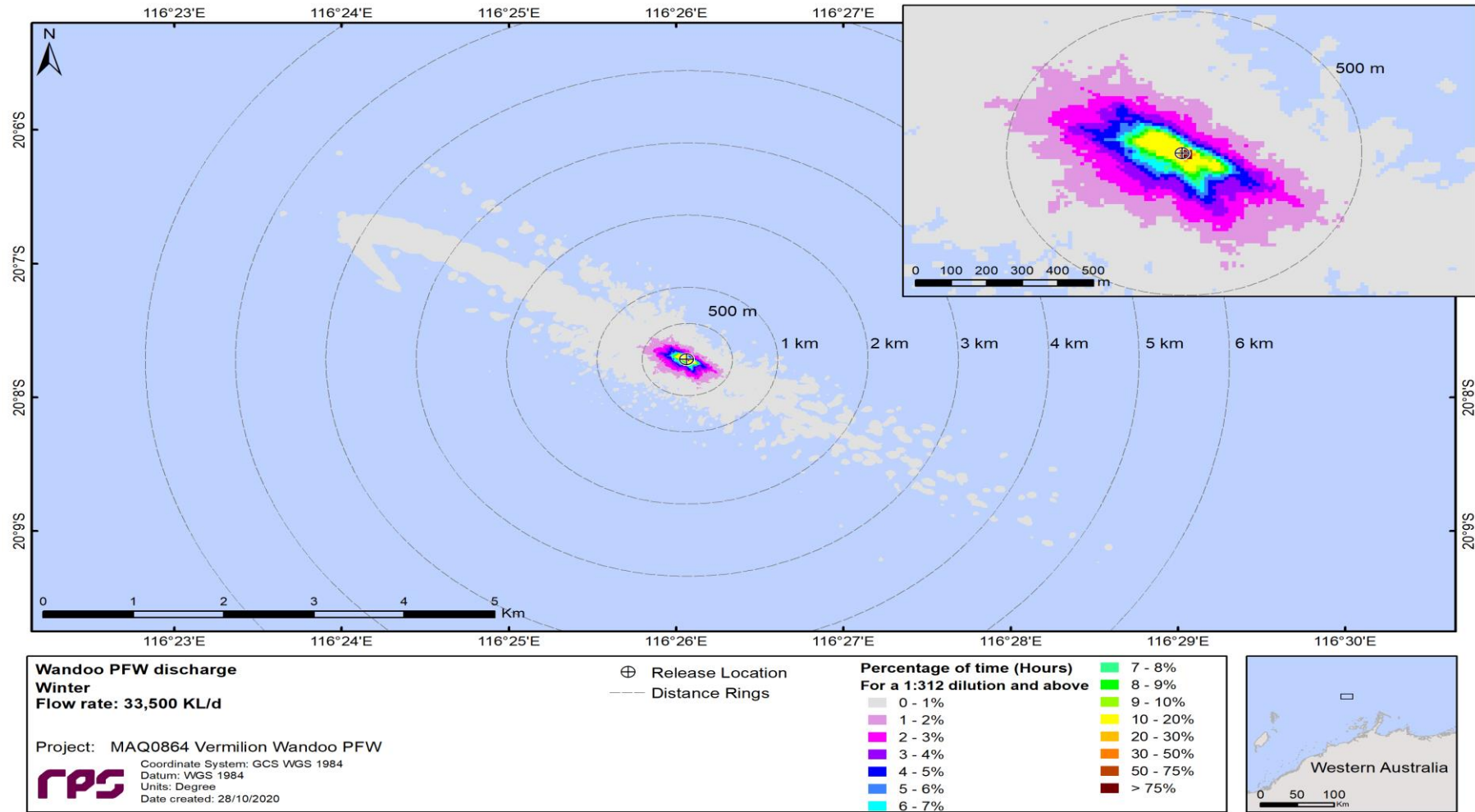
Figure 2-17 Spatial plots of percentage of time (hours) the PFW stream concentration occurred at, or below, equivalent dilution of 1:312 for the whole PFW stream. Modelling based on a flow rate of 33,500 kL/d during winter(July) conditions
