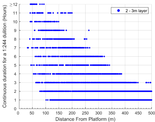
Figure 2-12 Scatter plots presenting the maximum continuous hours the PFW stream concentration occurred at, or below, equivalent dilution of 1:244 for the whole PFW stream. Modelling based on a flow rate of 33,500 kL/d during winter (July) conditions for the 0 – 1m (top plot), 1 – 2m (middle plot) and 2 – 3m depth layers (bottom plot)
