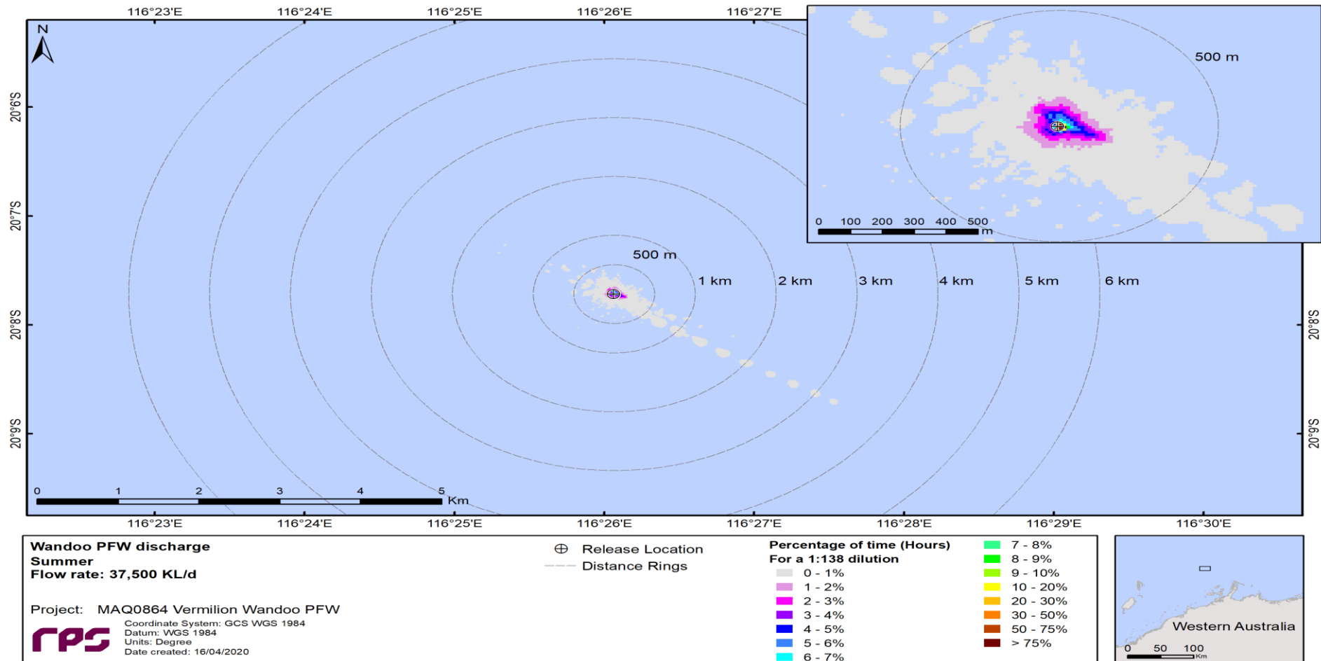
Figure 2-7 Spatial plots of percentage of time (hours) the PFW stream concentration occurred at, or below, equivalent dilution of 1:138 for the whole PFW stream. Modelling based on a flow rate of 37,500 kL/d during summer (January) conditions .
