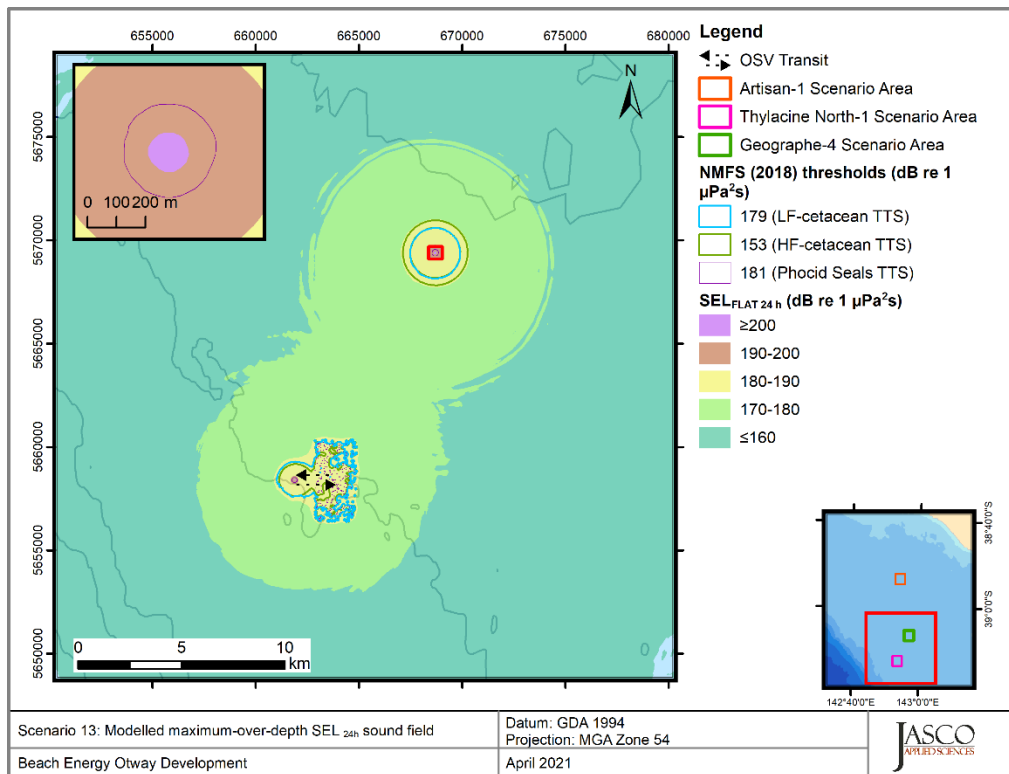
Figure 47. Geographe-4 and Thylacine North-1, Vessel stationary operating at 20% MCR with the MODU under resupply (Scenario 13), SEL 24h : Sound level contour map showing unweighted maximum-over-depth SEL 24h results, along with isopleths for PTS and TTS thresholds. Thresholds for some PTS and TTS were either not reached or were too short to be displayed on a map. Refer to the radii tables in Section 4.1 for distances.
