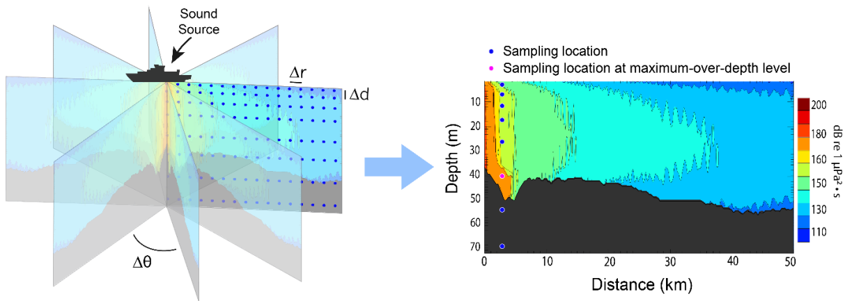
Figure B-4. The Nx2-D and maximum-over-depth modelling approach used by MONM.
