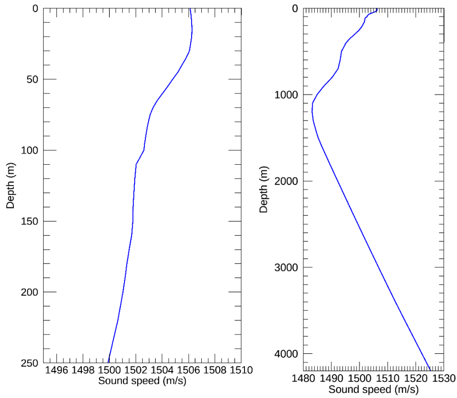
Figure B-3. The modelling sound speed profile corresponding to November: Top 250 m (left) and full profile (right) Profiles are calculated from temperature and salinity profiles from Generalized Digital Environmental Model V 3.0 (GDEM; Teague et al. 1990, Carnes 2009).
