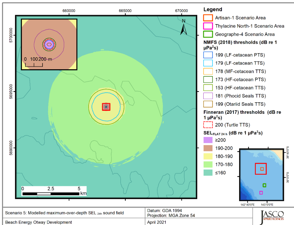
Figure 40. Artisan-1, Vessel stationary operating at 20% MCR (Scenario 5), SEL 24h : Sound level contour map showing unweighted maximum-over-depth SEL 24h results, along with isopleths for PTS and TTS thresholds. Thresholds for some PTS and TTS were either not reached or were too short to be displayed on a map. Refer to the radii tables in Section 4.1 for distances.
