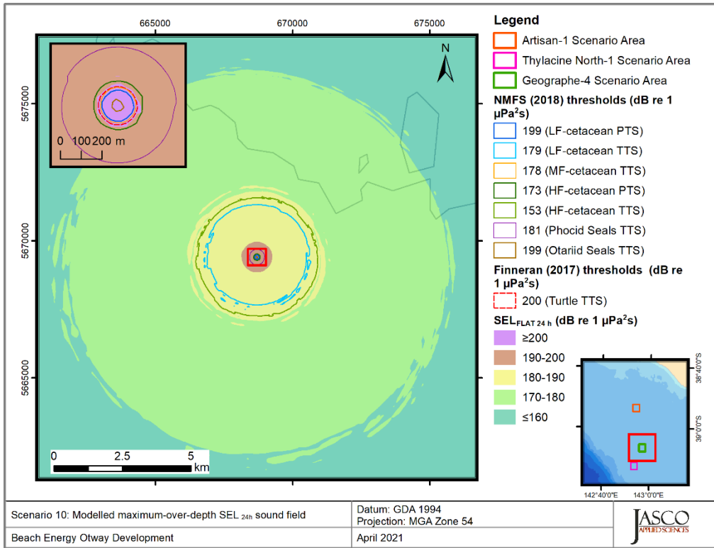
Figure 45. Geographe-4, Vessel stationary operating at 40% MCR (Scenario 10), SEL 24h : Sound level contour map showing unweighted maximum-over-depth SEL 24h results, along with isopleths for PTS and TTS thresholds. Thresholds for some PTS and TTS were either not reached or were too short to be displayed on a map. Refer to the radii tables in Section 4.1 for distances.
