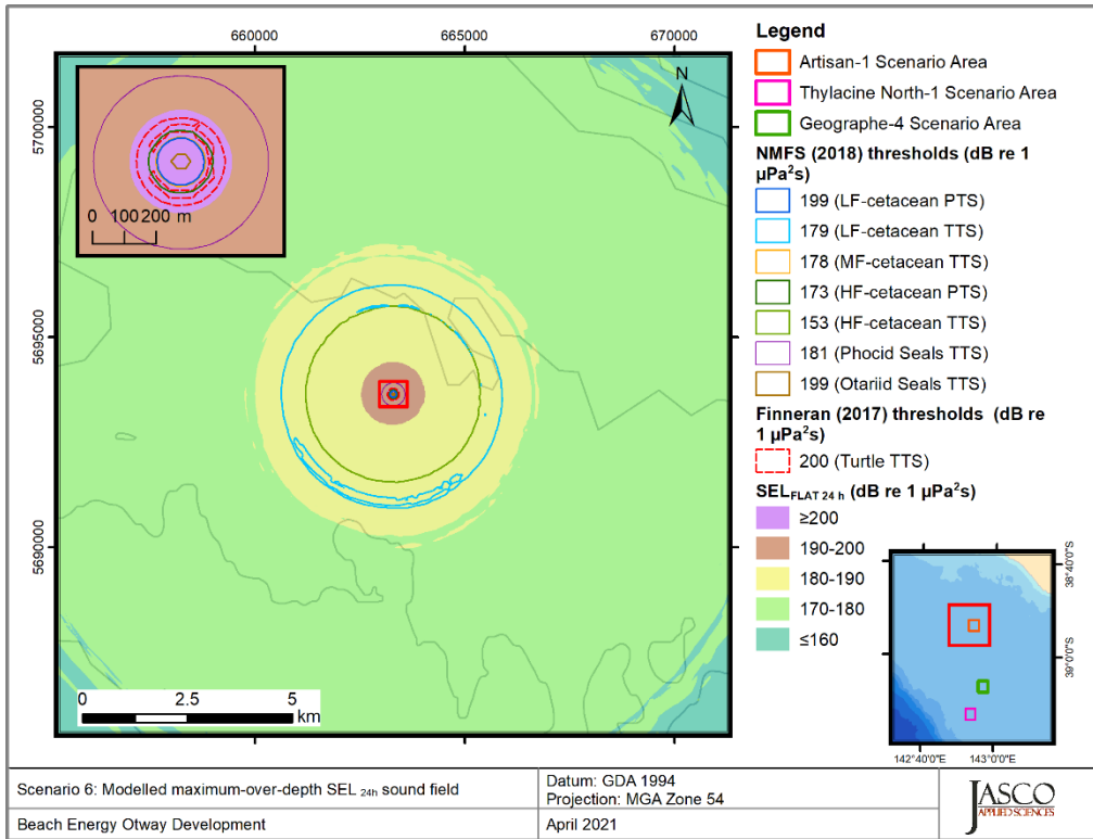
Figure 19. Artisan-1, Vessel stationary operating at 40% MCR (Scenario 6), SEL 24h : Sound level contour map showing unweighted maximum-over-depth SEL 24h results, along with isopleths for PTS and TTS thresholds. Thresholds for some PTS and TTS were either not reached or were too short to be displayed on a map. Refer to the radii tables in Section 4.1 for distances.
