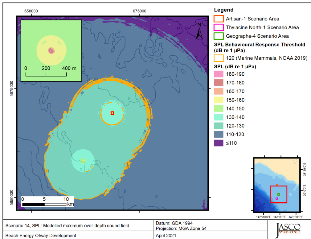
Figure 13. Geographe-4 and Thylacine North-1, Vessel stationary operating at 40% MCR with the MODU under resupply (Scenario 14), SPL: SPL: Sound level contour map, showing unweighted maximum-over-depth SPL results.
