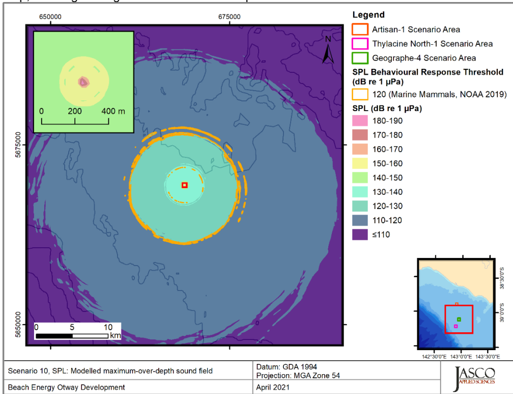
Figure 32. Geographe-4, Vessel stationary operating at 40% MCR (Scenario 10), SPL: SPL: Sound level contour map, showing unweighted maximum-over-depth SPL results.
