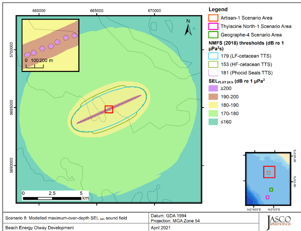
Figure 43. Artisan-1, Vessel laying pipe, operating at 40% MCR (Scenario 8), SEL 24h : Sound level contour map showing unweighted maximum-over-depth SEL 24h results, along with isopleths for PTS and TTS thresholds. Thresholds for some PTS and TTS were either not reached or were too short to be displayed on a map. Refer to the radii tables in Section 4.1 for distances.
