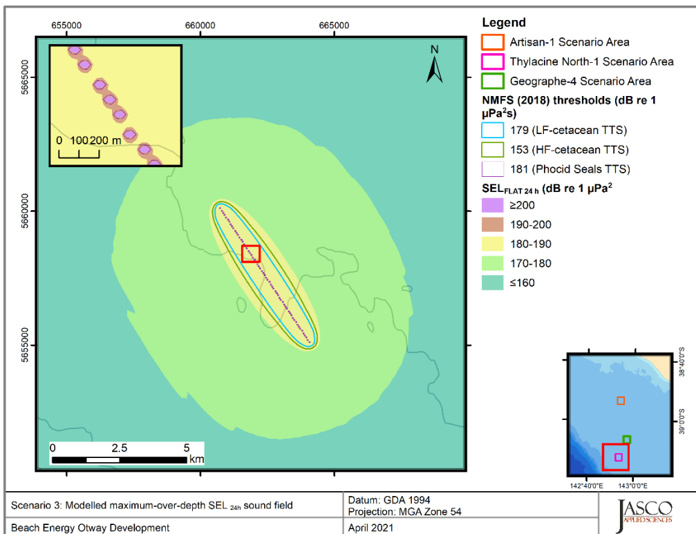
Figure 38. Thylacine North-1, Vessel laying pipe, operating at 20% MCR (Scenario 3), SEL 24h : Sound level contour map showing unweighted maximum-over-depth SEL 24h results, along with isopleths for PTS and TTS thresholds. Thresholds for some PTS and TTS were either not reached or were too short to be displayed on a map. Refer to the radii tables in Section 4.1 for distances.
