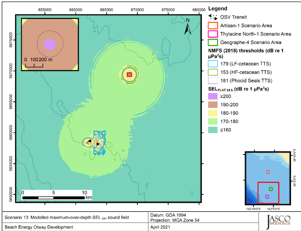
Figure 25. Geographe-4 and Thylacine North-1, Vessel stationary operating at 20% MCR with the MODU under resupply (Scenario 13), SEL 24h : Sound level contour map showing unweighted maximum-over-depth SEL 24h results, along with isopleths for PTS and TTS thresholds. Thresholds for some PTS and TTS were either not reached or were too short to be displayed on a map. Refer to the radii tables in Section 4.1 for distances.
