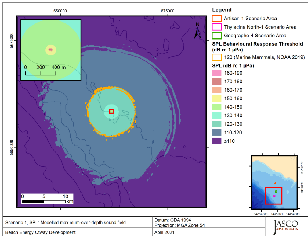
Figure 27. Thylacine North-1, Vessel stationary operating at 20% MCR (Scenarios 1 and 3), SPL: Sound level contour map, showing unweighted maximum-over-depth SPL results.
