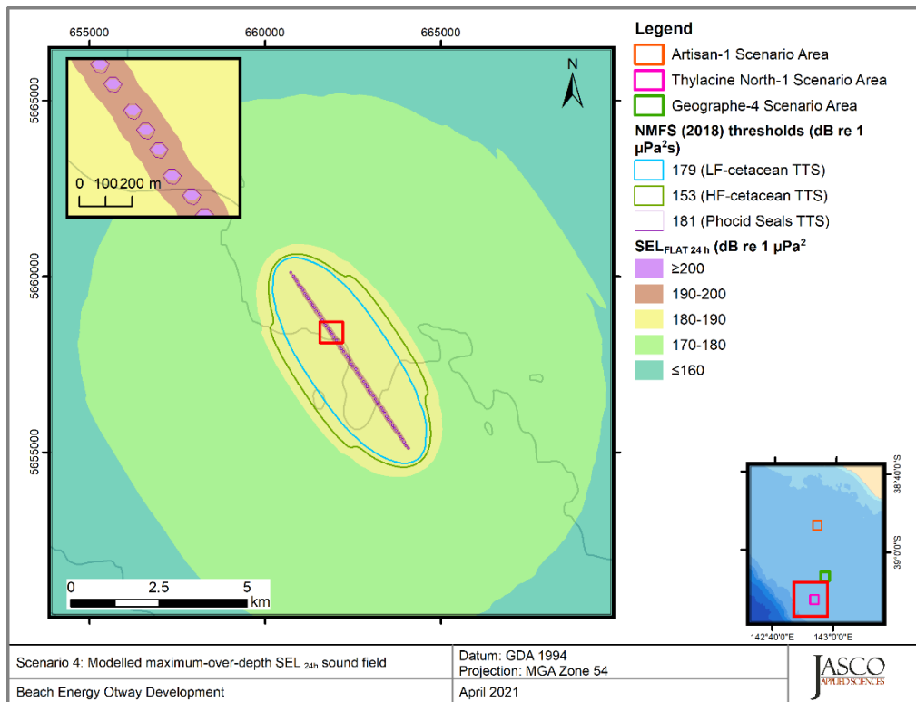
Figure 39. Thylacine North-1, Vessel laying pipe, operating at 40% MCR (Scenario 4), SEL 24h : Sound level contour map showing unweighted maximum-over-depth SEL 24h results, along with isopleths for PTS and TTS thresholds. Thresholds for some PTS and TTS were either not reached or were too short to be displayed on a map. Refer to the radii tables in Section 4.1 for distances.
