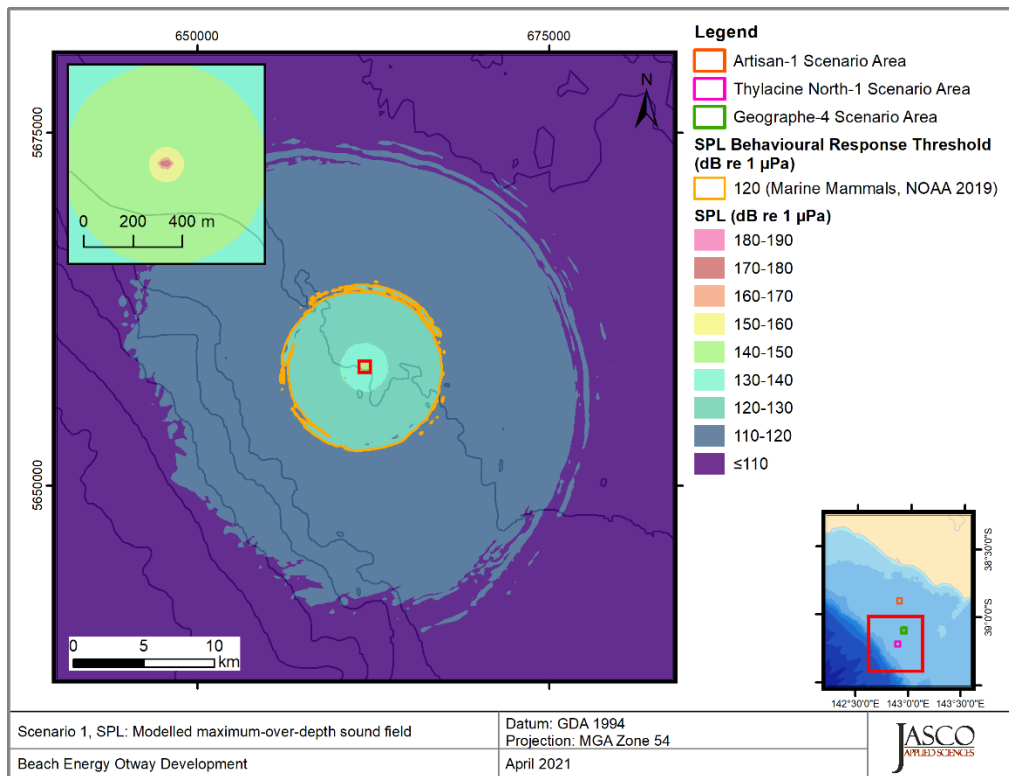
Figure 5. Thylacine North-1, Vessel stationary operating at 20% MCR (Scenarios 1 and 3), SPL: Sound level contour map, showing unweighted maximum-over-depth SPL results.
