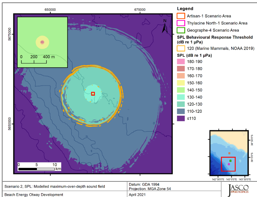
Figure 28. Thylacine North-1, Vessel stationary operating at 40% MCR (Scenarios 2 and 4), SPL: SPL: Sound level contour map, showing unweighted maximum-over-depth SPL results.
