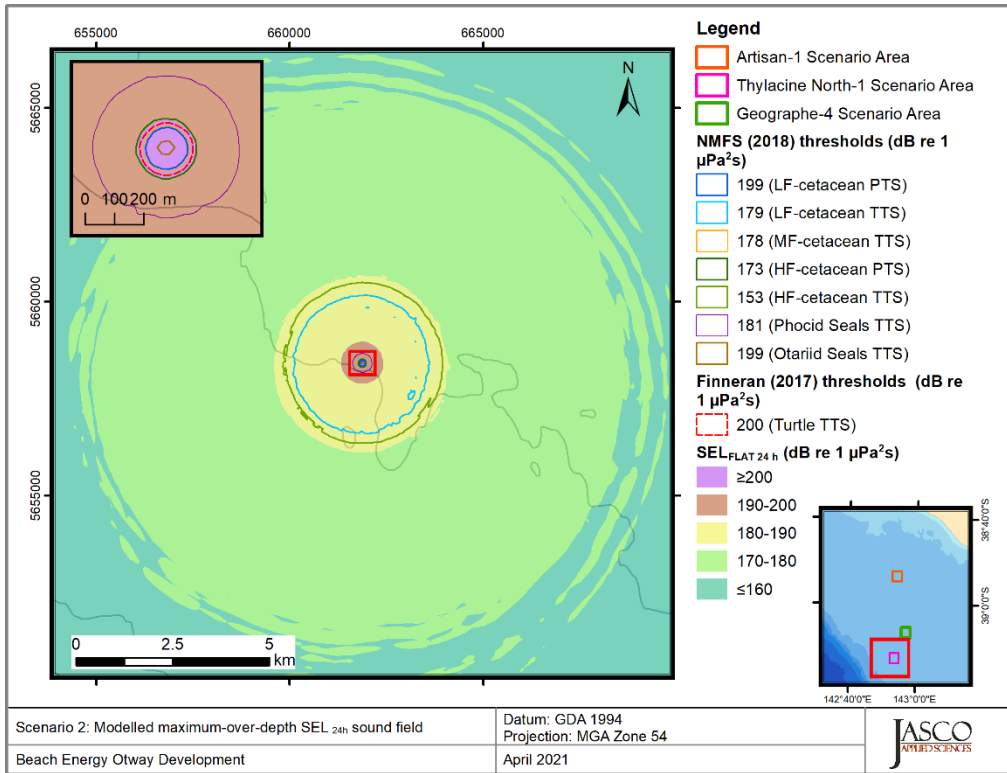
Figure 15. Thylacine North-1, Vessel stationary operating at 40% MCR (Scenario 2), SEL 24h : Sound level contour map showing unweighted maximum-over-depth SEL 24h results, along with isopleths for PTS and TTS thresholds. Thresholds for some PTS and TTS were either not reached or were too short to be displayed on a map. Refer to the radii tables in Section 4.1 for distances.
