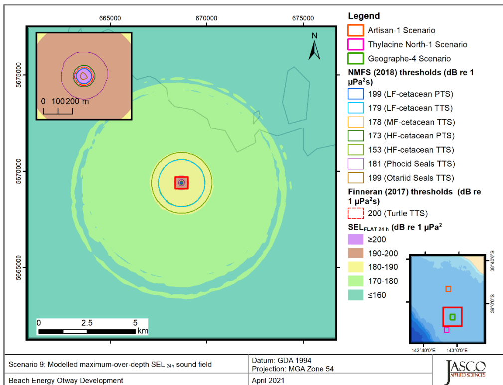
Figure 44. Geographe-4, Vessel stationary operating at 20% MCR (Scenario 9), SEL 24h : Sound level contour map showing unweighted maximum-over-depth SEL 24h results, along with isopleths for PTS and TTS thresholds. Thresholds for some PTS and TTS were either not reached or were too short to be displayed on a map. Refer to the radii tables in Section 4.1 for distances.
