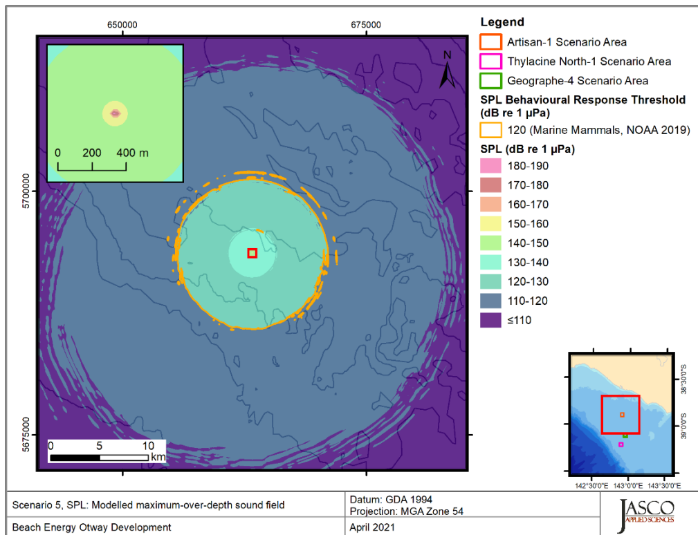
Figure 7. Artisan-1, Vessel stationary operating at 20% MCR (Scenarios 5 and 7), SPL: SPL: Sound level contour map, showing unweighted maximum-over-depth SPL results.
