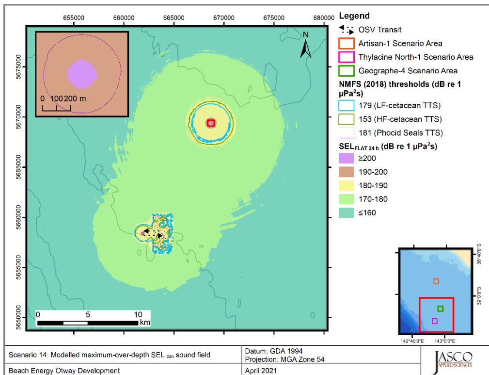
Figure 48. Geographe-4 and Thylacine North-1, Vessel stationary operating at 40% MCR with the MODU under resupply (Scenario 14), SEL 24h : Sound level contour map showing unweighted maximum-over-depth SEL 24h results, along with isopleths for PTS and TTS thresholds. Thresholds for some PTS and TTS were either not reached or were too short to be displayed on a map. Refer to the radii tables in Section 4.1 for distances.
