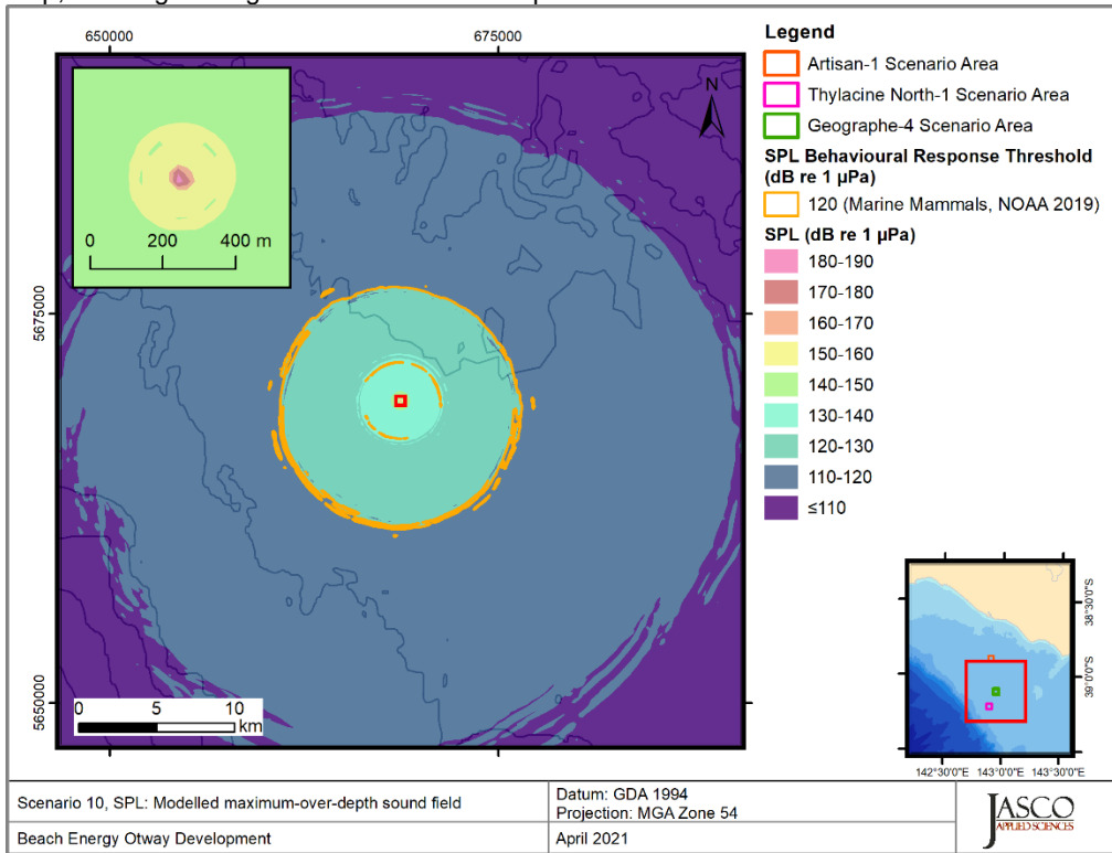
Figure 10. Geographe-4, Vessel stationary operating at 40% MCR (Scenario 10), SPL: SPL: Sound level contour map, showing unweighted maximum-over-depth SPL results.
