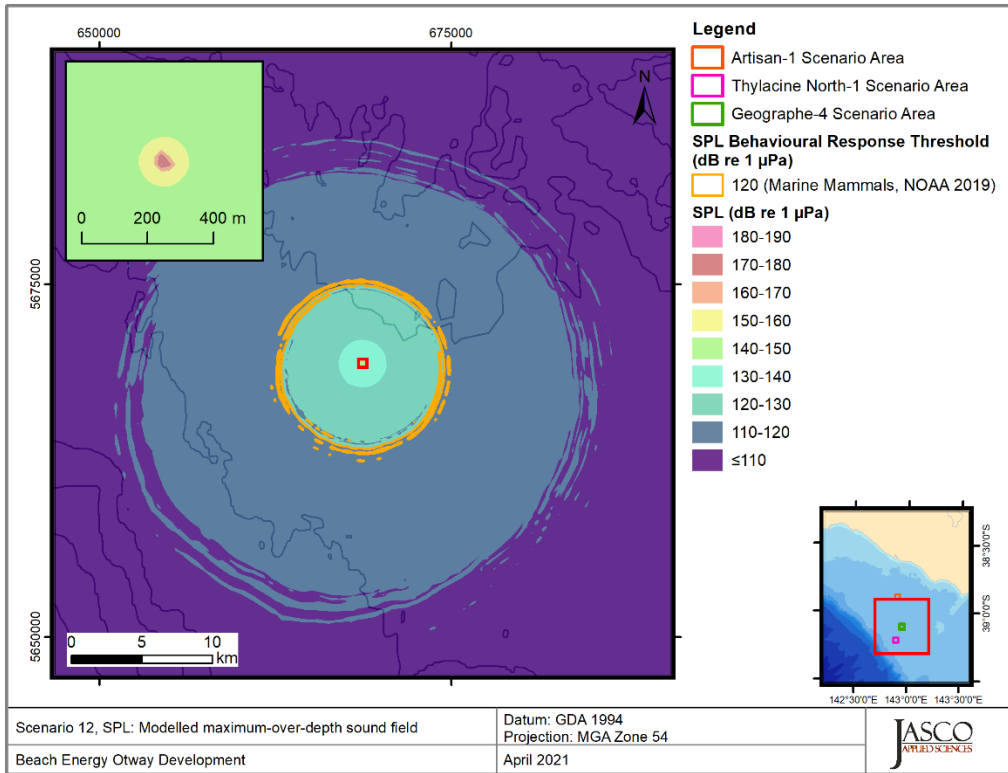
Figure 11. Geographe-4, Vessel stationary operating at 20% MCR and ROV cutter operating (Scenario 12), SPL: SPL: Sound level contour map, showing unweighted maximum-over-depth SPL results.
