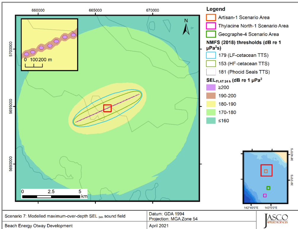
Figure 20. Artisan-1, Vessel laying pipe, operating at 20% MCR (Scenario 7), SEL 24h : Sound level contour map showing unweighted maximum-over-depth SEL 24h results, along with isopleths for PTS and TTS thresholds. Thresholds for some PTS and TTS were either not reached or were too short to be displayed on a map. Refer to the radii tables in Section 4.1 for distances.
