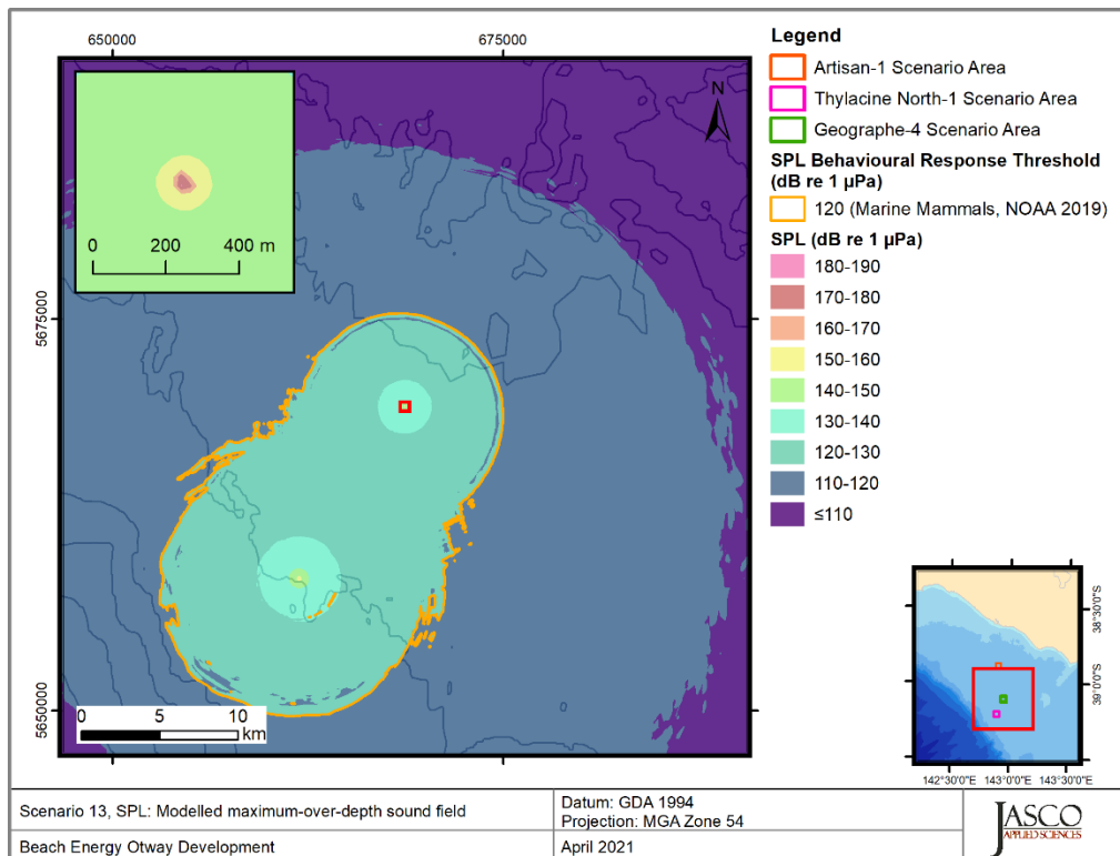
Figure 34. Geographe-4 and Thylacine North-1, Vessel stationary operating at 20% MCR with the MODU under resupply (Scenario 13), SPL: SPL: Sound level contour map, showing unweighted maximum-over-depth SPL results.
