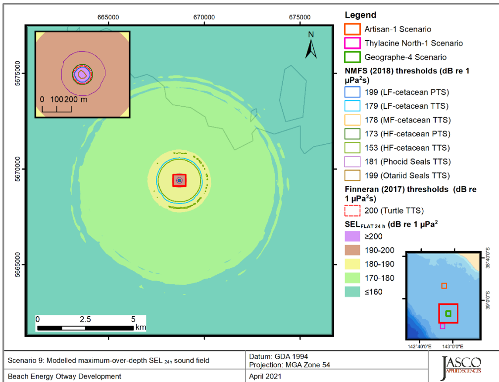
Figure 22. Geographe-4, Vessel stationary operating at 20% MCR (Scenario 9), SEL 24h : Sound level contour map showing unweighted maximum-over-depth SEL 24h results, along with isopleths for PTS and TTS thresholds. Thresholds for some PTS and TTS were either not reached or were too short to be displayed on a map. Refer to the radii tables in Section 4.1 for distances.
