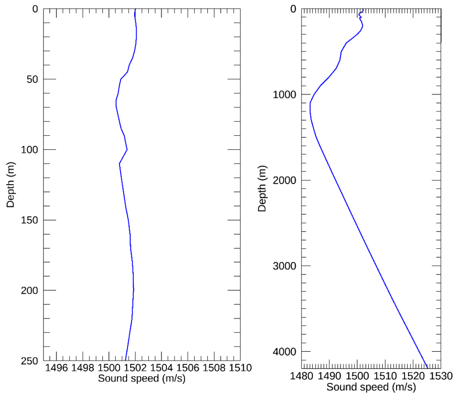
Figure B-2. The modelling sound speed profile corresponding to October: Top 250 m (left) and full profile (right) Profiles are calculated from temperature and salinity profiles from Generalized Digital Environmental Model V 3.0 (GDEM; Teague et al. 1990, Carnes 2009).
