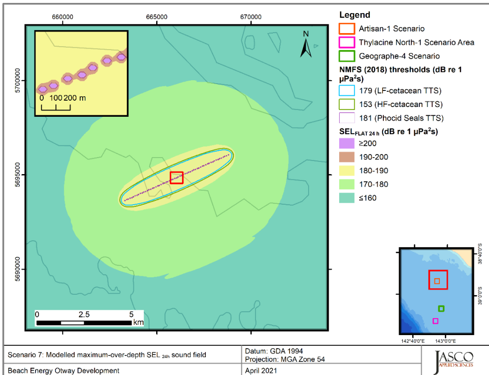
Figure 42. Artisan-1, Vessel laying pipe, operating at 20% MCR (Scenario 7), SEL 24h : Sound level contour map showing unweighted maximum-over-depth SEL 24h results, along with isopleths for PTS and TTS thresholds. Thresholds for some PTS and TTS were either not reached or were too short to be displayed on a map. Refer to the radii tables in Section 4.1 for distances.
