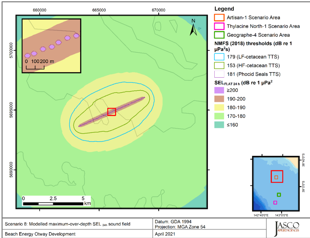
Figure 21. Artisan-1, Vessel laying pipe, operating at 40% MCR (Scenario 8), SEL 24h : Sound level contour map showing unweighted maximum-over-depth SEL 24h results, along with isopleths for PTS and TTS thresholds. Thresholds for some PTS and TTS were either not reached or were too short to be displayed on a map. Refer to the radii tables in Section 4.1 for distances.
