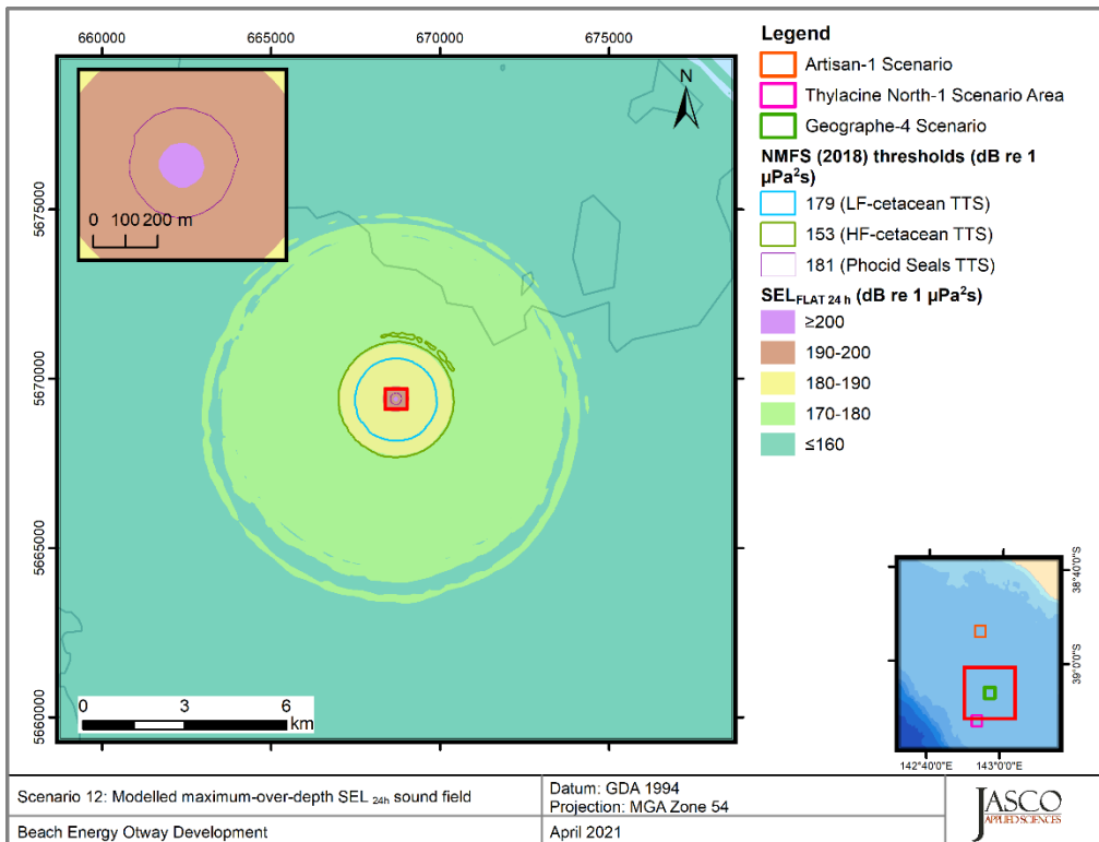
Figure 46. Geographe-4, Vessel stationary operating at 20% MCR and ROV cutter operating (Scenario 12), SEL 24h : Sound level contour map showing unweighted maximum-over-depth SEL 24h results, along with isopleths for PTS and TTS thresholds. Thresholds for some PTS and TTS were either not reached or were too short to be displayed on a map. Refer to the radii tables in Section 4.1 for distances.
