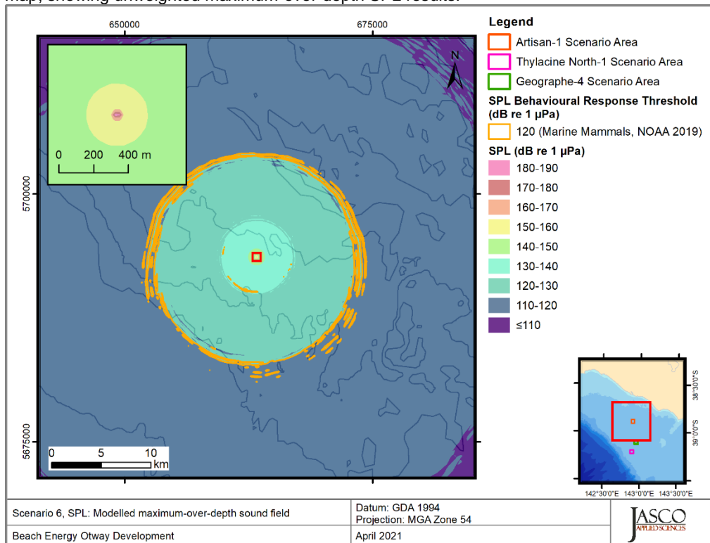
Figure 8. Artisan-1, Vessel stationary operating at 40% MCR (Scenarios 6 and 8), SPL: SPL: Sound level contour map, showing unweighted maximum-over-depth SPL results.
