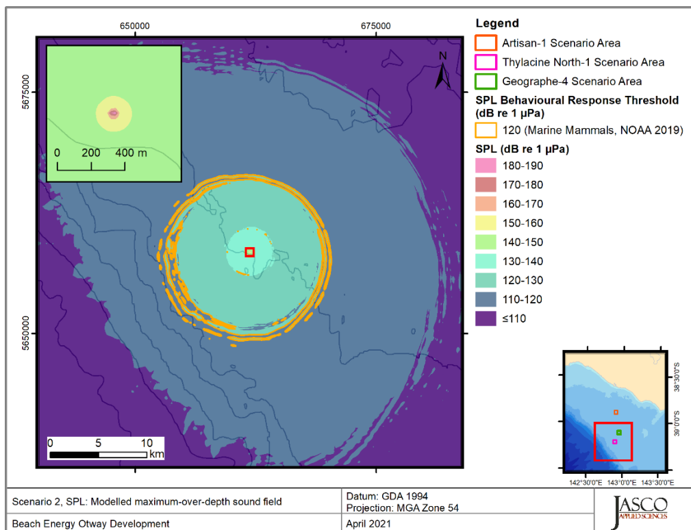
Figure 6. Thylacine North-1, Vessel stationary operating at 40% MCR (Scenarios 2 and 4), SPL: SPL: Sound level contour map, showing unweighted maximum-over-depth SPL results.
