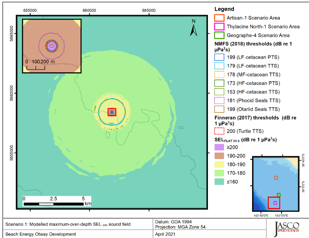
Figure 14. Thylacine North-1, Vessel stationary operating at 20% MCR (Scenario1), SEL 24h : Sound level contour map showing unweighted maximum-over-depth SEL 24h results, along with isopleths for PTS and TTS thresholds. Thresholds for some PTS and TTS were either not reached or were too short to be displayed on a map. Refer to the radii tables in Section 4.1 for distances.
