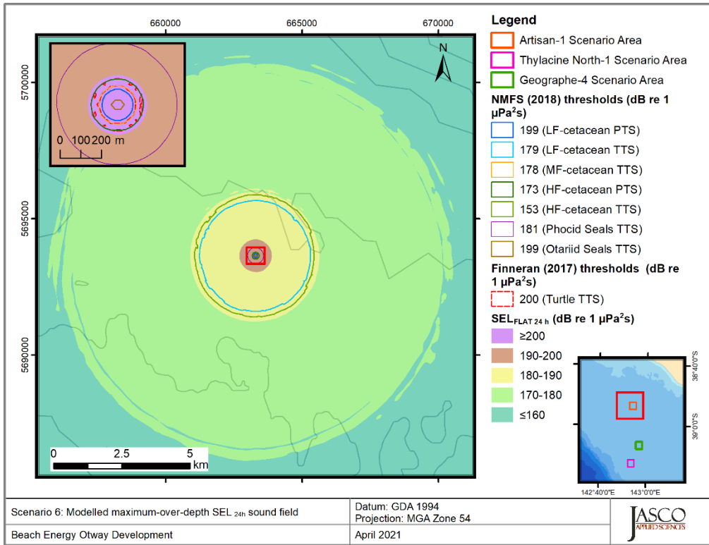
Figure 41. Artisan-1, Vessel stationary operating at 40% MCR (Scenario 6), SEL 24h : Sound level contour map showing unweighted maximum-over-depth SEL 24h results, along with isopleths for PTS and TTS thresholds. Thresholds for some PTS and TTS were either not reached or were too short to be displayed on a map. Refer to the radii tables in Section 4.1 for distances.
