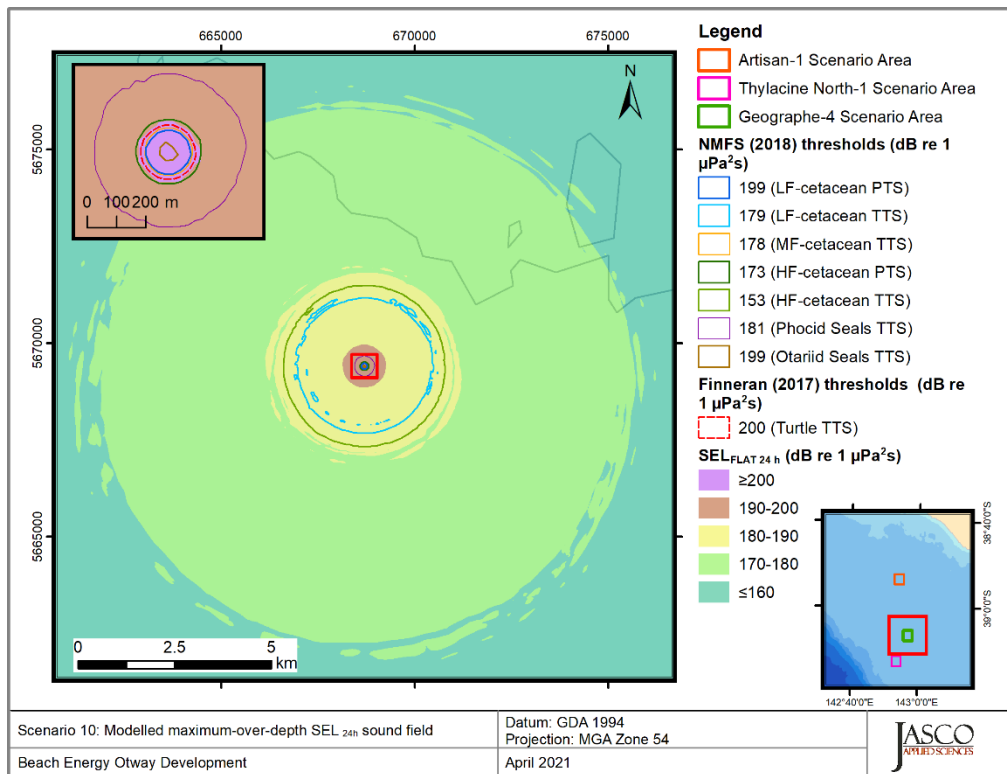
Figure 23. Geographe-4, Vessel stationary operating at 40% MCR (Scenario 10), SEL 24h : Sound level contour map showing unweighted maximum-over-depth SEL 24h results, along with isopleths for PTS and TTS thresholds. Thresholds for some PTS and TTS were either not reached or were too short to be displayed on a map. Refer to the radii tables in Section 4.1 for distances.
