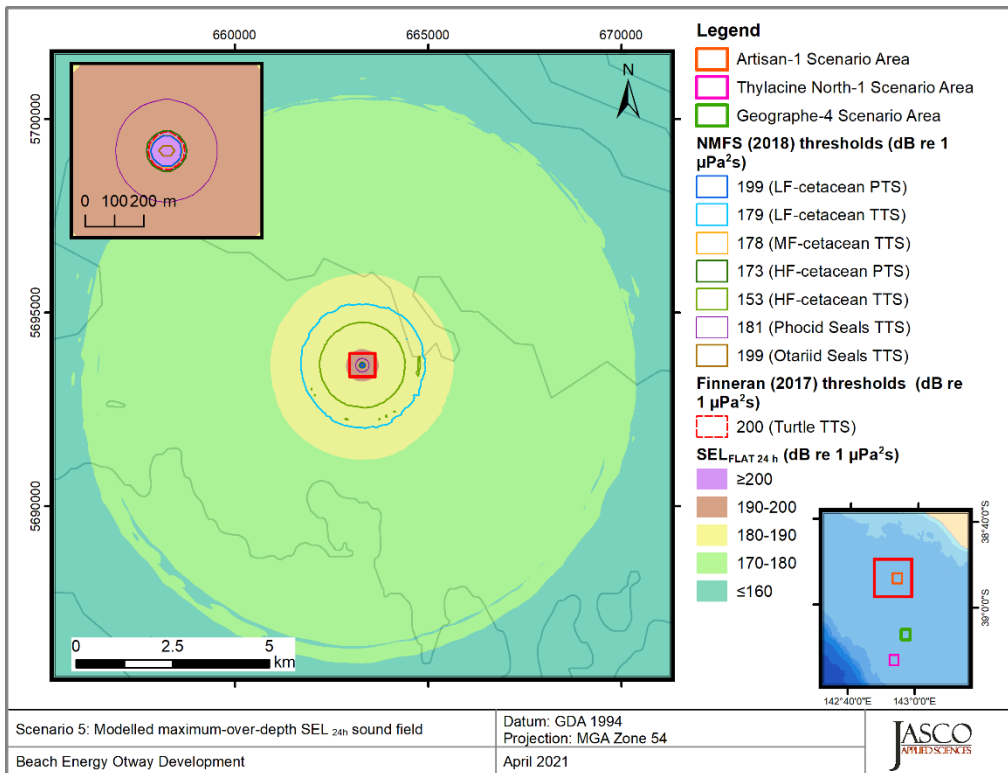
Figure 18. Artisan-1, Vessel stationary operating at 20% MCR (Scenario 5), SEL 24h : Sound level contour map showing unweighted maximum-over-depth SEL 24h results, along with isopleths for PTS and TTS thresholds. Thresholds for some PTS and TTS were either not reached or were too short to be displayed on a map. Refer to the radii tables in Section 4.1 for distances.
