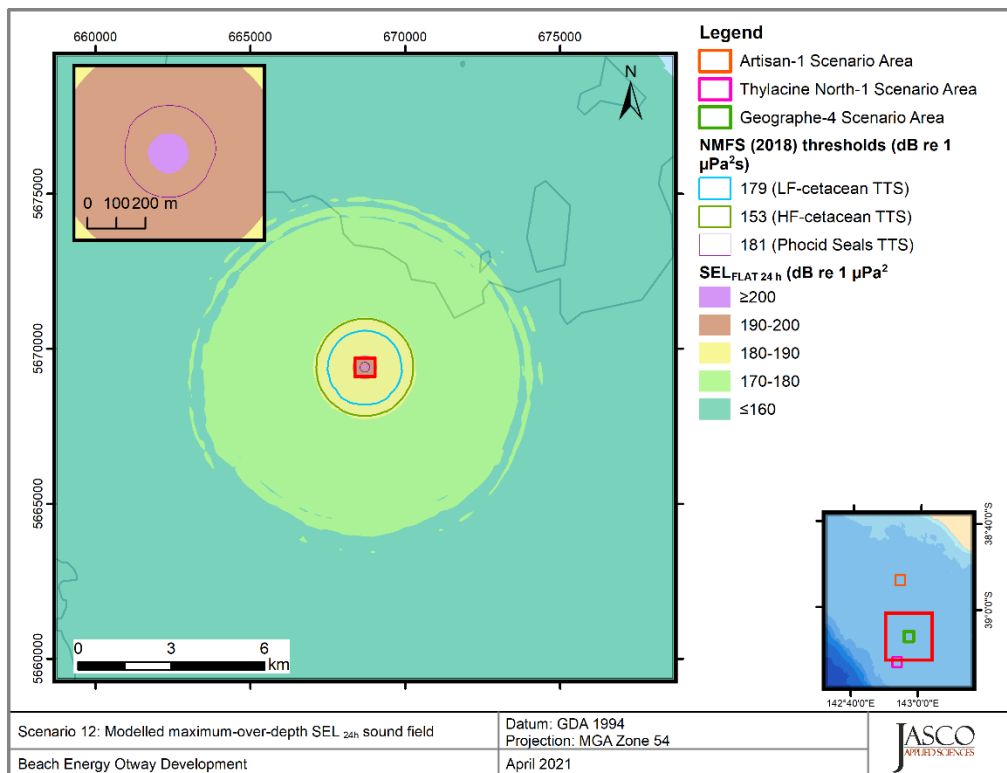
Figure 24. Geographe-4, Vessel stationary operating at 20% MCR and ROV cutter operating (Scenario 12), SEL 24h : Sound level contour map showing unweighted maximum-over-depth SEL 24h results, along with isopleths for PTS and TTS thresholds. Thresholds for some PTS and TTS were either not reached or were too short to be displayed on a map. Refer to the radii tables in Section 4.1 for distances.
