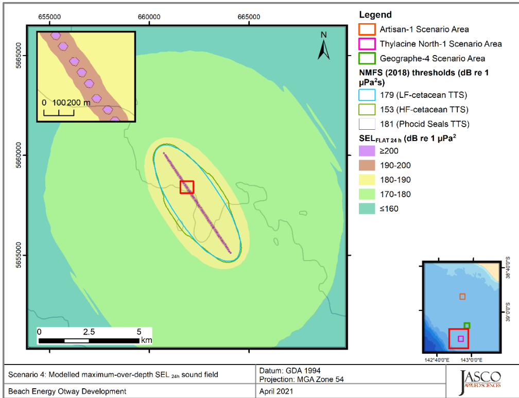
Figure 17. Thylacine North-1, Vessel laying pipe, operating at 40% MCR (Scenario 4), SEL 24h : Sound level contour map showing unweighted maximum-over-depth SEL 24h results, along with isopleths for PTS and TTS thresholds. Thresholds for some PTS and TTS were either not reached or were too short to be displayed on a map. Refer to the radii tables in Section 4.1 for distances.
