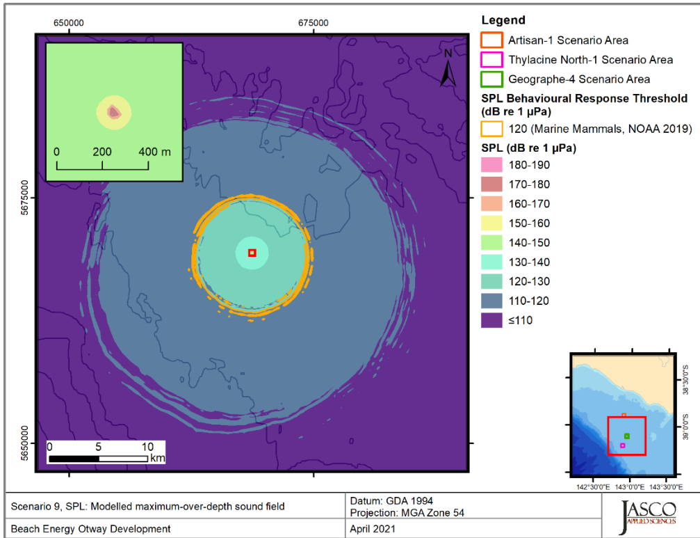
Figure 9. Geographe-4, Vessel stationary operating at 20% MCR (Scenario 9), SPL: SPL: Sound level contour map, showing unweighted maximum-over-depth SPL results.
