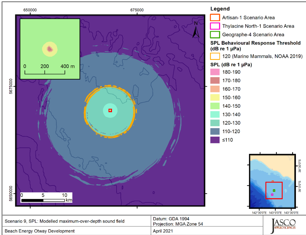
Figure 31. Geographe-4, Vessel stationary operating at 20% MCR (Scenario 9), SPL: SPL: Sound level contour map, showing unweighted maximum-over-depth SPL results.
