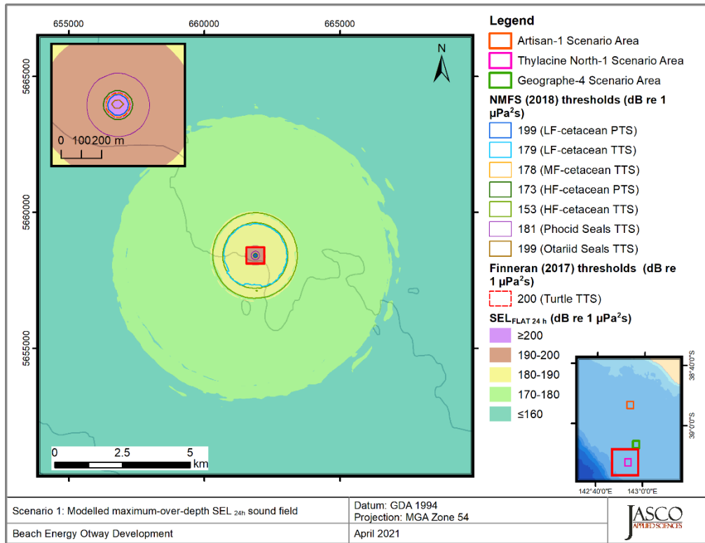
Figure 36. Thylacine North-1, Vessel stationary operating at 20% MCR (Scenario 1), SEL 24h : Sound level contour map showing unweighted maximum-over-depth SEL 24h results, along with isopleths for PTS and TTS thresholds. Thresholds for some PTS and TTS were either not reached or were too short to be displayed on a map. Refer to the radii tables in Section 4.1 for distances.
