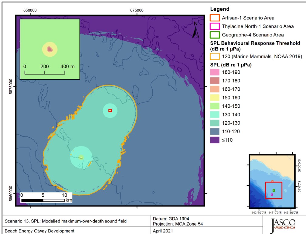
Figure 12. Geographe-4 and Thylacine North-1, Vessel stationary operating at 20% MCR with the MODU under resupply (Scenario 13), SPL: SPL: Sound level contour map, showing unweighted maximum-over-depth SPL results.
