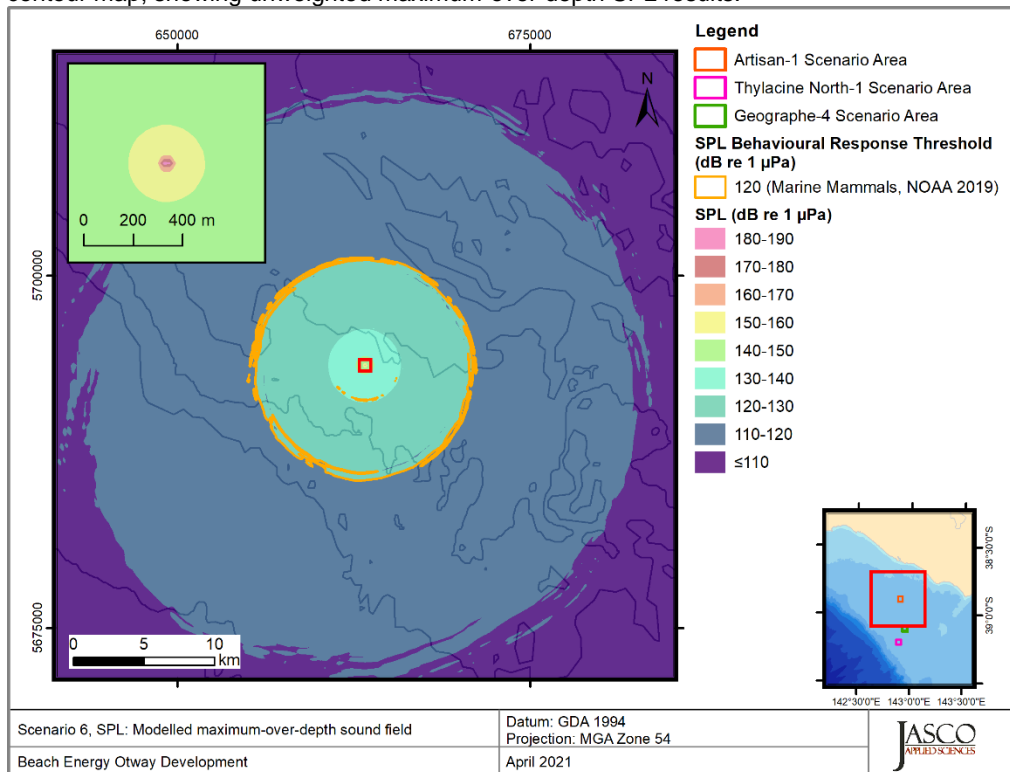
Figure 30. Artisan-1, Vessel stationary operating at 40% MCR (Scenarios 6 and 8), SPL: SPL: Sound level contour map, showing unweighted maximum-over-depth SPL results.
