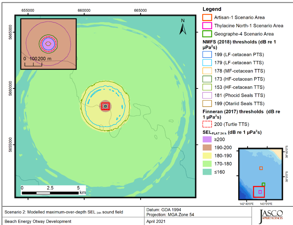
Figure 37. Thylacine North-1, Vessel stationary operating at 40% MCR (Scenario 2), SEL 24h : Sound level contour map showing unweighted maximum-over-depth SEL 24h results, along with isopleths for PTS and TTS thresholds. Thresholds for some PTS and TTS were either not reached or were too short to be displayed on a map. Refer to the radii tables in Section 4.1 for distances.
