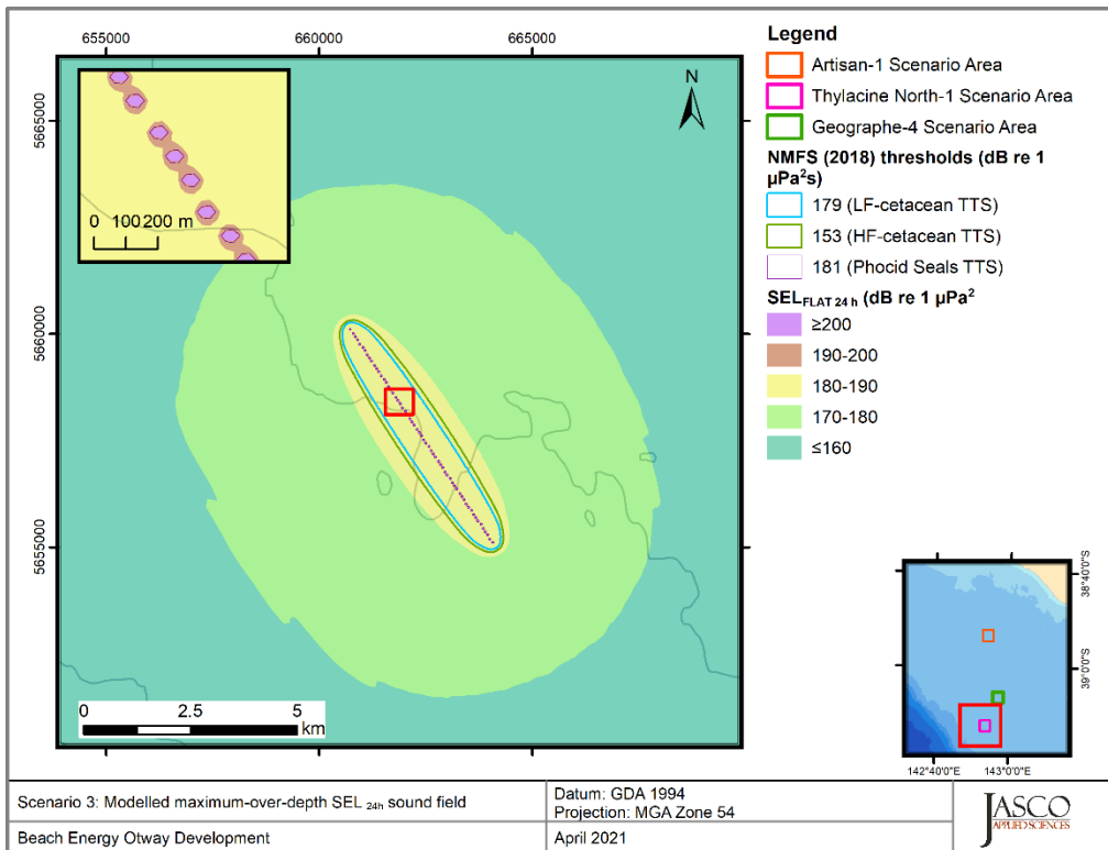
Figure 16. Thylacine North-1, Vessel laying pipe, operating at 20% MCR (Scenario 3), SEL 24h : Sound level contour map showing unweighted maximum-over-depth SEL 24h results, along with isopleths for PTS and TTS thresholds. Thresholds for some PTS and TTS were either not reached or were too short to be displayed on a map. Refer to the radii tables in Section 4.1 for distances.
