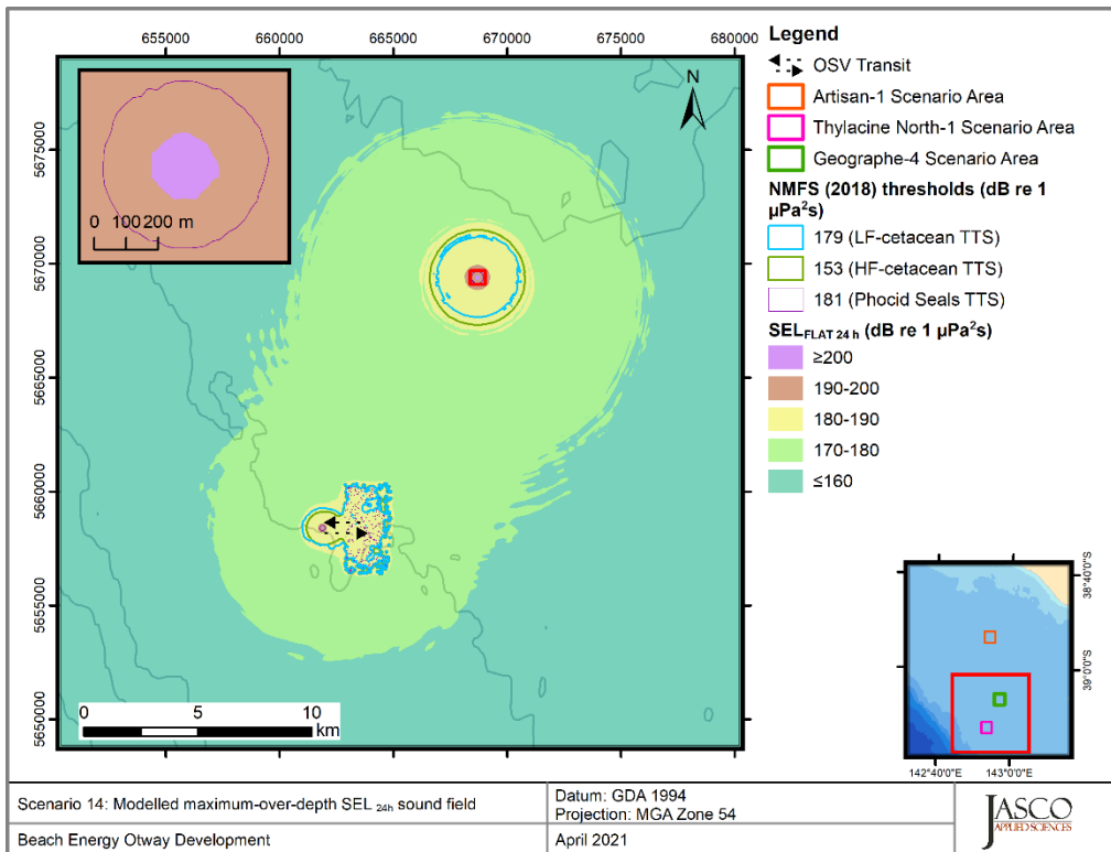
Figure 26. Geographe-4 and Thylacine North-1, Vessel stationary operating at 40% MCR with the MODU under resupply (Scenario 14), SEL 24h : Sound level contour map showing unweighted maximum-over-depth SEL 24h results, along with isopleths for PTS and TTS thresholds. Thresholds for some PTS and TTS were either not reached or were too short to be displayed on a map. Refer to the radii tables in Section 4.1 for distances.
