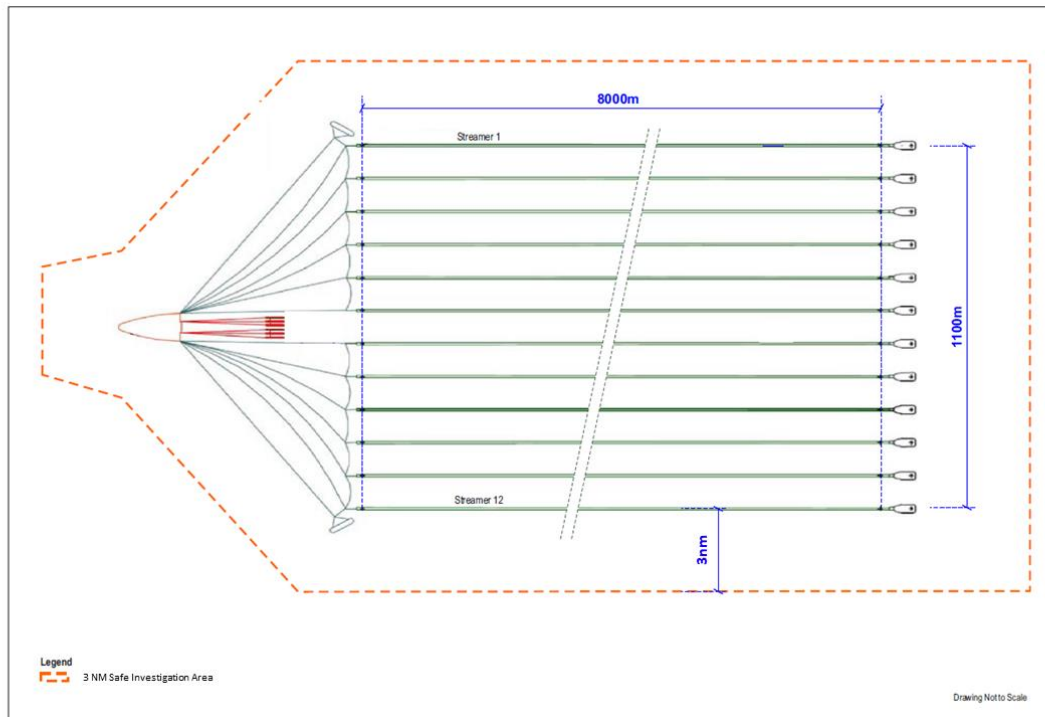
Figure 3-2: Safe Navigation Area surround the seismic vessel and towed arrays (note that streamer lengths and spreads are indicative and may vary)
