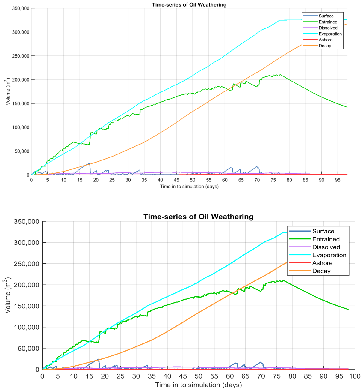
Figure 10.32 Predicted weathering and fates graph for the trajectory with the largest volume of oil ashore for the unmitigated (upper image) and mitigated (lower image) cases. Results are based on a 786,858 m 3 surface release of crude oil over 77 days, tracked for 98 days.
