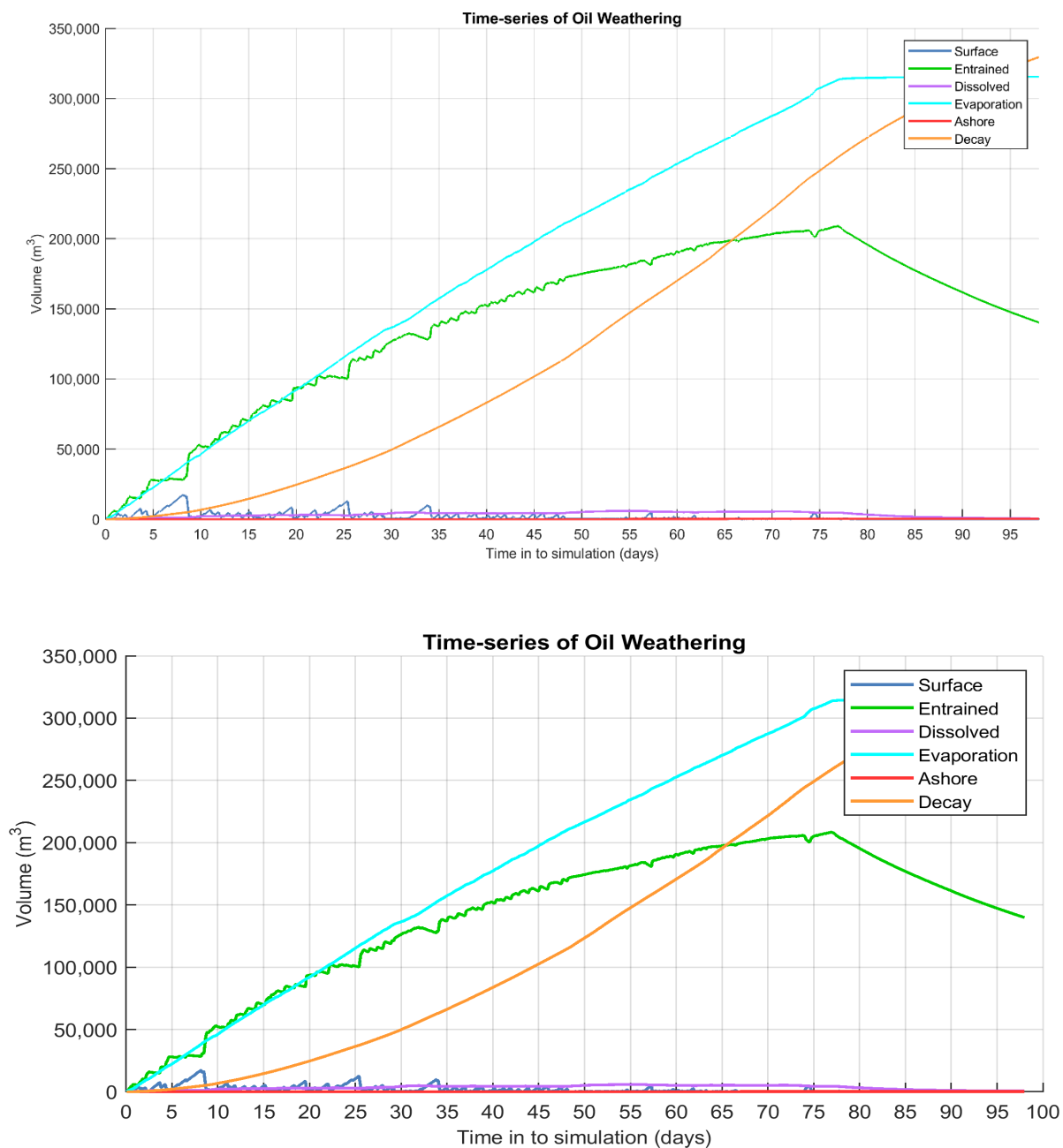
Figure 10.41 Predicted weathering and fates graph for the trajectory with the largest area of dissolved hydrocarbons above 10 ppb for the unmitigated (upper image) and mitigated (lower image) cases. Results are based on a 786,858 m 3 surface release of crude oil over 77 days, tracked for 98 days.
