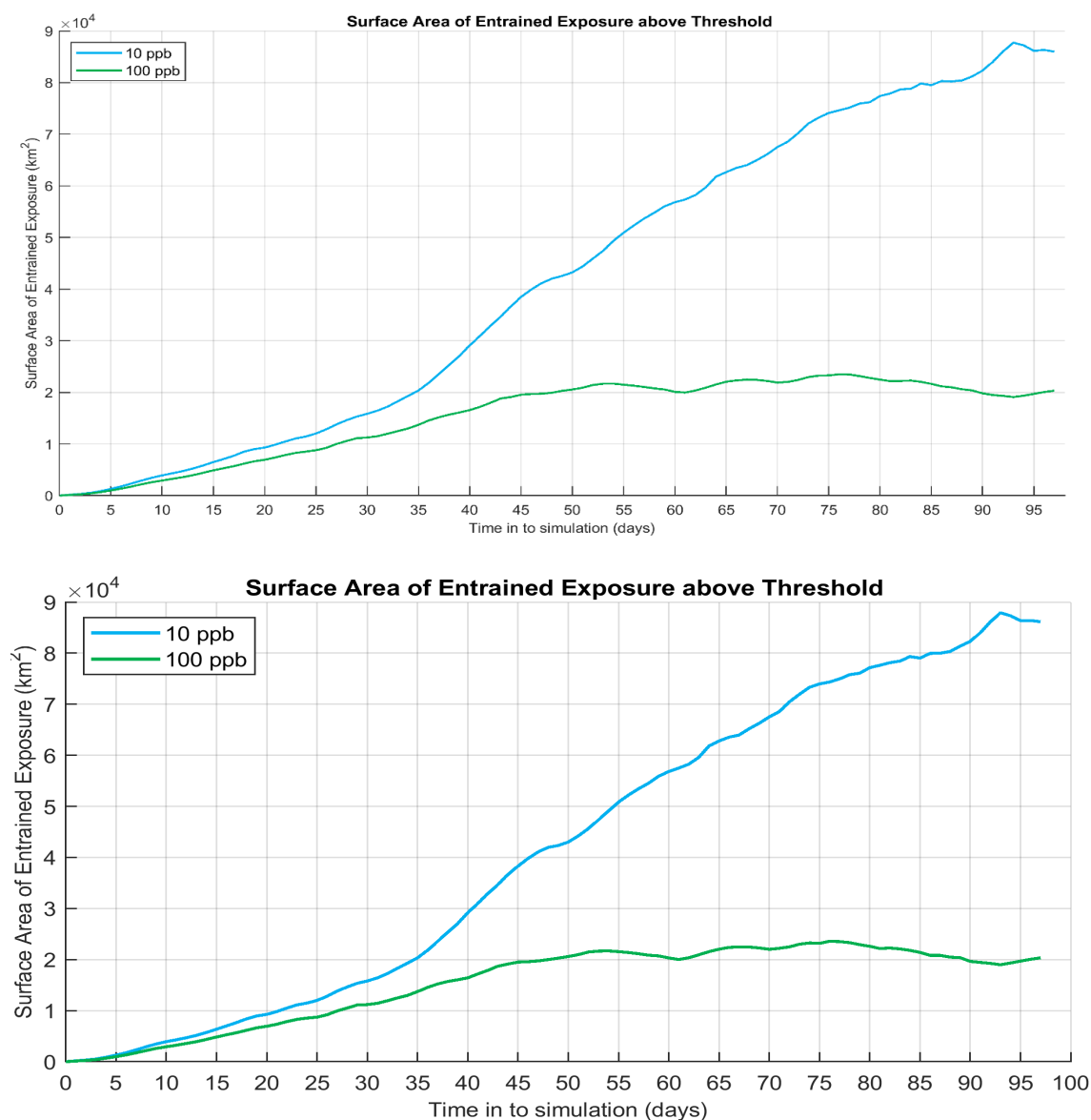
Figure 10.37 Time series of the area of low (10 ppb) and moderate (100 ppb) entrained hydrocarbons for the trajectory with the largest area of entrained hydrocarbons above 10 ppb for the unmitigated (upper image) and mitigated (lower image) cases. Results are based on a 786,858 m 3 surface release of crude oil over 77 days, tracked for 98 days.
