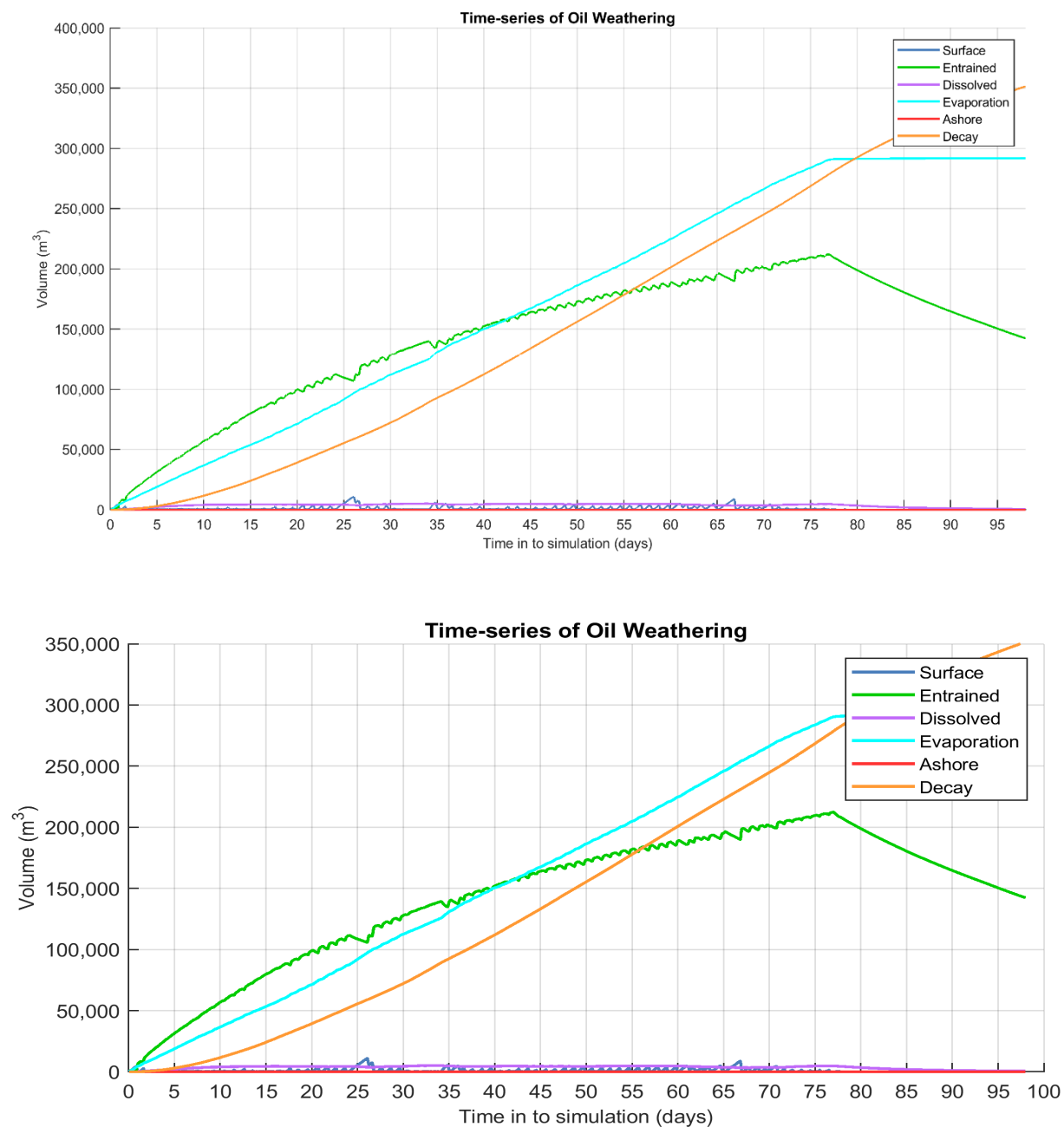
Figure 10.38 Predicted weathering and fates graph for the trajectory with the largest area of entrained hydrocarbons above 10 ppb for the unmitigated (upper image) and mitigated (lower image) cases. Results are based on a 786,858 m 3 surface release of crude oil over 77 days, tracked for 98 days.
