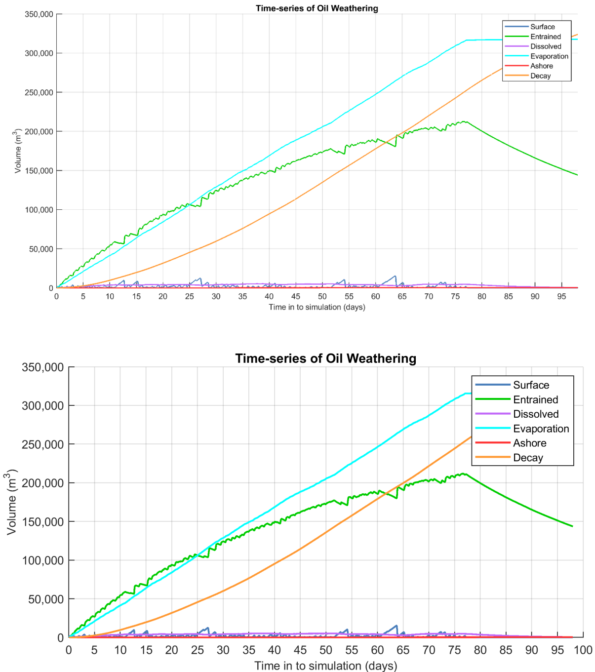
Figure 10.29 Predicted weathering and fates graph for the trajectory with the minimum time before shoreline accumulation above 10 g/m 2 for the unmitigated (upper image) and mitigated (lower image) cases. Results are based on a 786,858 m 3 surface release of crude oil over 77 days, tracked for 98 days.
