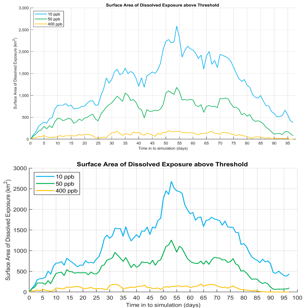
Figure 10.40 Time series of the area of low (10 ppb), moderate (50 ppb) and high (400 ppb) dissolved hydrocarbons for the trajectory with the largest area of dissolved hydrocarbons above 10 ppb for the unmitigated (upper image) and mitigated (lower image) cases. Results are based on a 786,858 m 3 surface release of crude oil over 77 days, tracked for 98 days.
