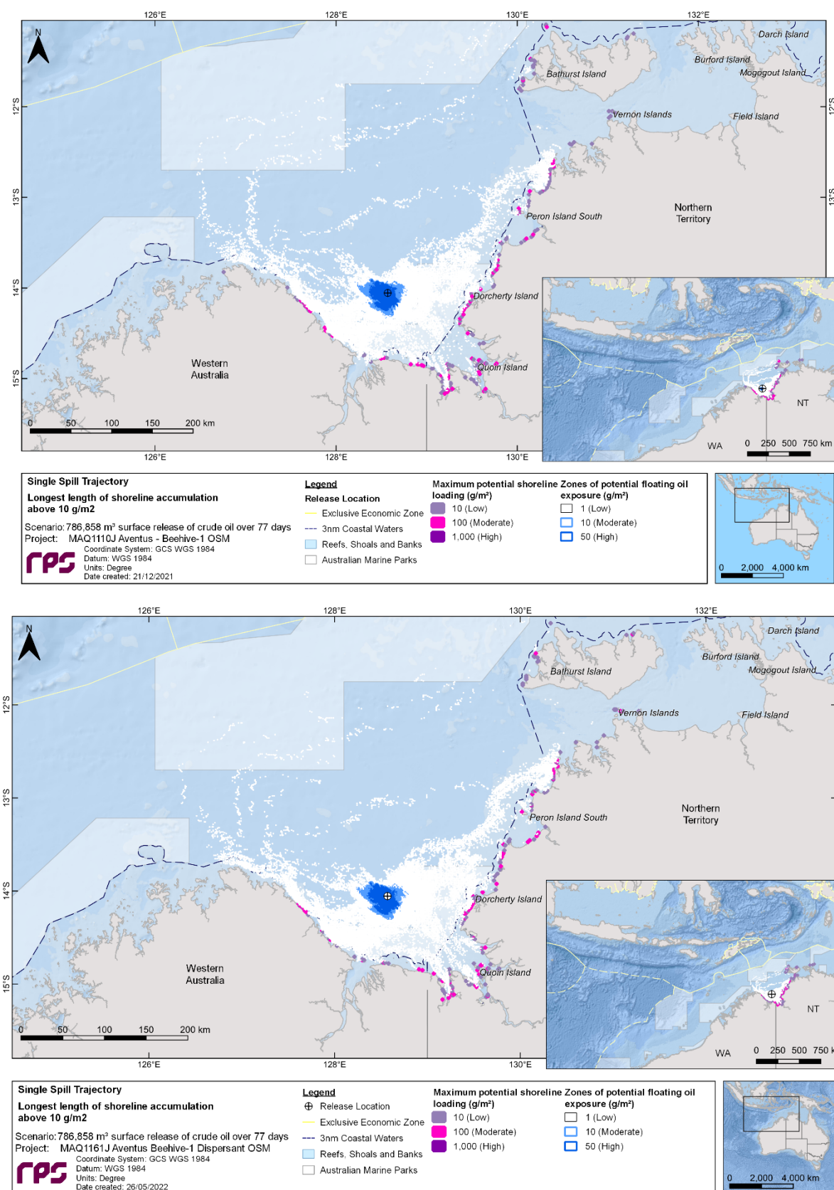
Figure 10.33 Zones of potential floating oil exposure and shoreline accumulation, for the trajectory with the longest length of shoreline accumulation above 10 g/m 2 for the unmitigated (upper image) and mitigated (lower image) cases. Results are based on a 786,858 m 3 surface release of crude oil over 77 days, tracked for 98 days.
