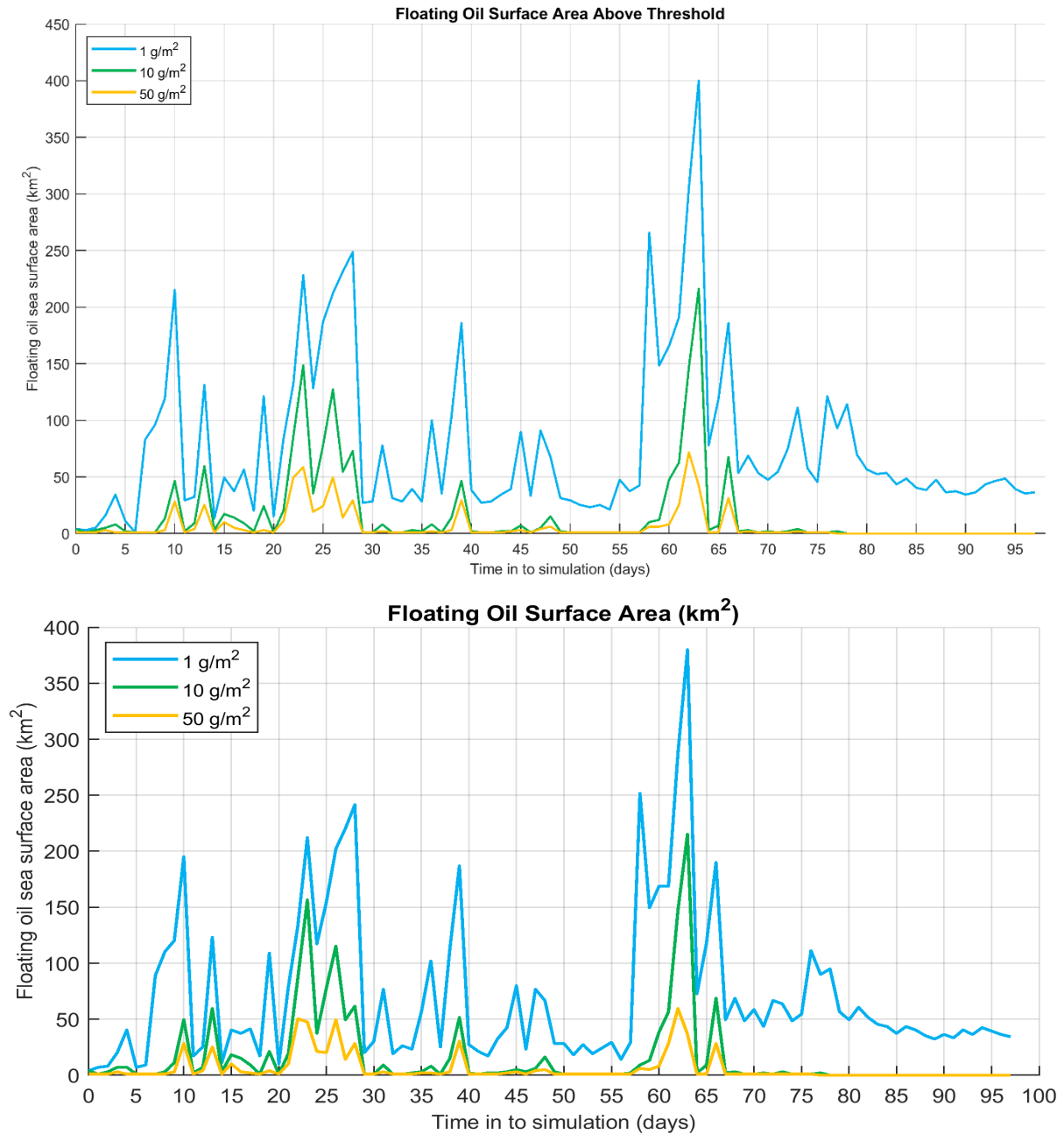
Figure 10.26 Time series of the area of low (1 g/m 2 ), moderate (10 g/m 2 ) and high (50 g/m 2 ) floating oil for the trajectory with the largest swept area of floating oil above 1 g/m 2 for the unmitigated (upper image) and mitigated (lower image) cases. Results are based on a 786,858 m 3 surface release of crude oil over 77 days, tracked for 98 days.
