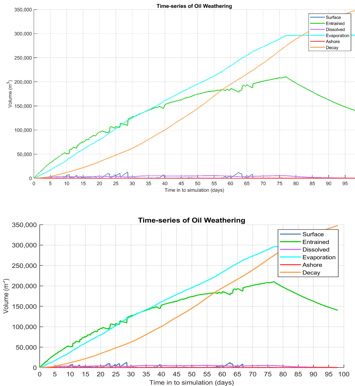
Figure 10.27 Predicted weathering and fates graph for the trajectory with the largest swept area of floating oil above 1 g/m 2 for the unmitigated (upper image) and mitigated (lower image) cases. Results are based on a 786,858 m 3 surface release of crude oil over 77 days, tracked for 98 days.
