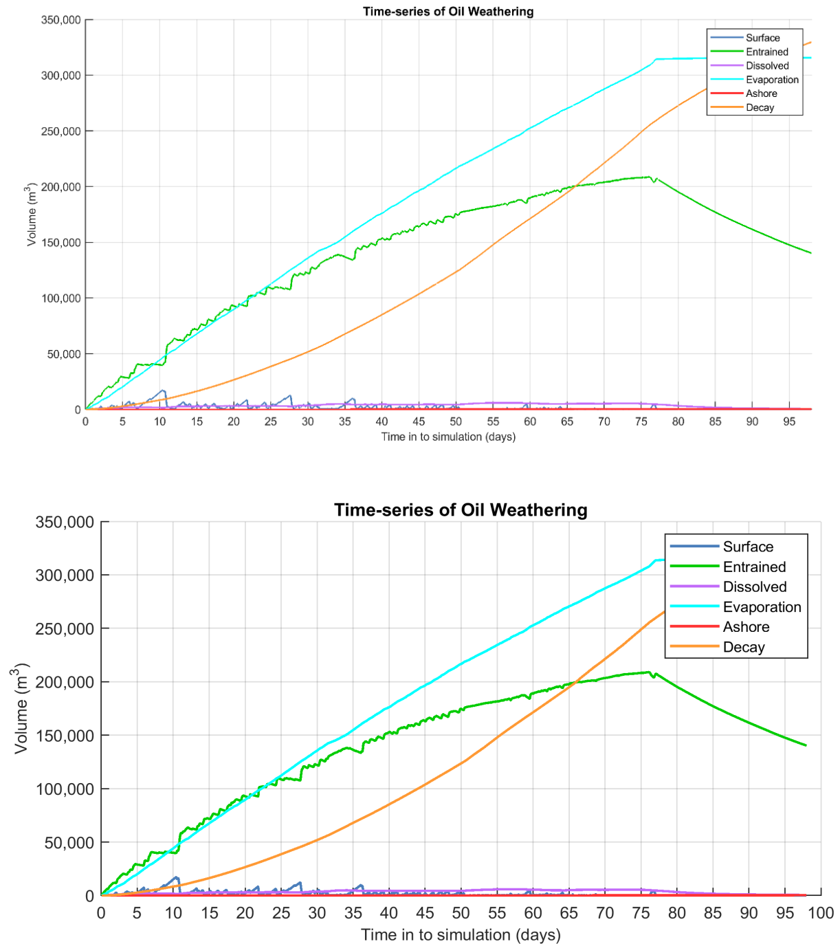
Figure 10.35 Predicted weathering and fates graph for the trajectory with the longest length of shoreline accumulation above 10 g/m 2 for the unmitigated (upper image) and mitigated (lower image) cases. Results are based on a 786,858 m 3 surface release of crude oil over 77 days, tracked for 98 days.
