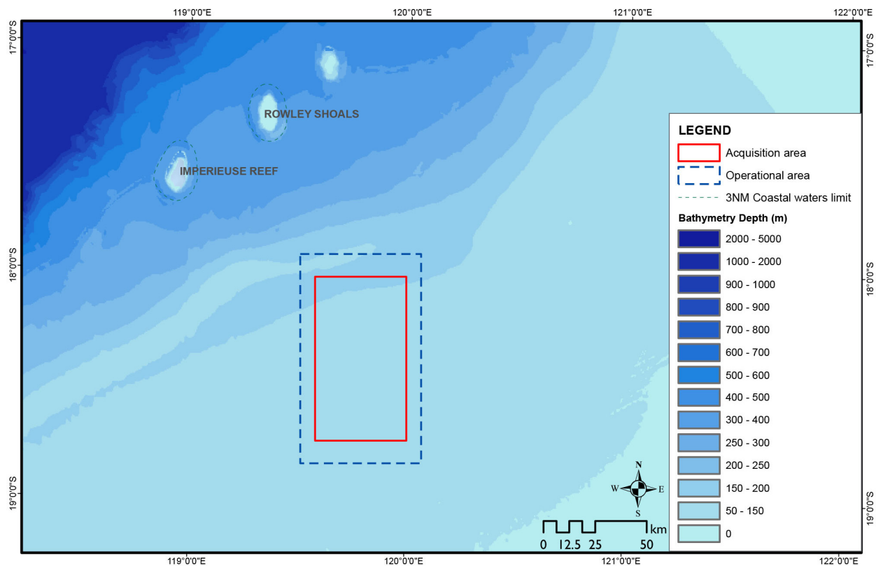
Figure 4-6 – Bathymetry within the Operational Area and Surrounds
