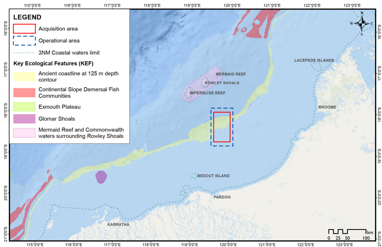
Figure 4-16 – Key Ecological Features
