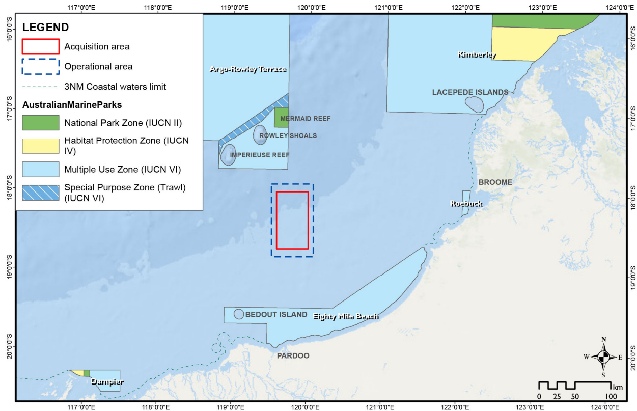
Figure 4-15 – Commonwealth and State Protected Areas
