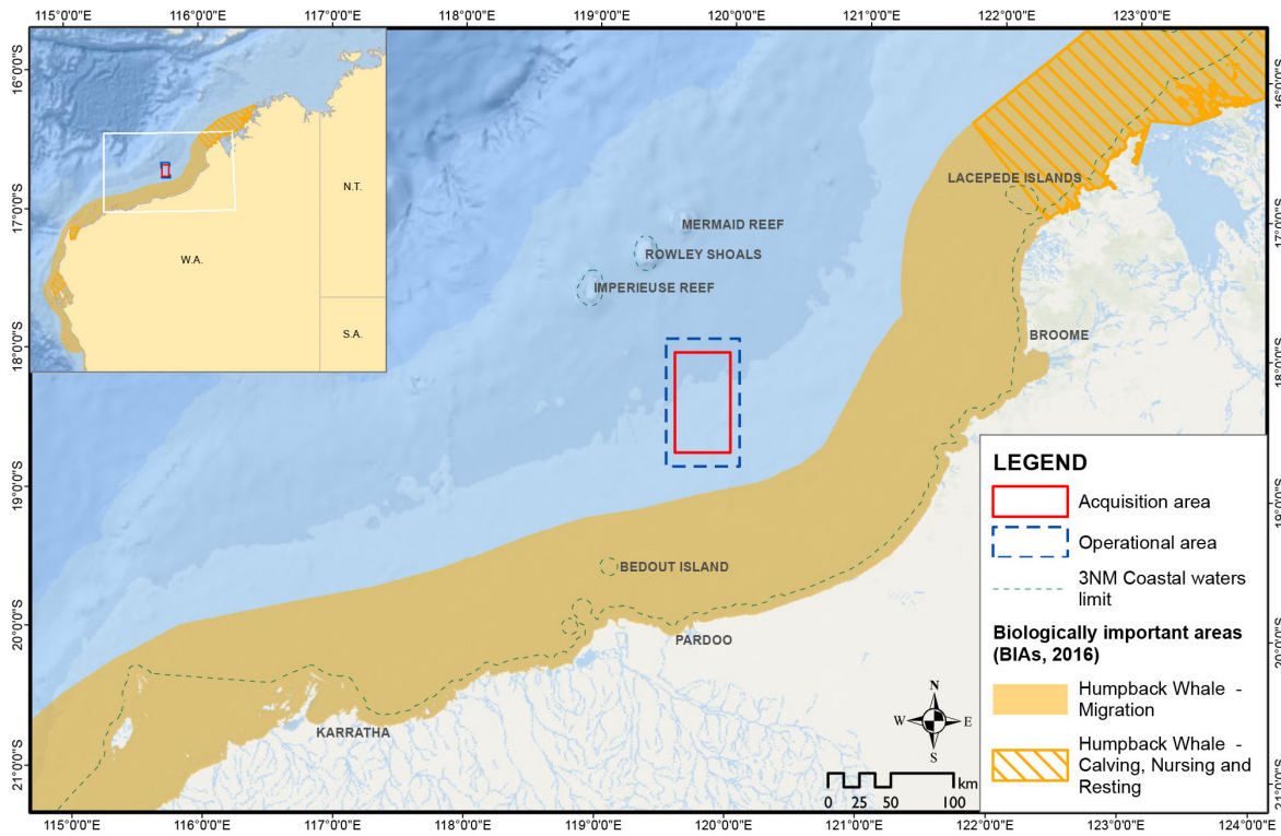
Figure 4-10 – Humpback Whale BIAs
