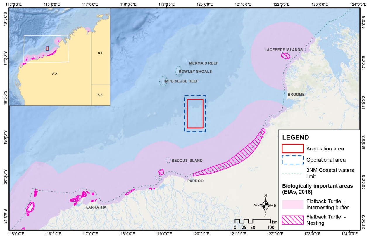
Figure 4-13 – Flatback Turtle BIAs
