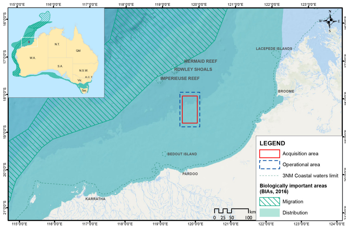
Figure 4-11 – Pygmy Blue Whale BIAs
