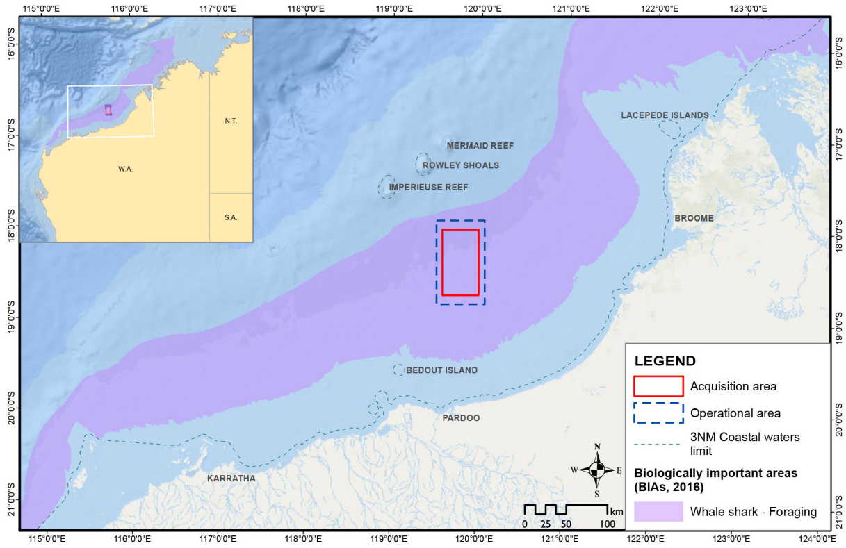
Figure 4-12 – Whale Shark BIAs
