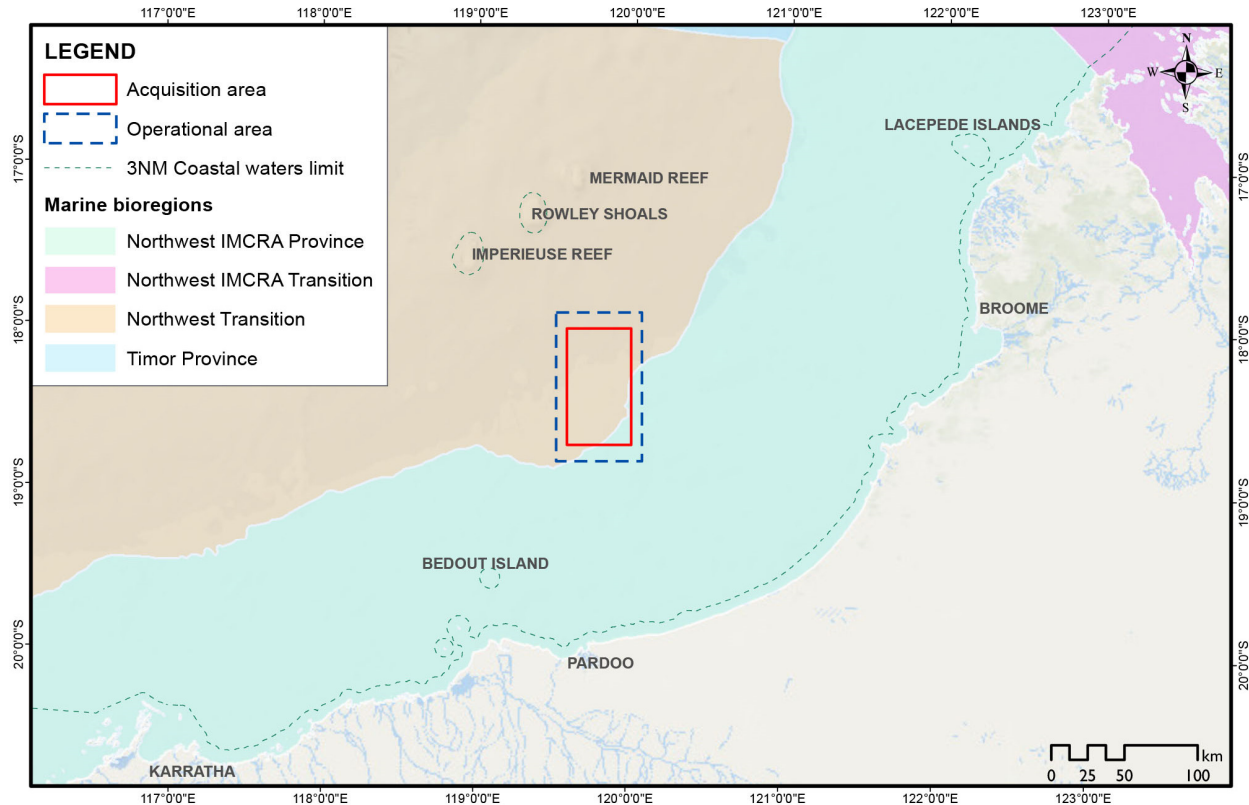
Figure 4-3 – Provincial Bioregions (IMCRA v4.0)
